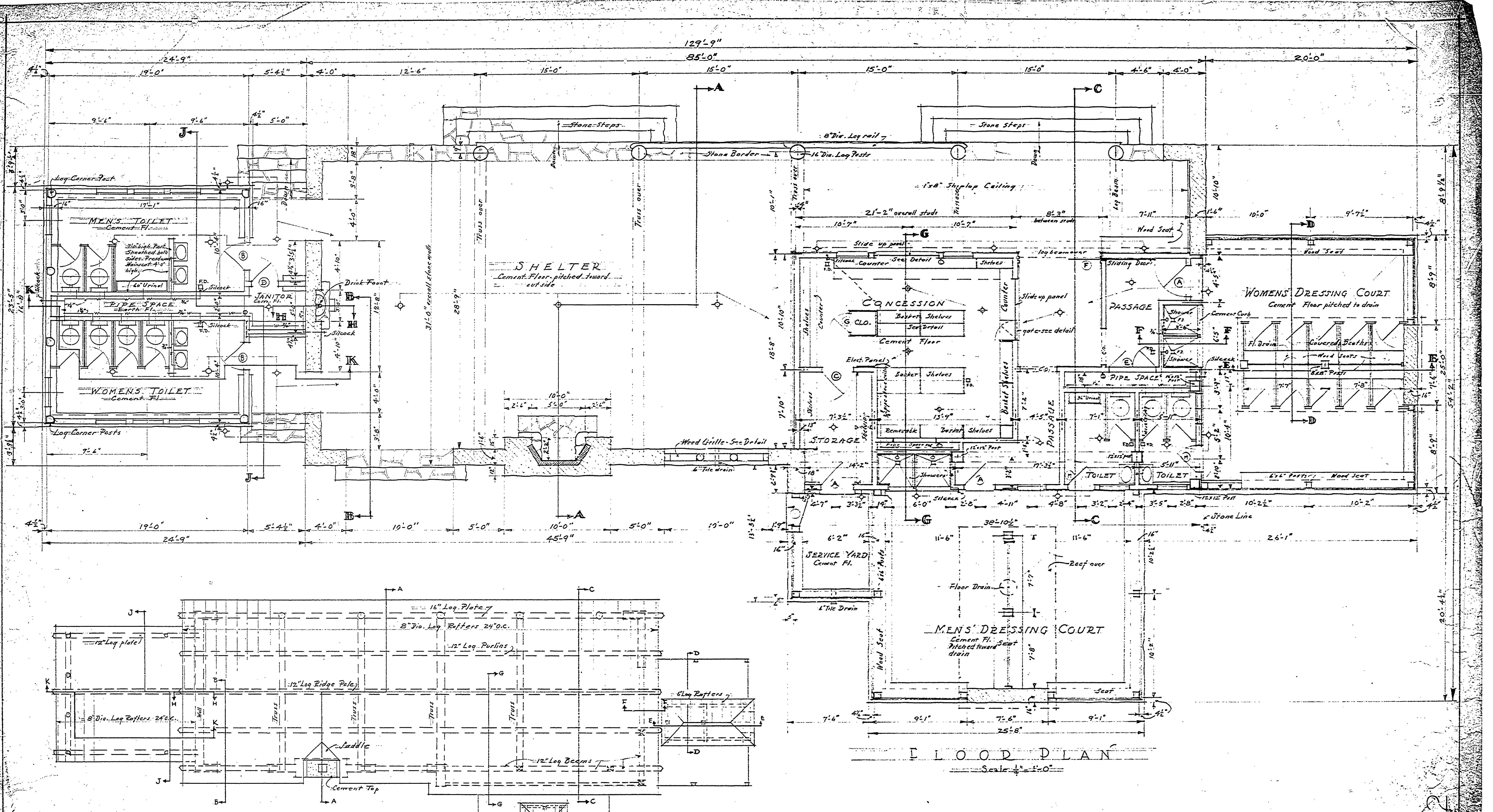
ROOF FRAMING PLAN Scale 1/8" = 1'-0"
