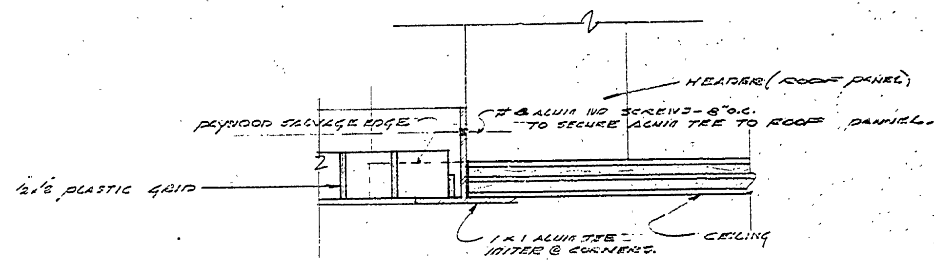
TYPICAL SECTION THRU PLASTIC GRID SUPPORT @ SKYLIGHTS.
