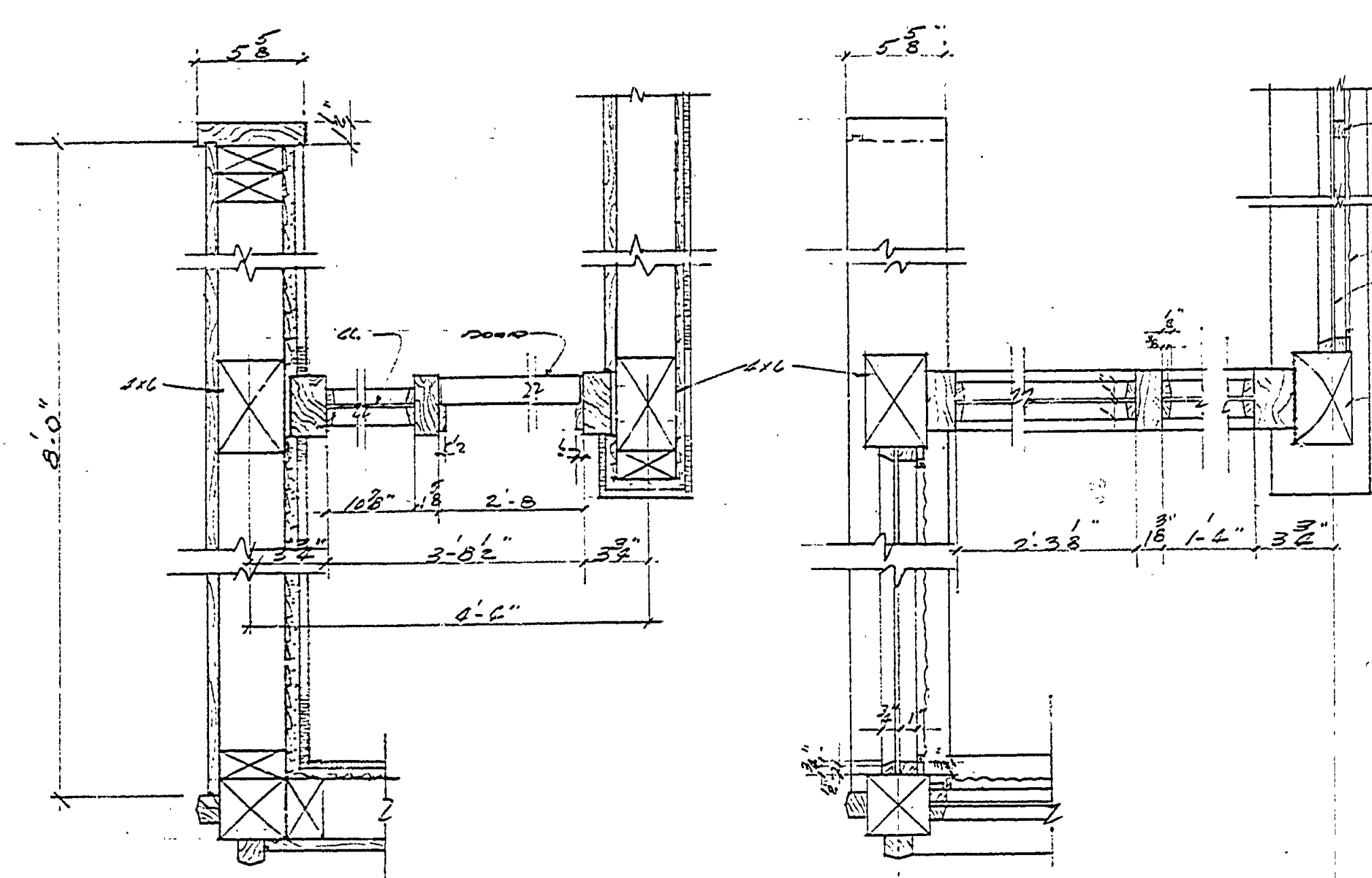
ENTRANCE DET. 9/55
