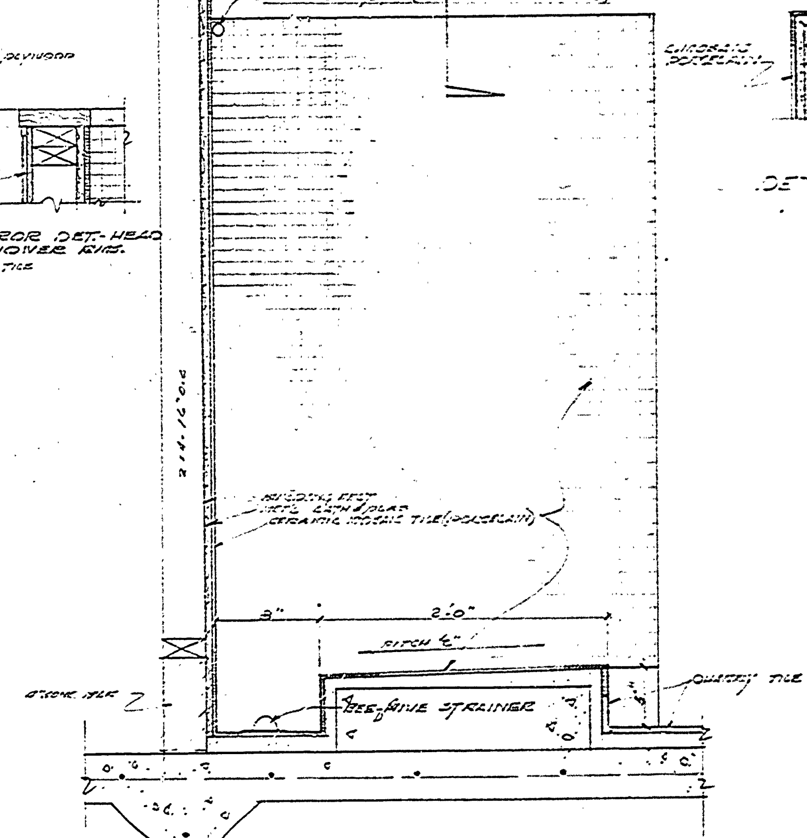
DETAIL URINAL 7/55
