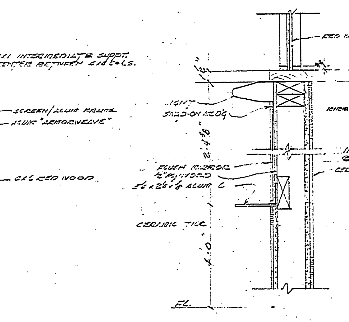
MIRROR & LIGHT DETAIL
