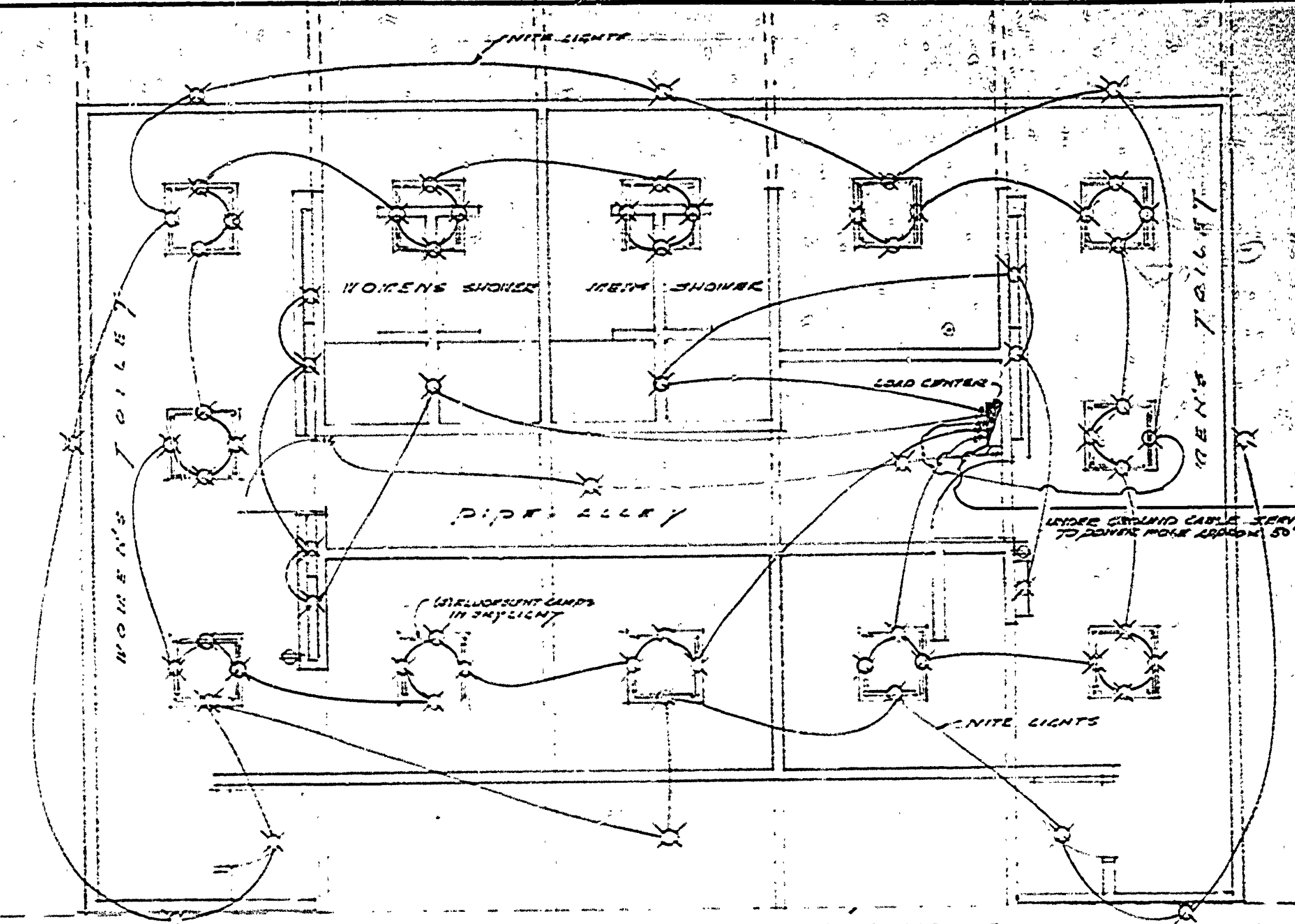
ELECTRICAL LIGHTING PLAN
