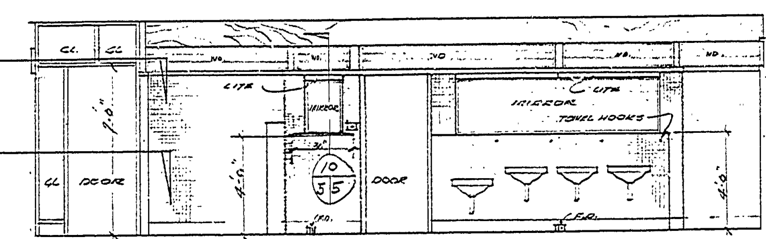
WEST INTERIOR ELEVATION - MEN'S TOILET
