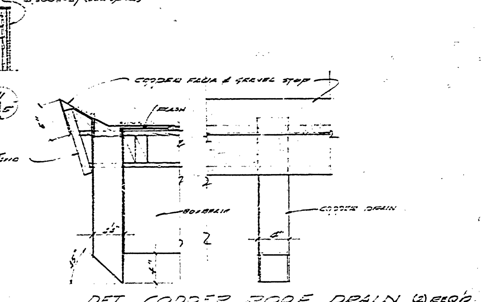
DET. COPPER ROOF DRAIN 10/55
