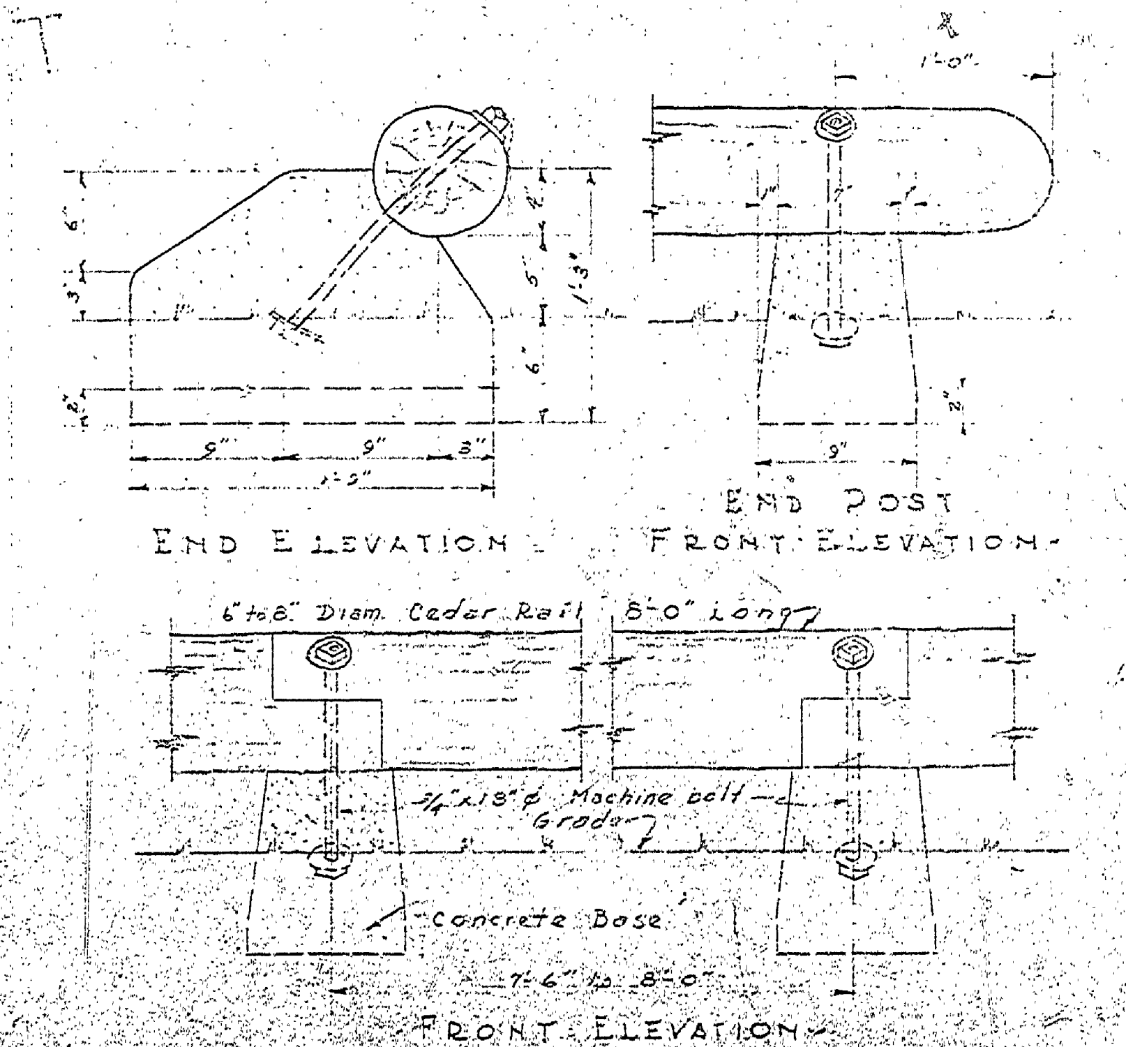
PARKING AREA LOG BARRIER DETAILS Scale 1/2" = 1'-0"
