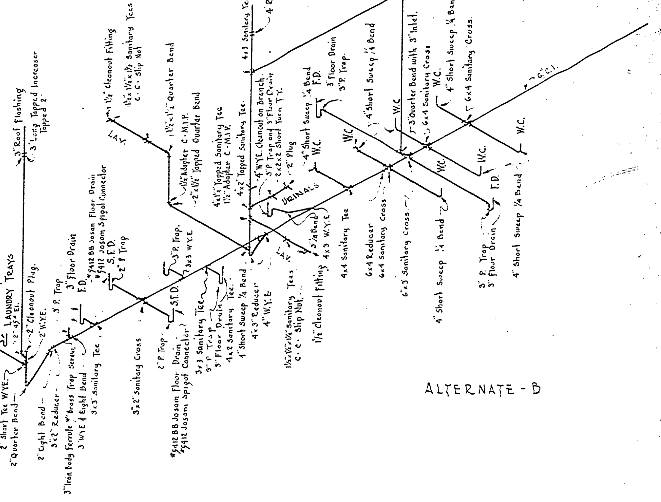
DRAINAGE PIPING DIAGRAM No Scale.
