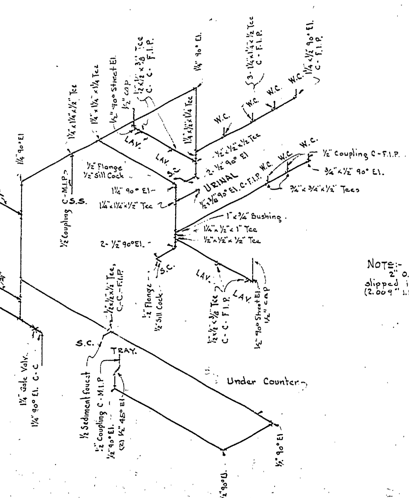
COLD WATER PIPE LAYOUT No Scale.
