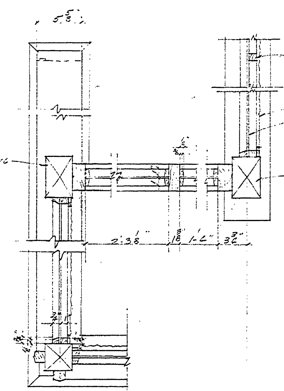
ENTRANCE DET. SCALE 1/4" = 1'-0"
