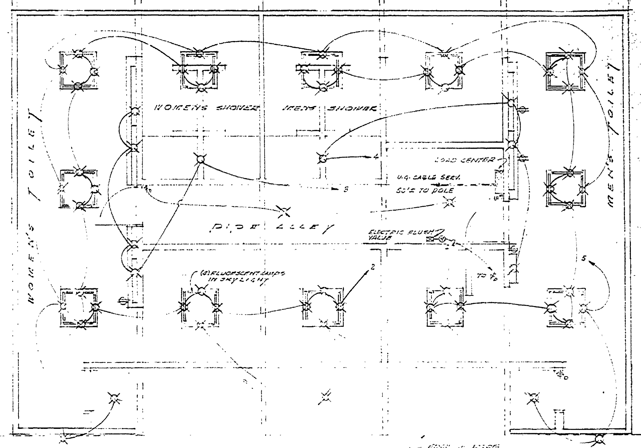
ELECTRICAL LIGHTING PLAN
