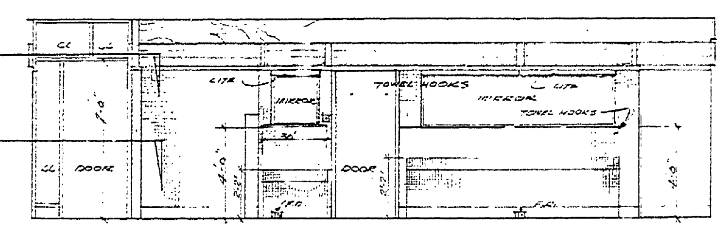
EAST INTERIOR ELEVATION - MEN'S TOILET
