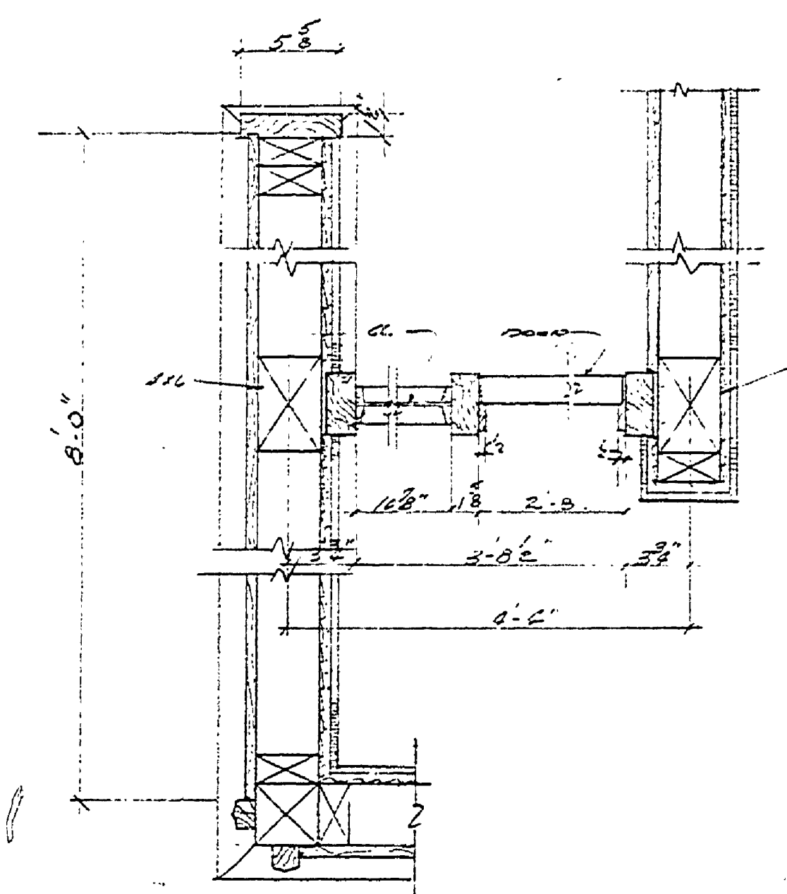
ENTRANCE DET. SCALE 1/4" = 1'-0"
