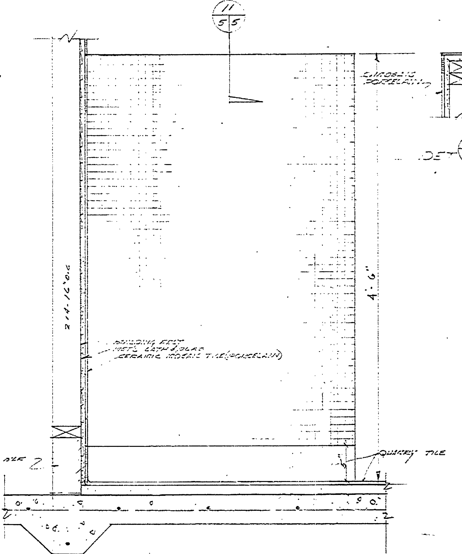
DETAIL URINAL
