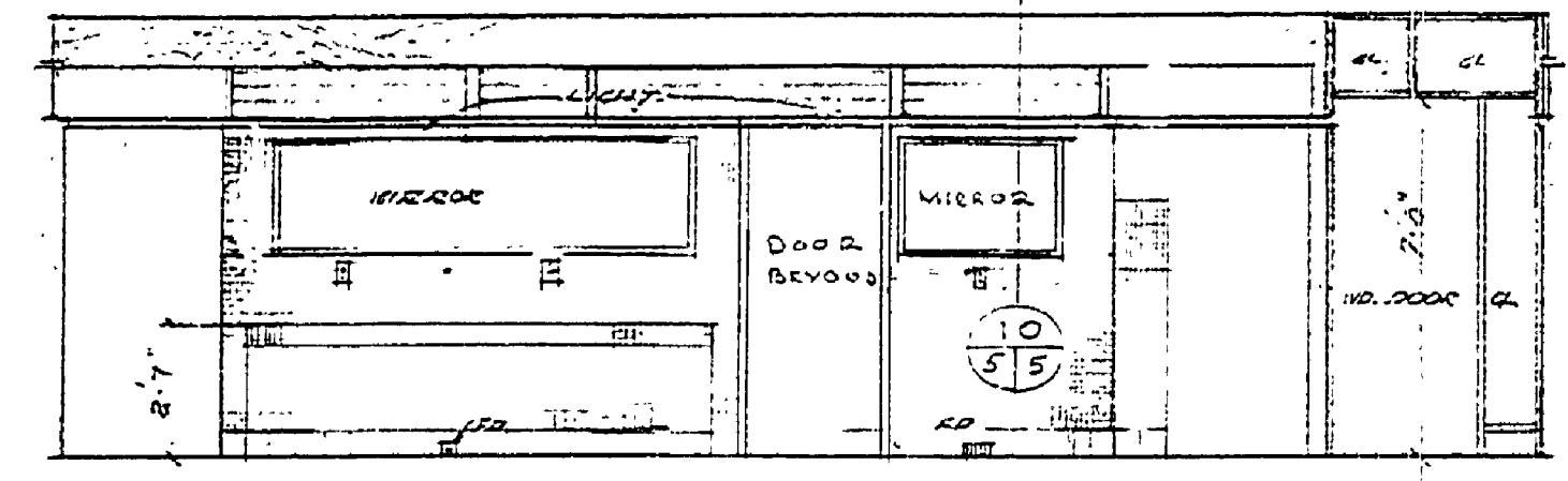
INTERIOR ELEV. - MEN'S TOILET
