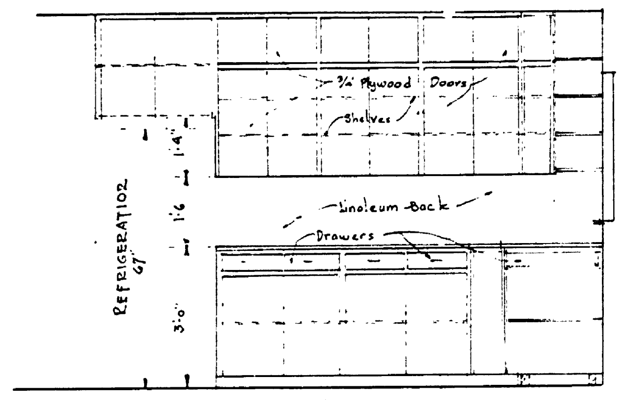
ELEVATIONS OF KITCHEN No. 11 Scale 1/2" = 1'-0"
