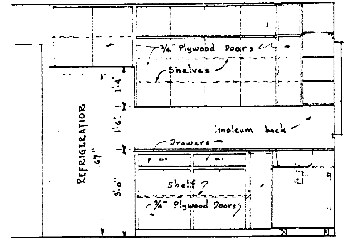
ELEVATIONS OF KITCHEN No. 7 Scale 1/2" = 1'-0"
