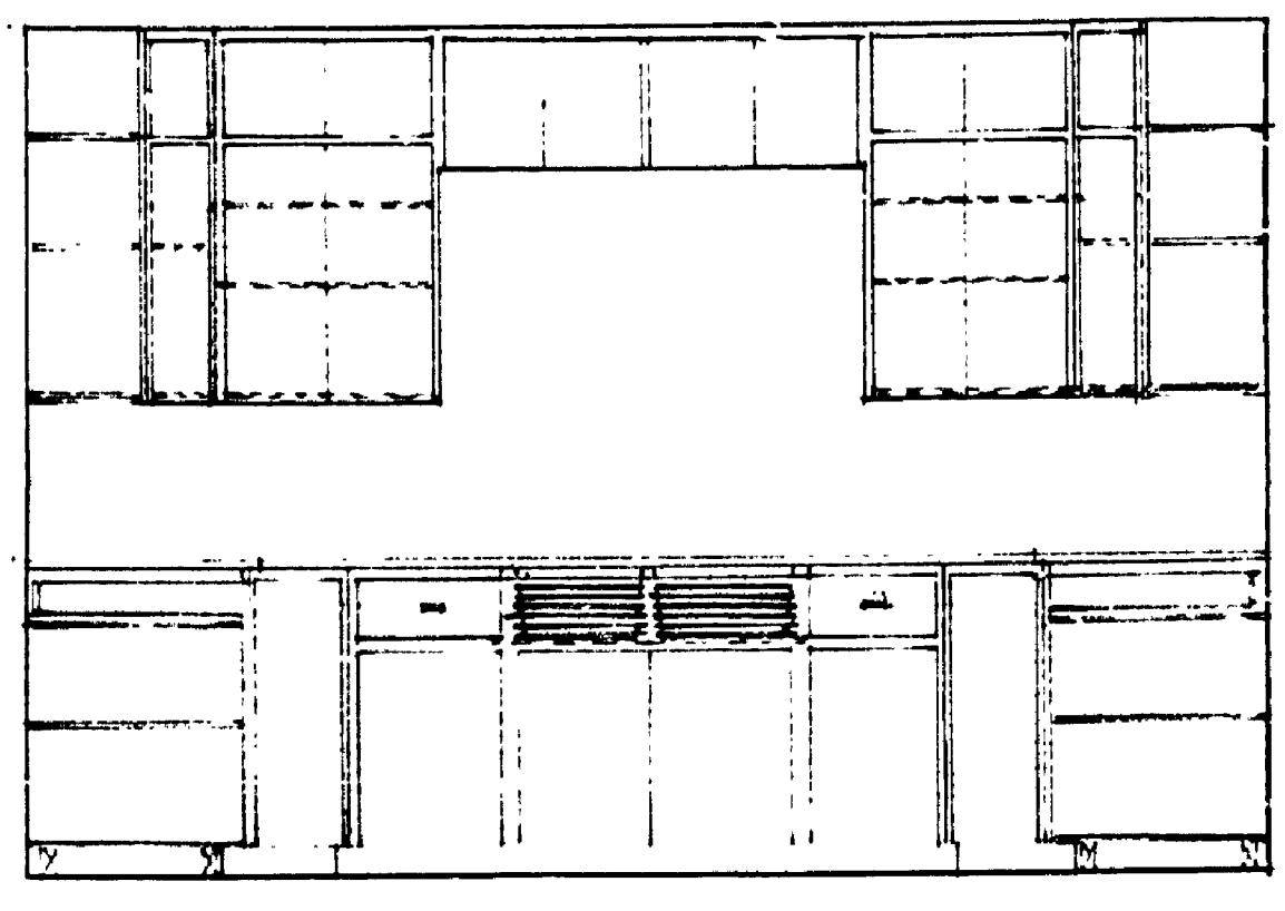
ELEVATIONS OF KITCHEN No. 11 Scale 1/2" = 1'-0"
