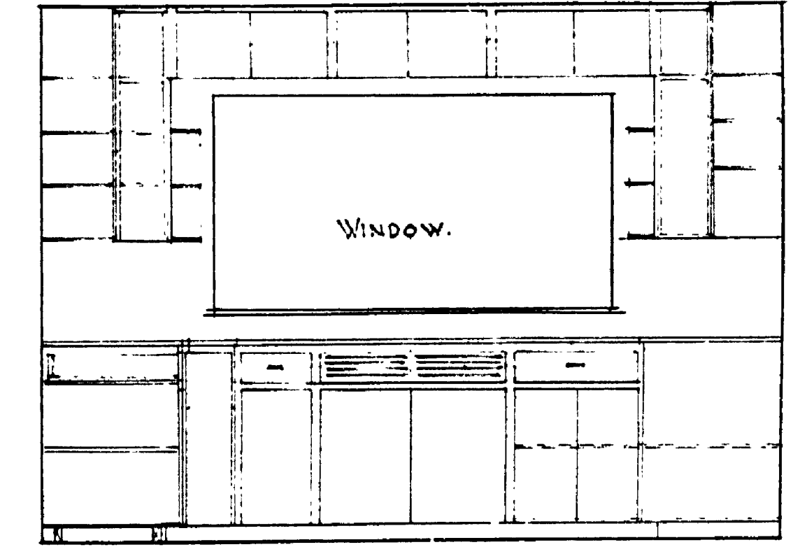
ELEVATIONS OF KITCHEN No. 8 Scale 1/2" = 1'-0"
