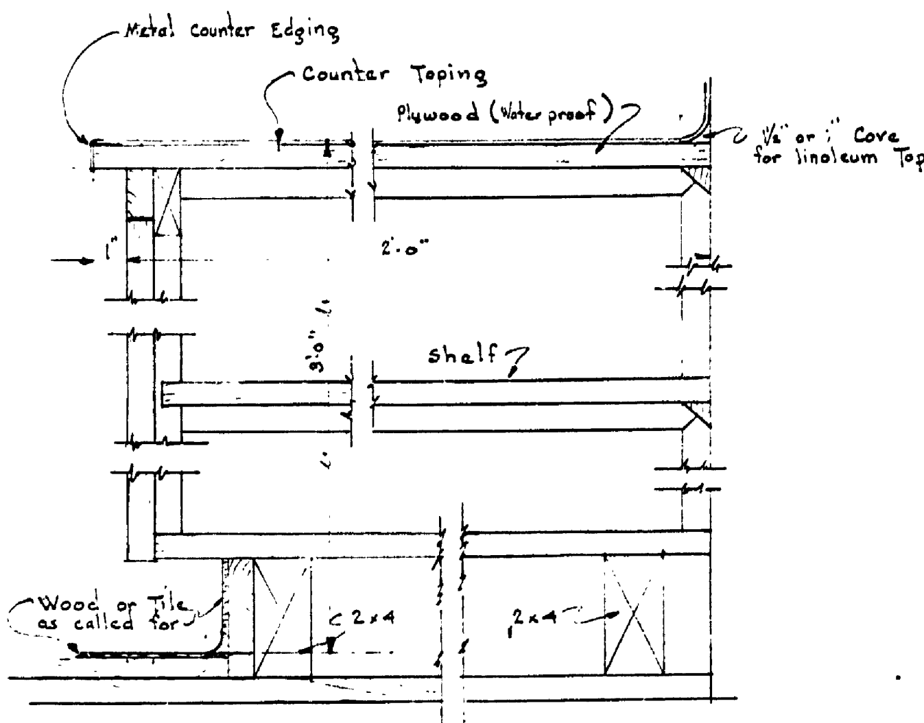
TYPICAL SECTION THRU COUNTER Scale 1/2" = 1'-0"
