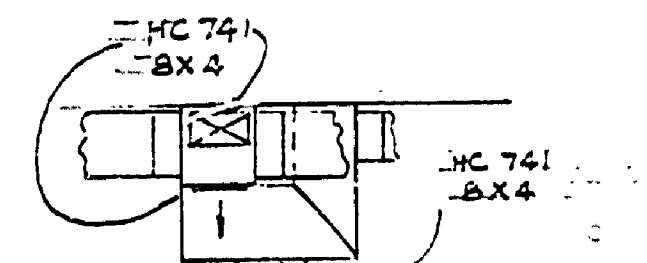
END VIEW OF TRUNK DUCT SHOWING DIFFUSERS SECTION B-B
