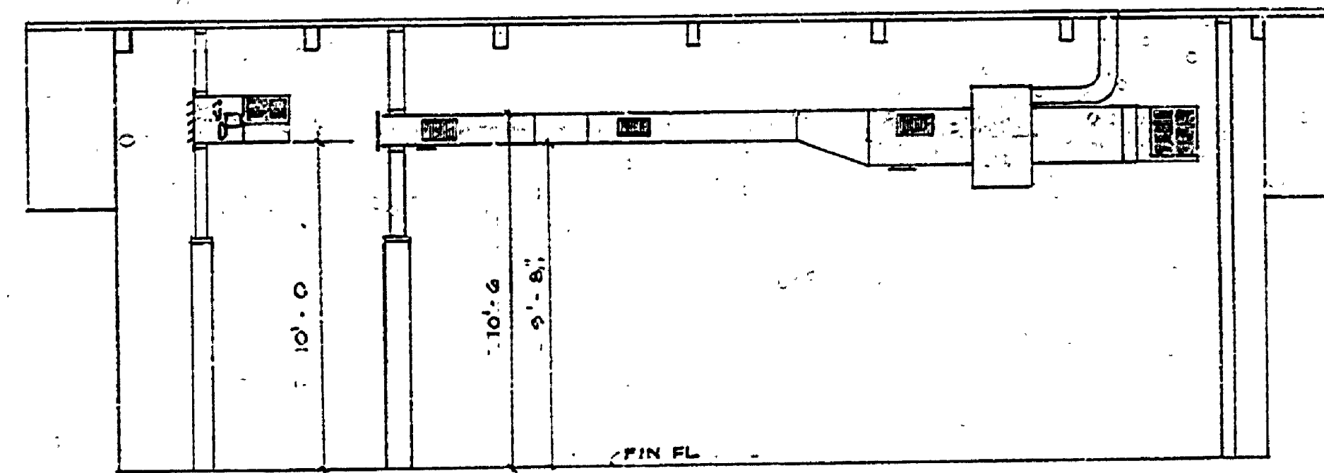
HALF SECTION SHOWING DUCTWORK IN PIPE ALLEY, 1/4\"/>
