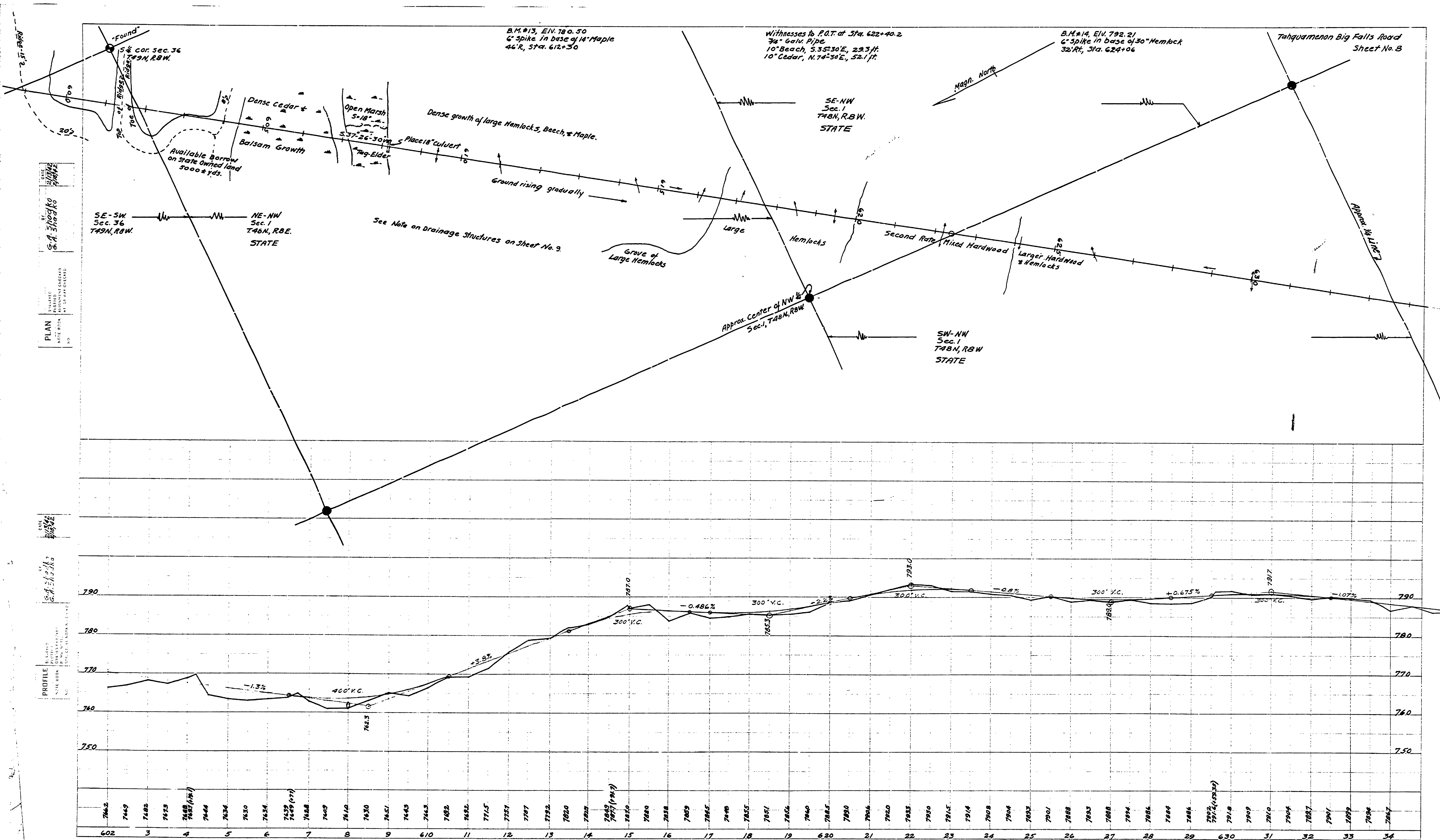
PLATE 1 PLAN AND PROFILE OF ROAD DIAMOND THE PLAN, PROFILE, AND DRAINAGE ARE SHOWN IN THIS PLATE. SCALE: 1" = 40' HORIZ. 1" = 10' VERT.
