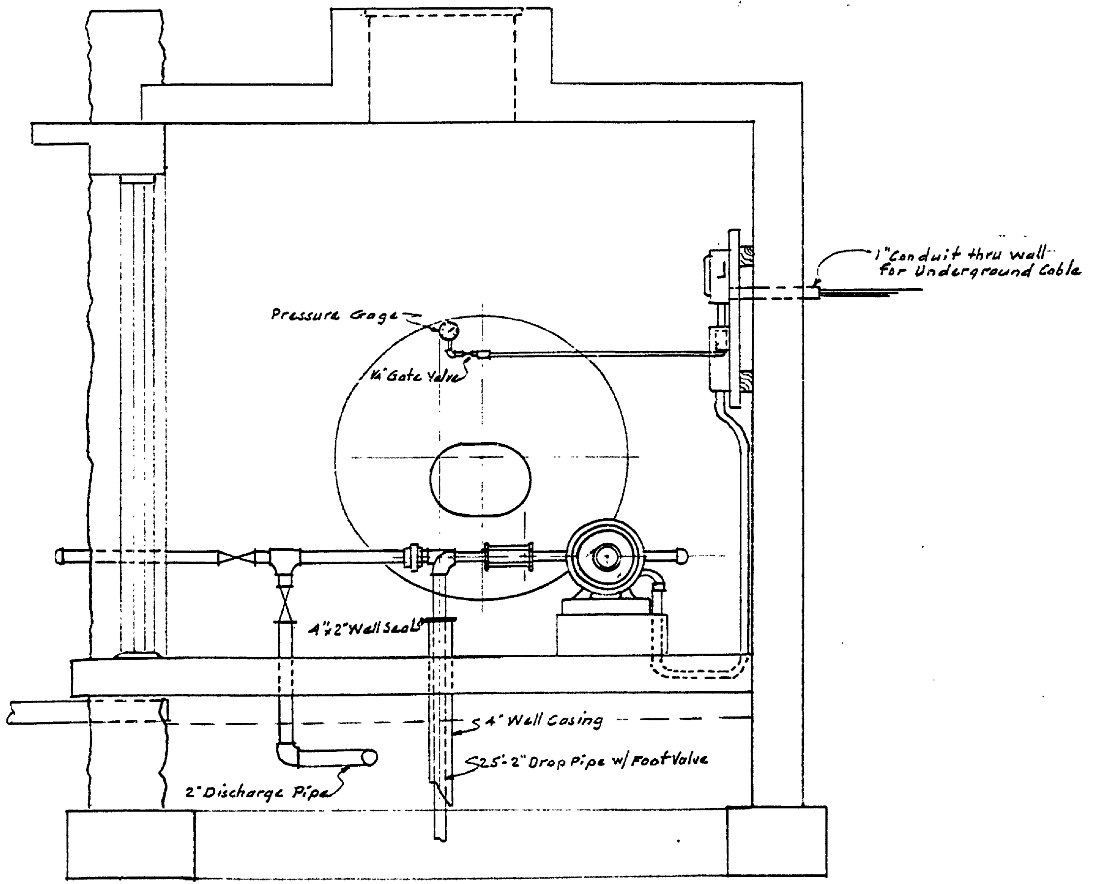
SECTION A-A SCALE 3/4"=1'-0"
