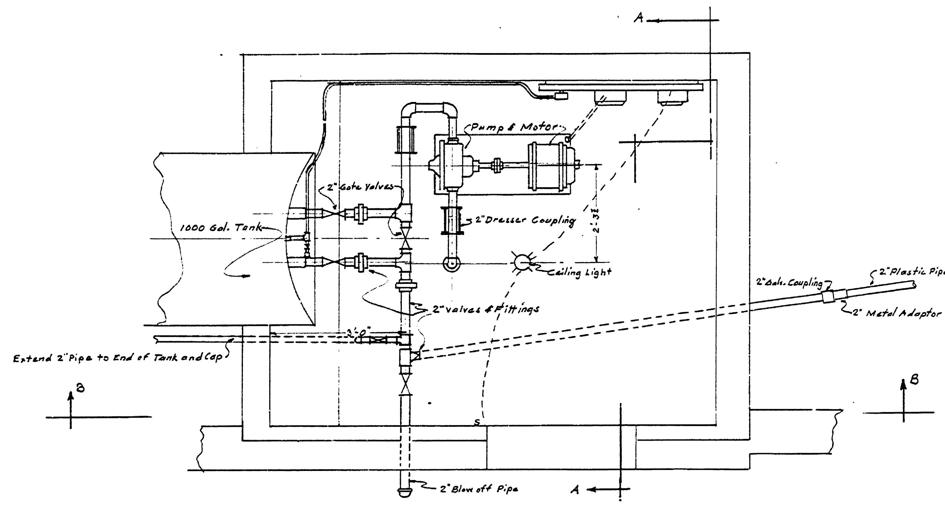
PLAN OF MECHANICAL LAYOUT SCALE 3/4"=1'-0"
