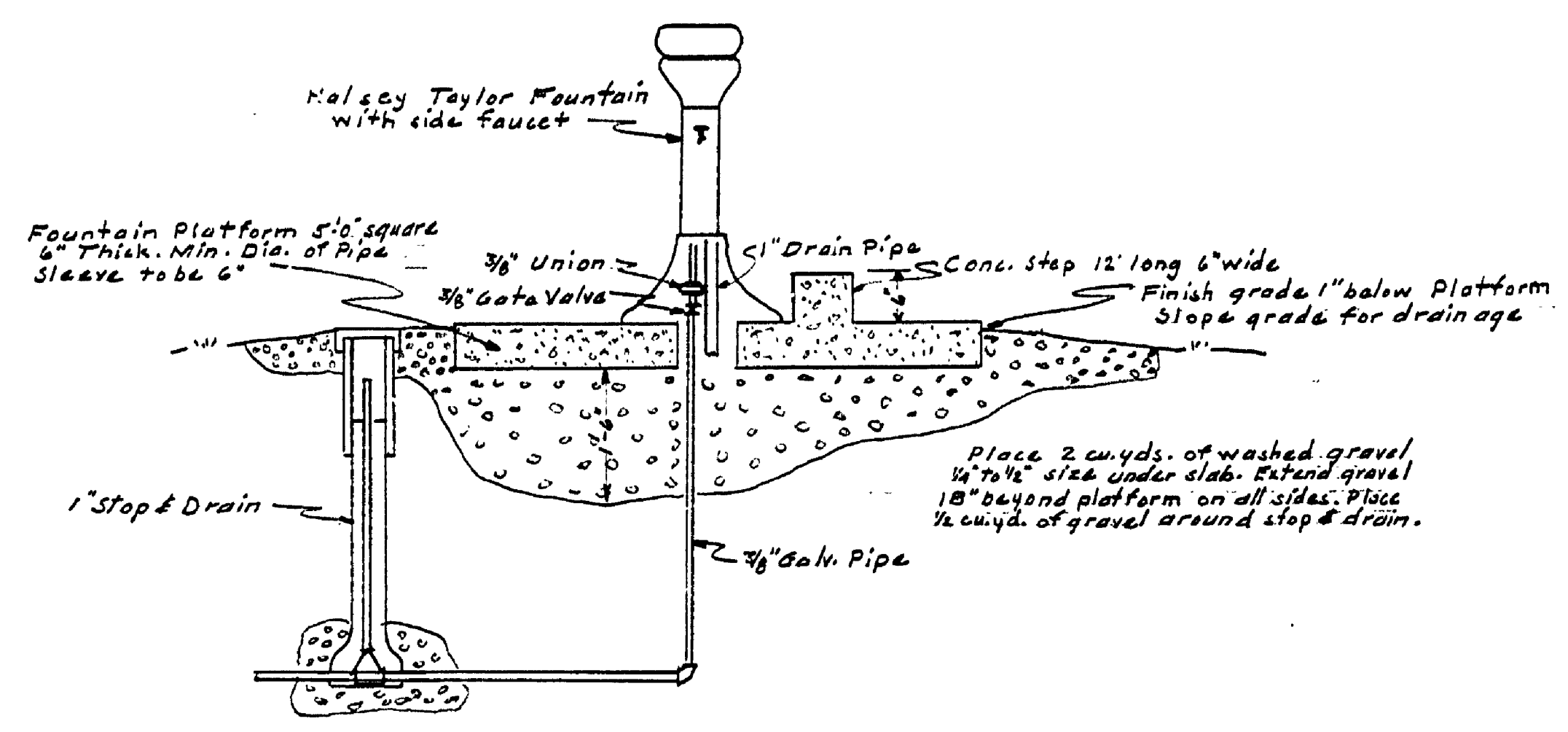
DRINKING FOUNTAIN Not to scale
