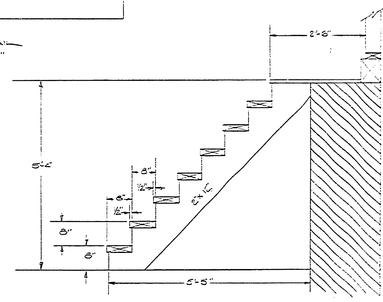
BASEMENT STAIR DETAIL SCALE 3/4" = 1'-0"
