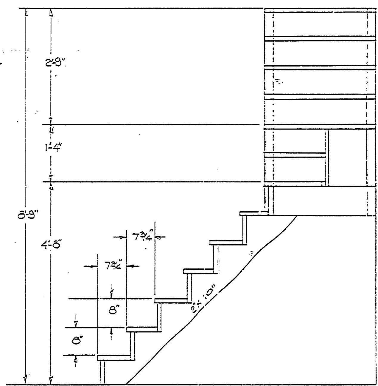
MAIN STAIR DETAIL SCALE 3/4" = 1'-0"
