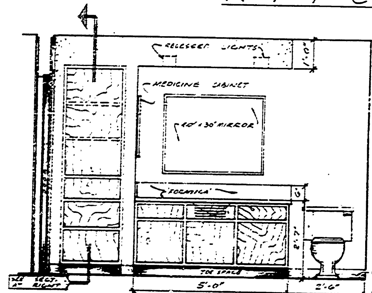
ELEVATION - BATHROOM SCALE = 1/2" = 1'-0"
