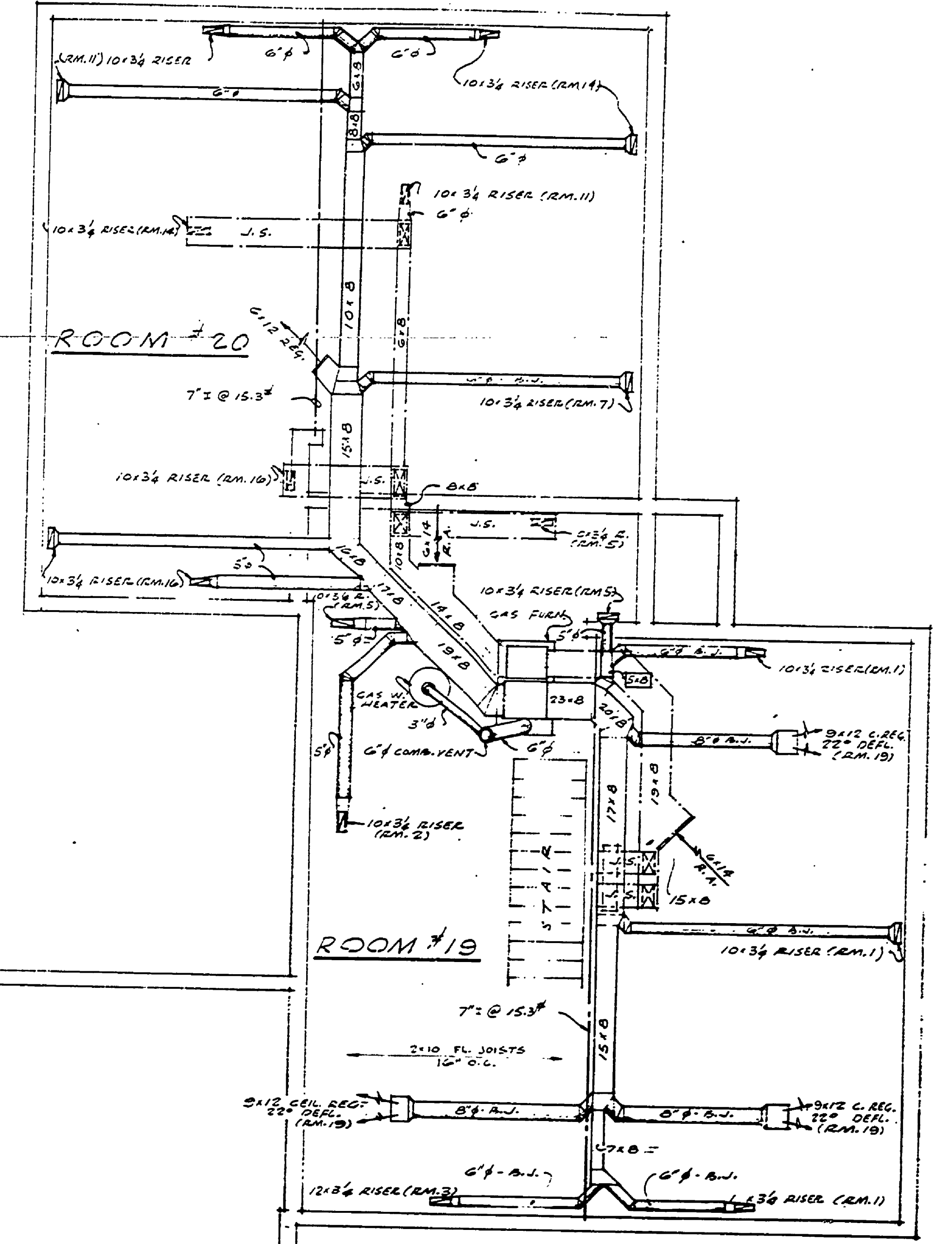
HEATING PLAN - BASEMENT SCALE = 1/8" = 1'-0"
