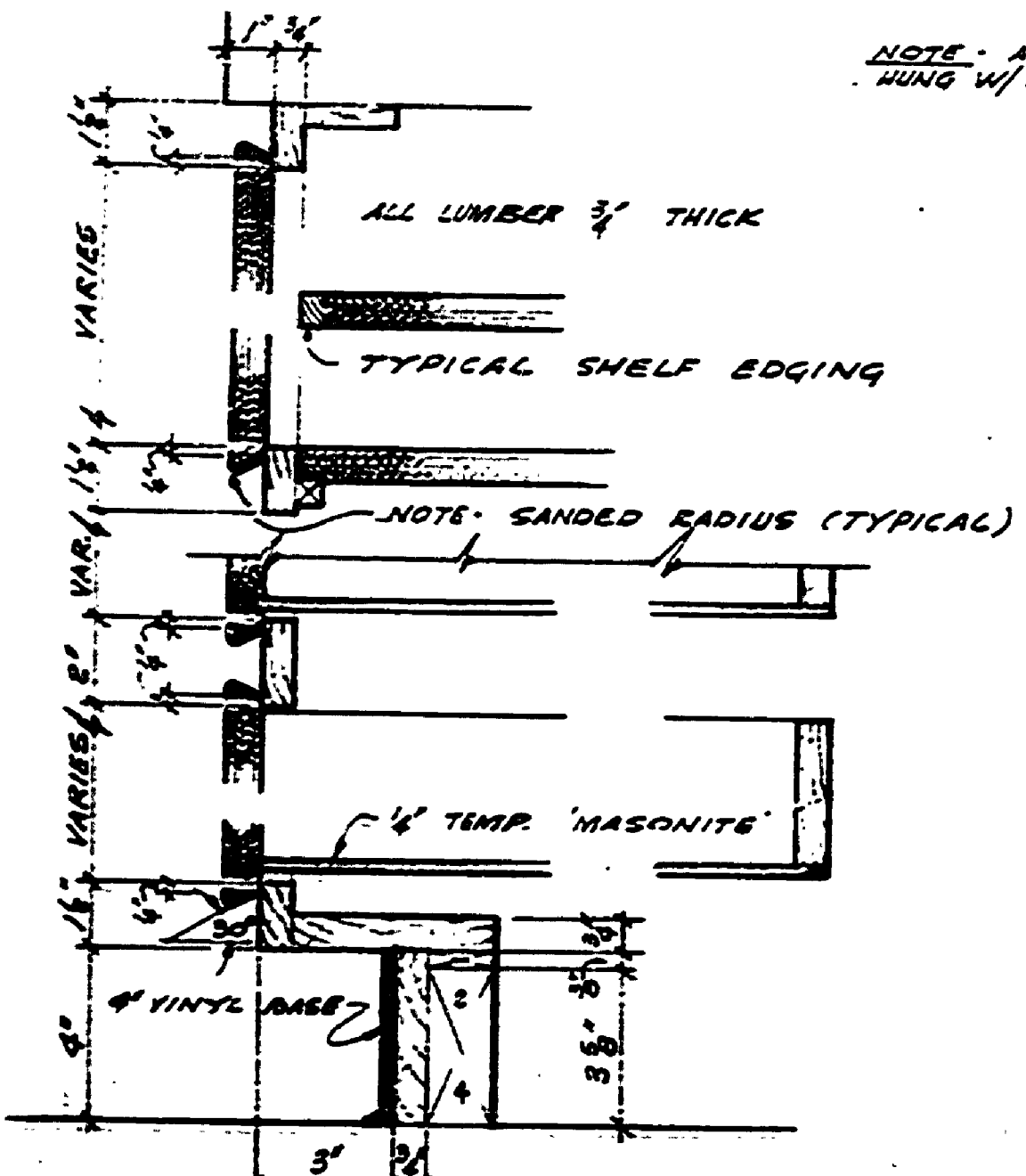
CABINET DETAILS SCALE = 5/8" = 1'-0"
