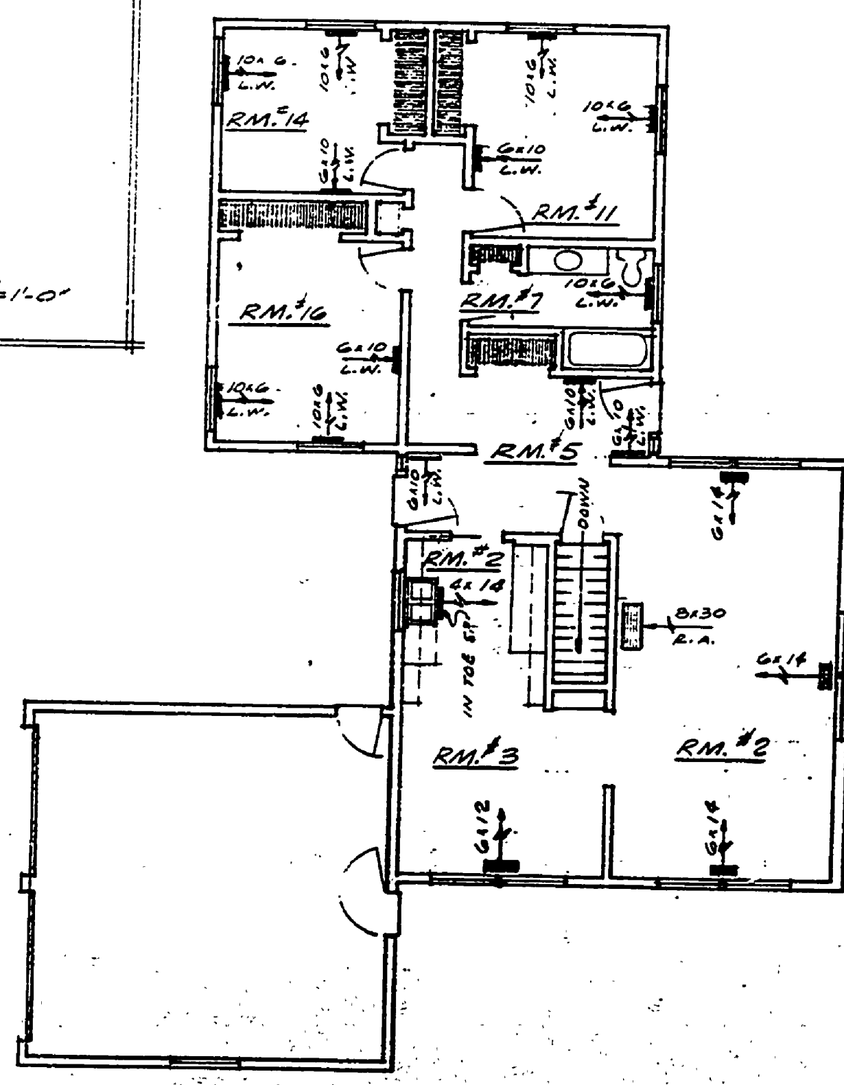
HEATING - FIRST FL. PLAN SCALE = 1/8" = 1'-0"
