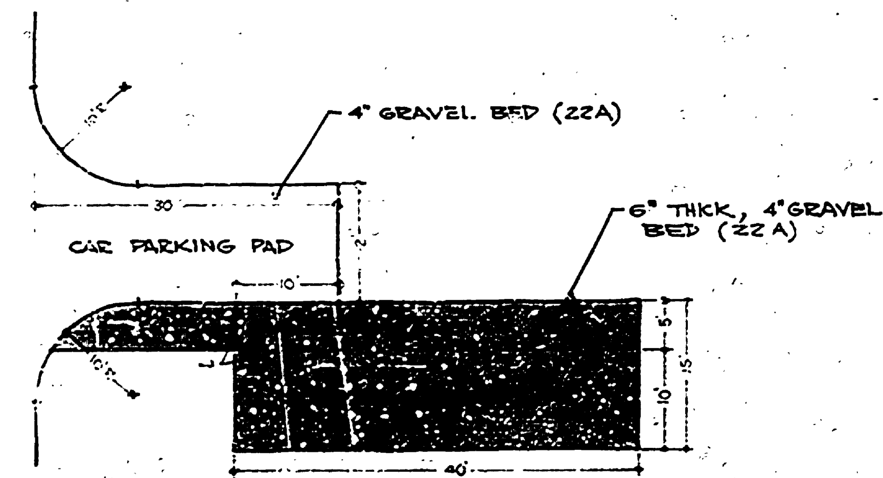
CAR & TRAILER PAD DETAIL - A SCALE: 1" = 10'
