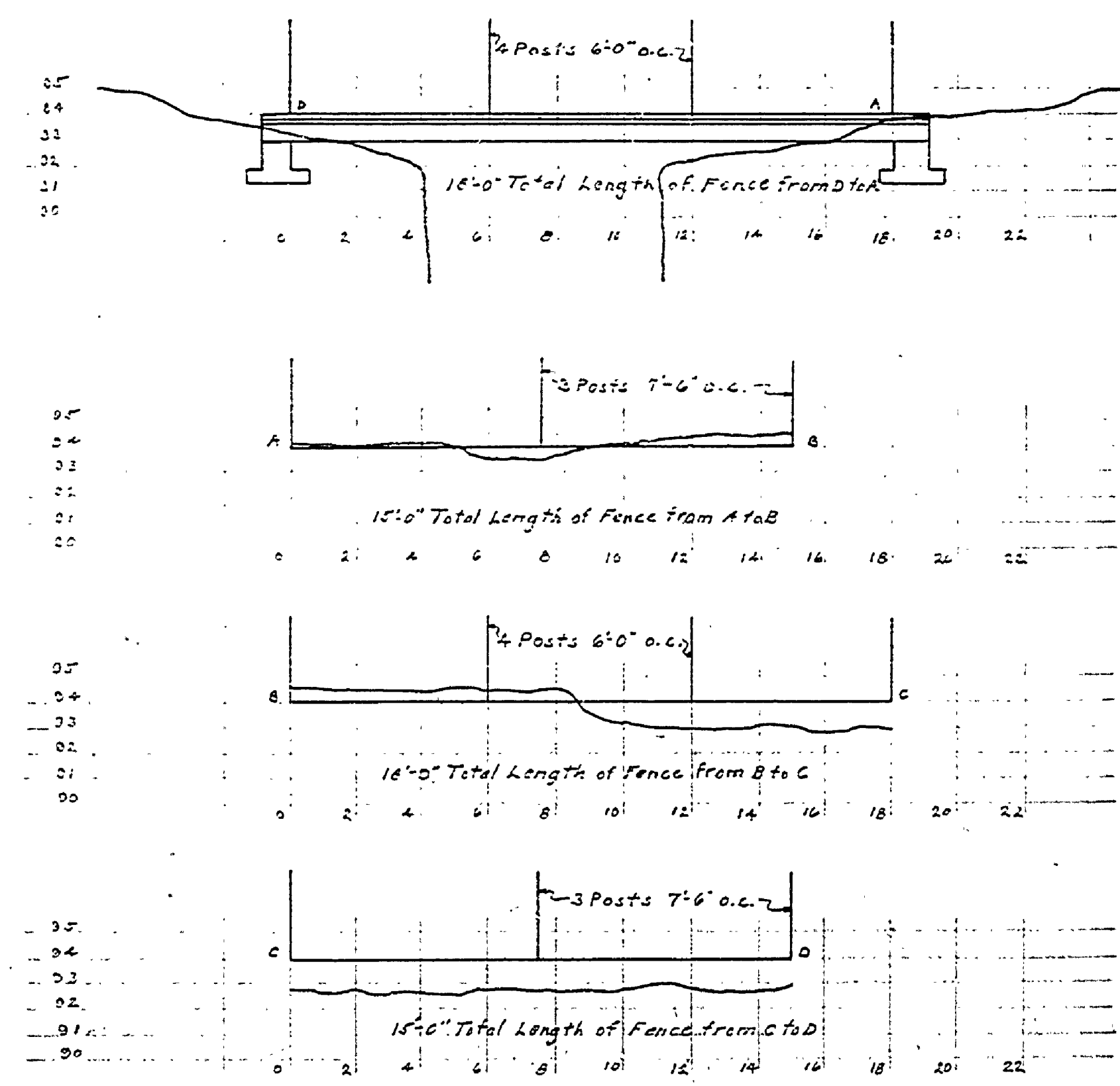
PROFILE OF FENCE LINE FOR MINE SHAFT NO. 1
