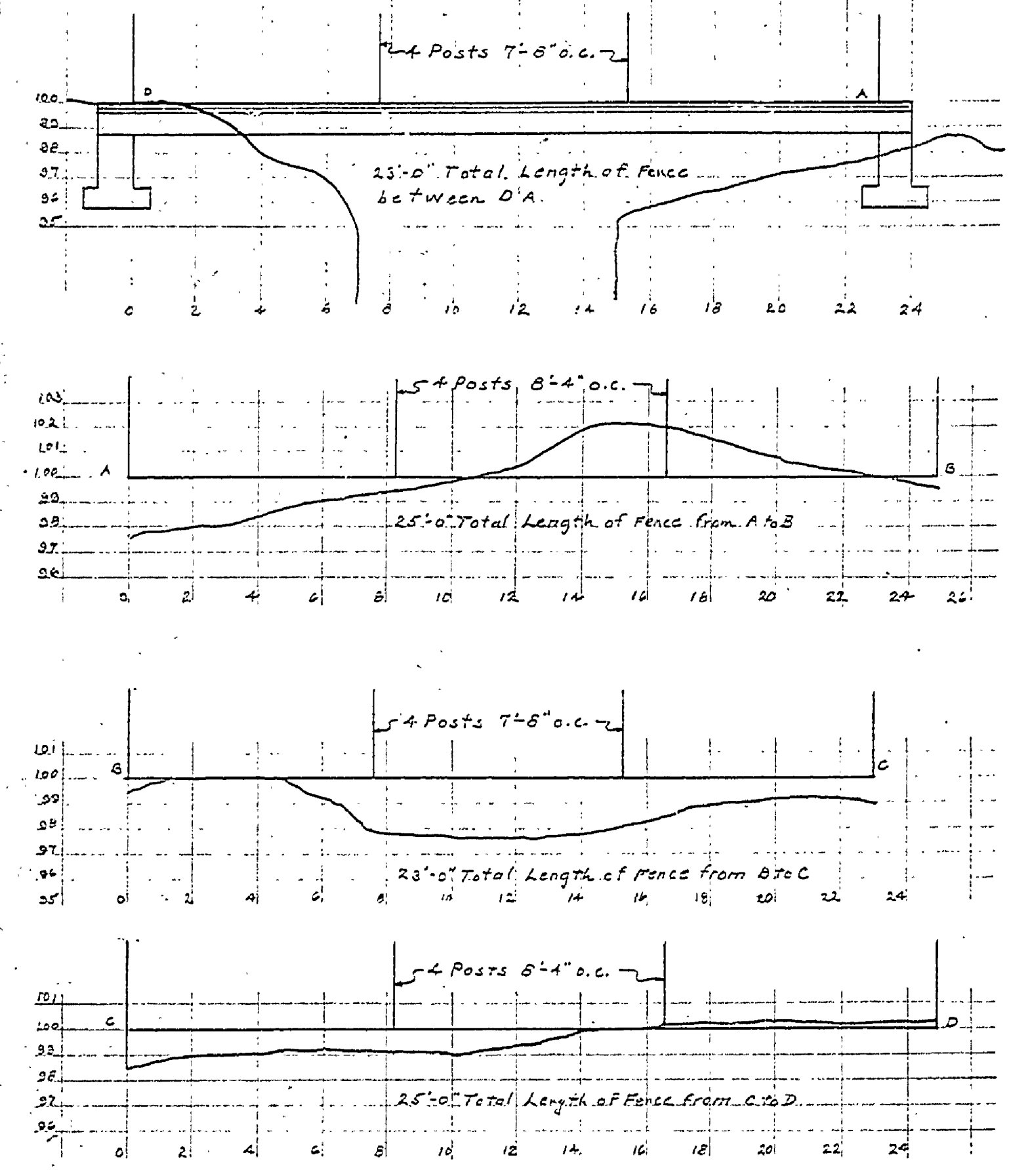
PROFILE OF FENCE LINE FOR MINE SHAFT NO. 3
