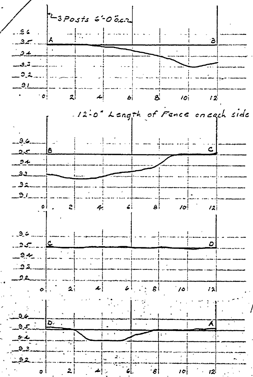
PROFILE OF FENCE LINE FOR MINE SHAFT NO. 2
