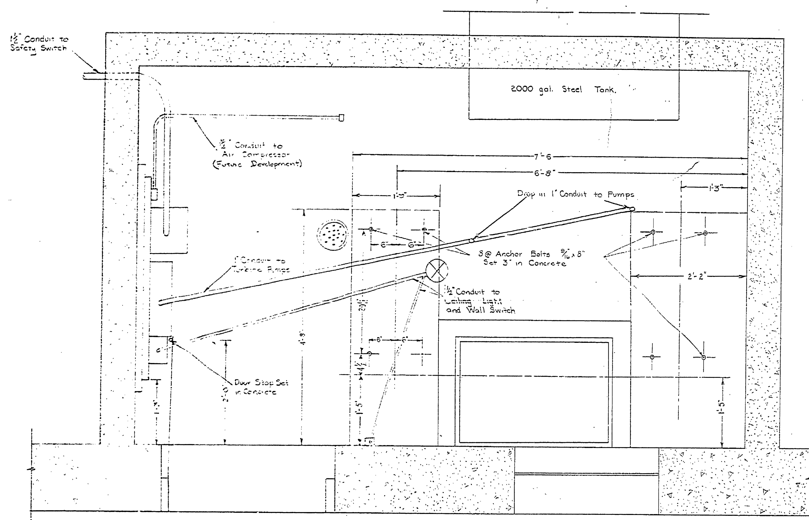
PLAN FOR MOUNTING TURBINE PUMPS Scale 1"=1'-0"
