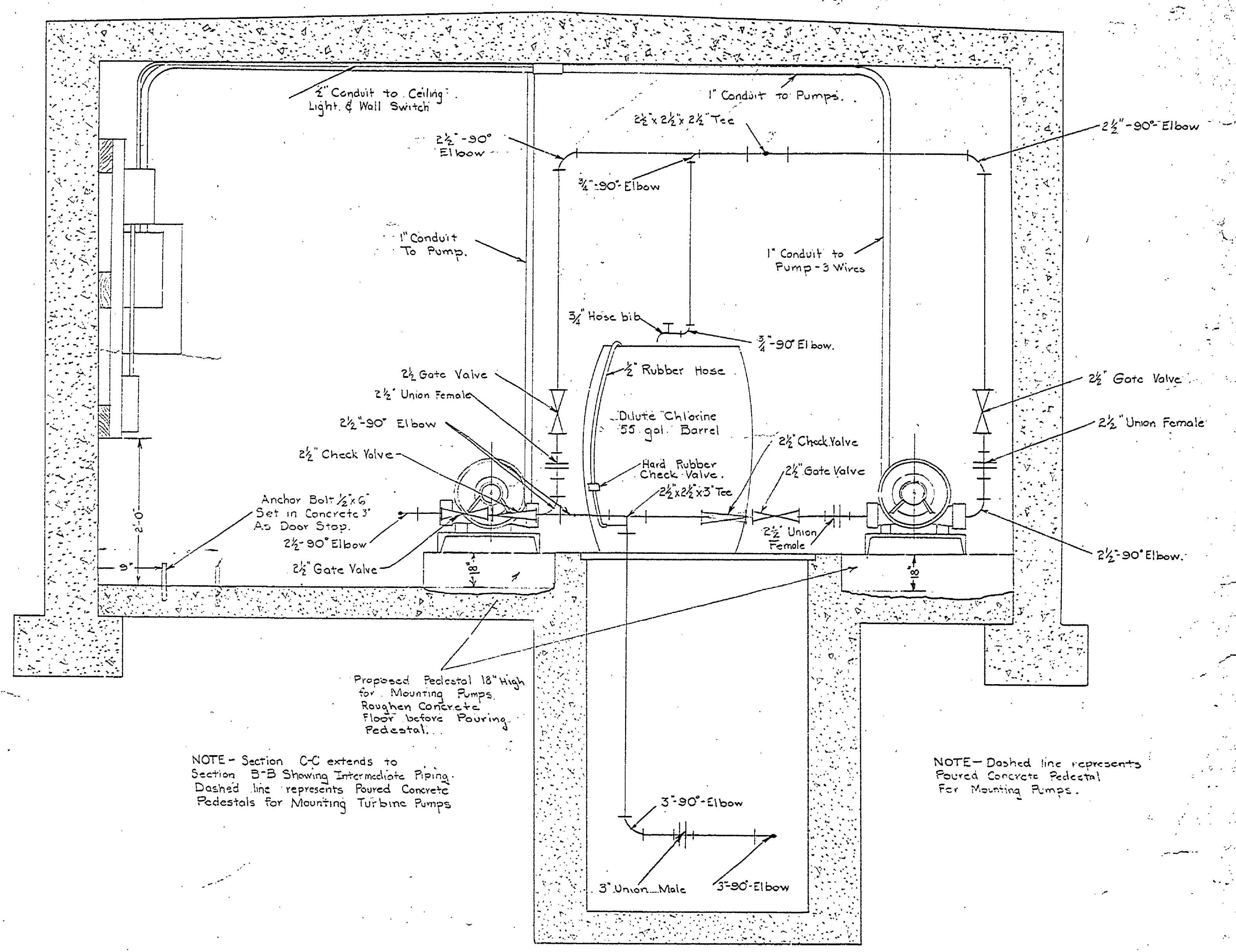
SECTION C-C Scale 1"=1'-0"
