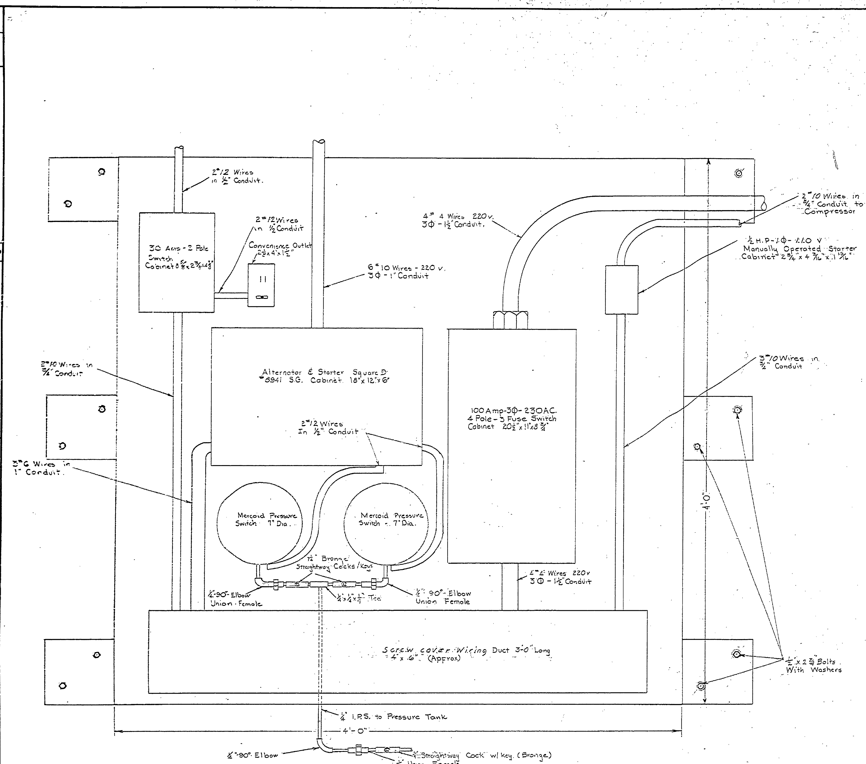
LAY-OUT FOR CONTROL PANEL Scale 3" = 1'-0"
