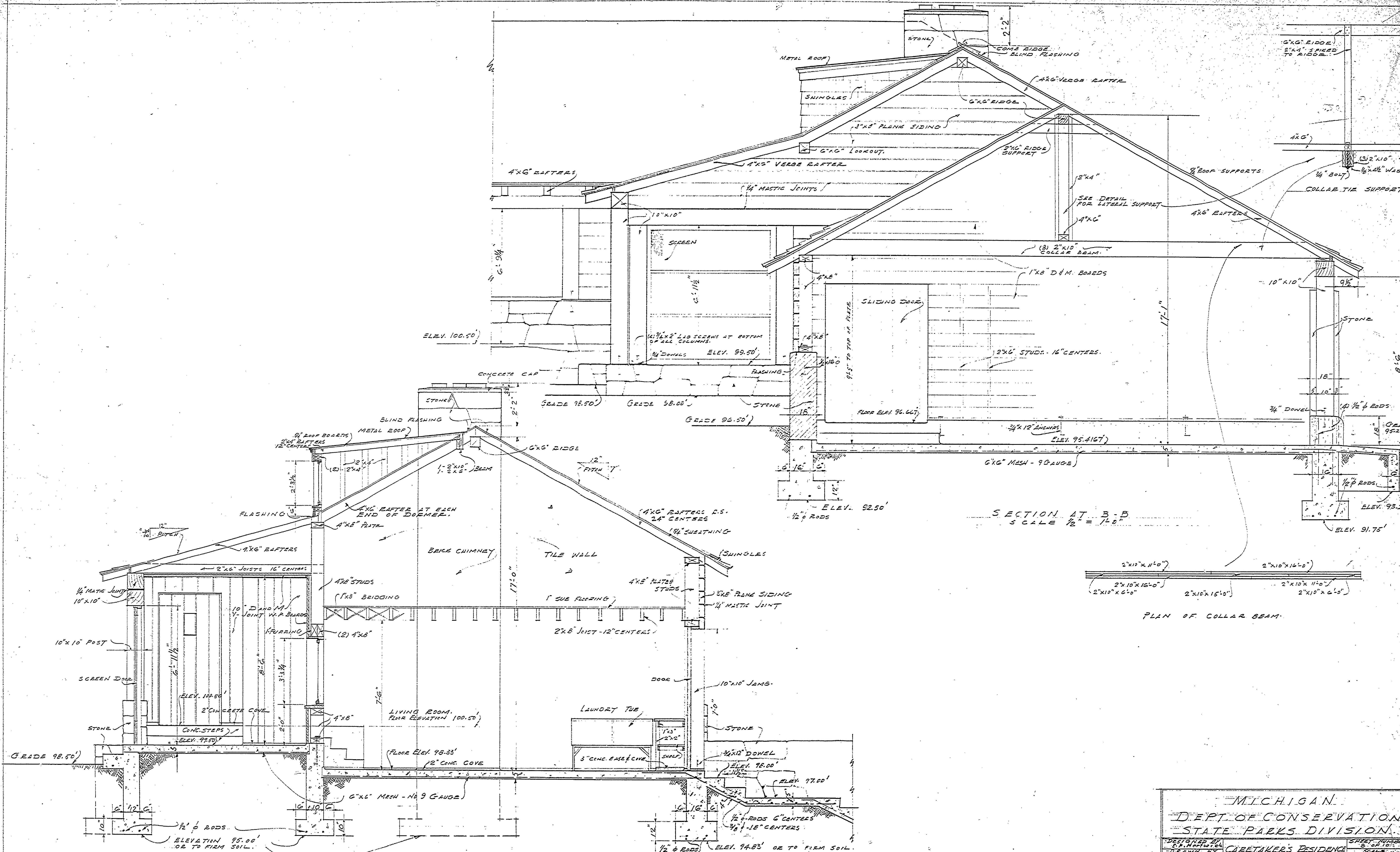
SECTION AT C-C SCALE 1/2" = 1'-0"
