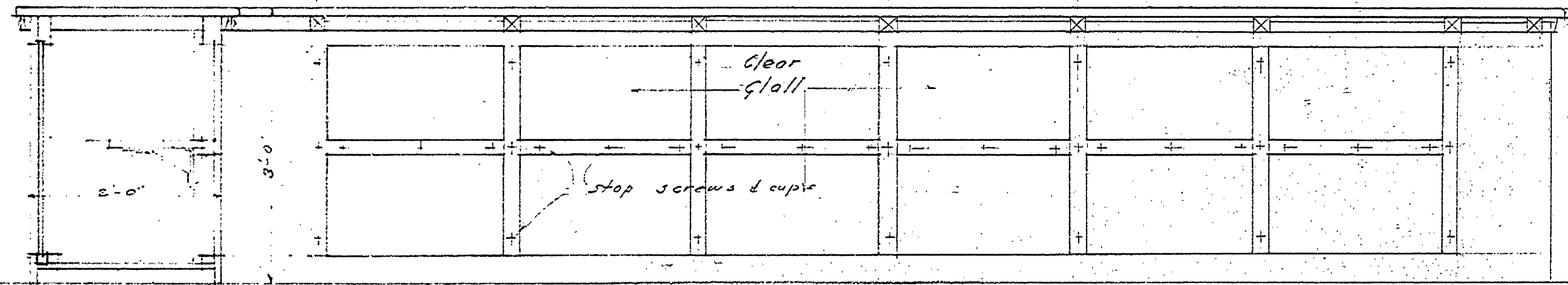
ELEVATION SCALE 1/2"=1'-0"
