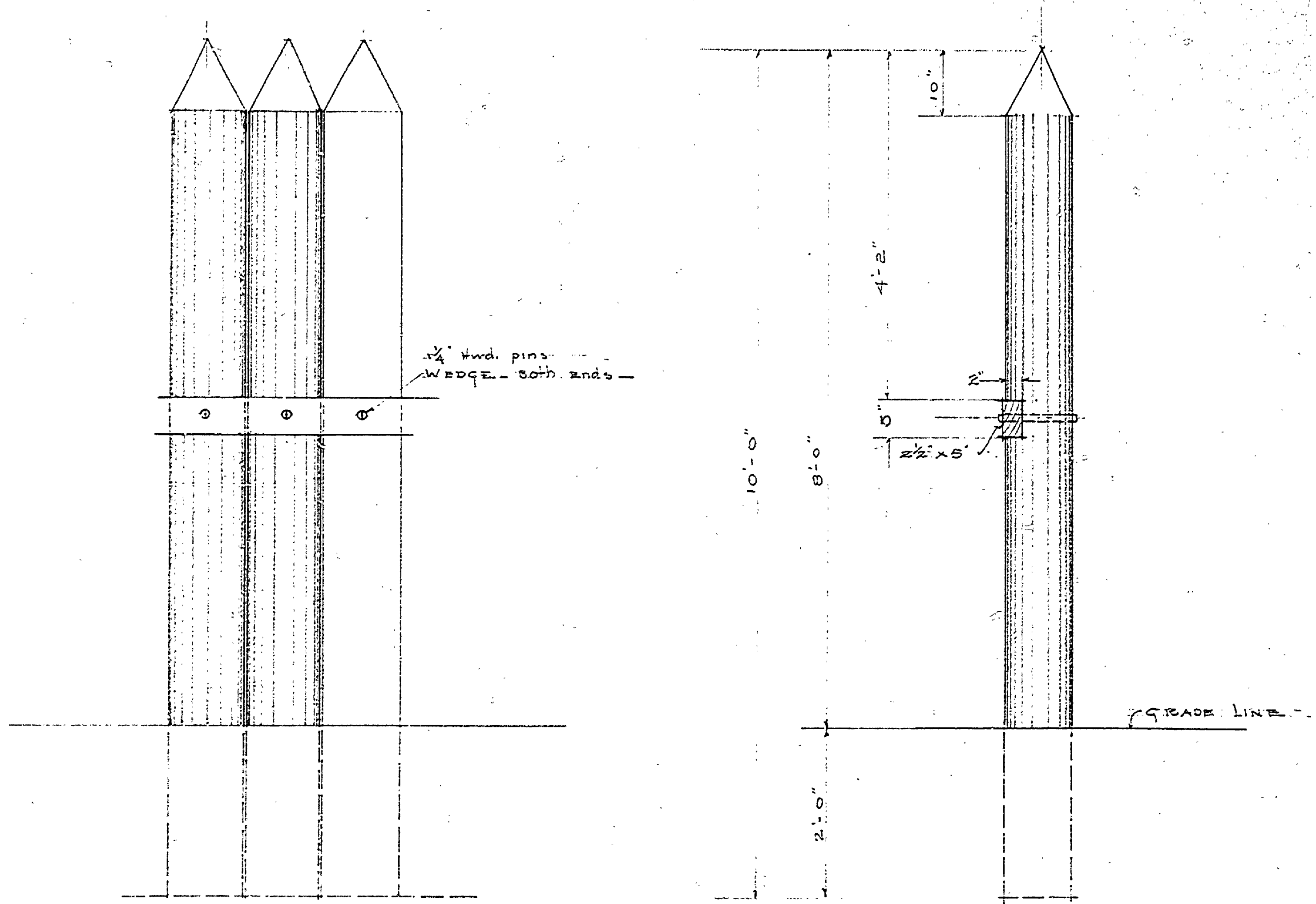
SIZE OF POSTS MIN. 7" AT TOP MAX. 10" DETAIL OF STOCKADE scale 1"=1'-0"
