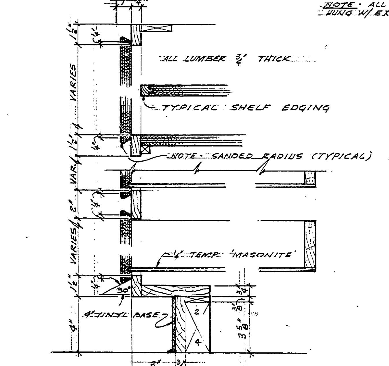
CABINET DETAILS SCALE - 3/8" = 1'-0"
