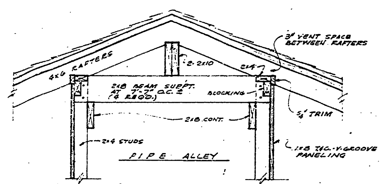
SECTION - TYPICAL INTERMEDIATE RIDGE BEAM SUPPORT & VENT INTO PIPE ALLEY 1/2" = 1'-0"
