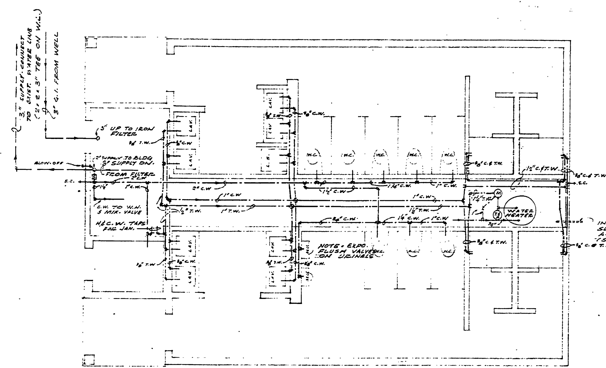
PLUMBING FL. PLAN (WATER)
