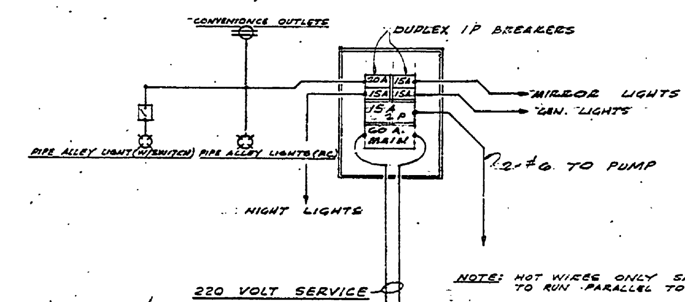
SCHEMATIC WIRING DIAGRAM ELECTRIC SERVICE PANEL & AUTOMATIC LIGHT CONTROL
