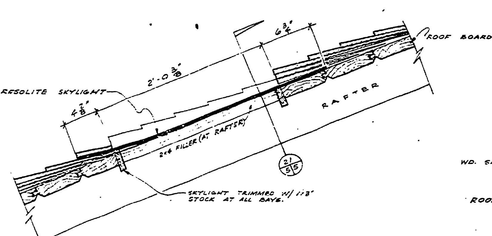
TYPICAL SKYLIGHT DET. 1/2" = 1'-0"
