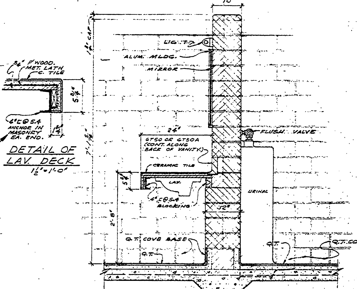
SECTION 3/8" = 1'-0"
