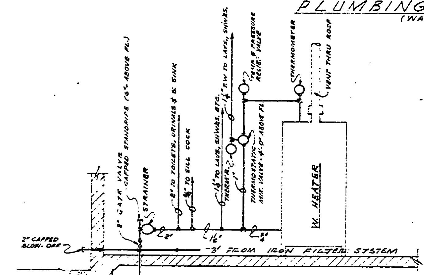
PLUMBING FL. PLAN (WATER)
