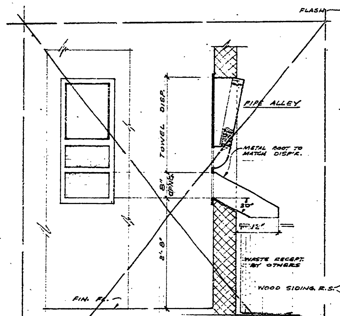
ELEVATION SECTION RECESSED TOWEL DISPENSER & WASTE DISPOSAL CHUTE 3/8" = 1'-0" DELETE THIS DETAIL
