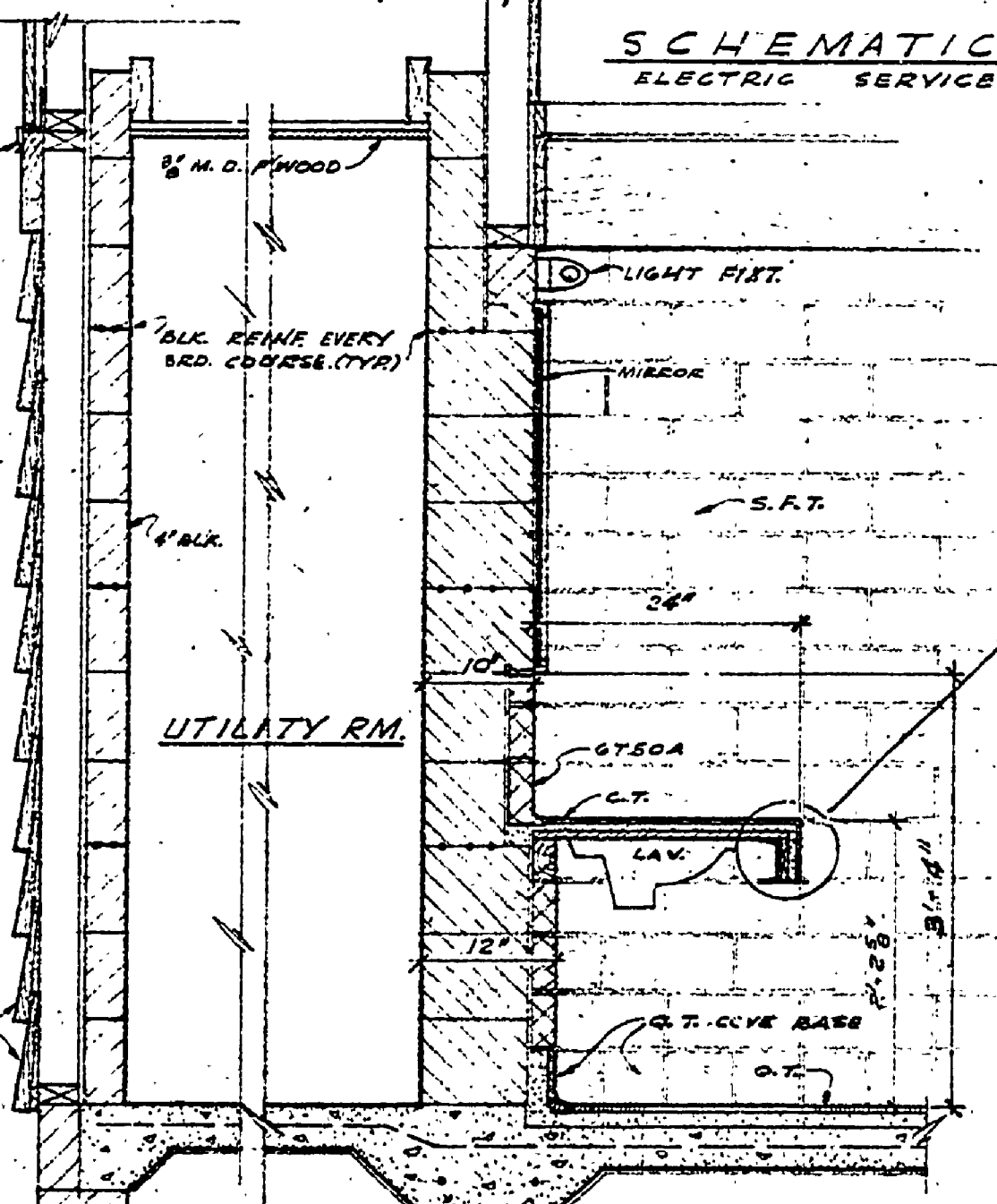
SECTION 3/8" = 1'-0"
