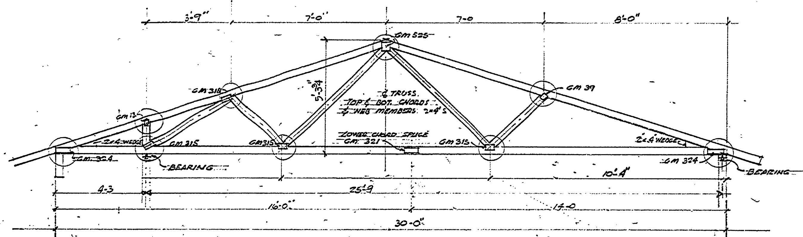
TRUSS DIAGRAM - TYPE - B SCALE 3/8" = 1'-0"
