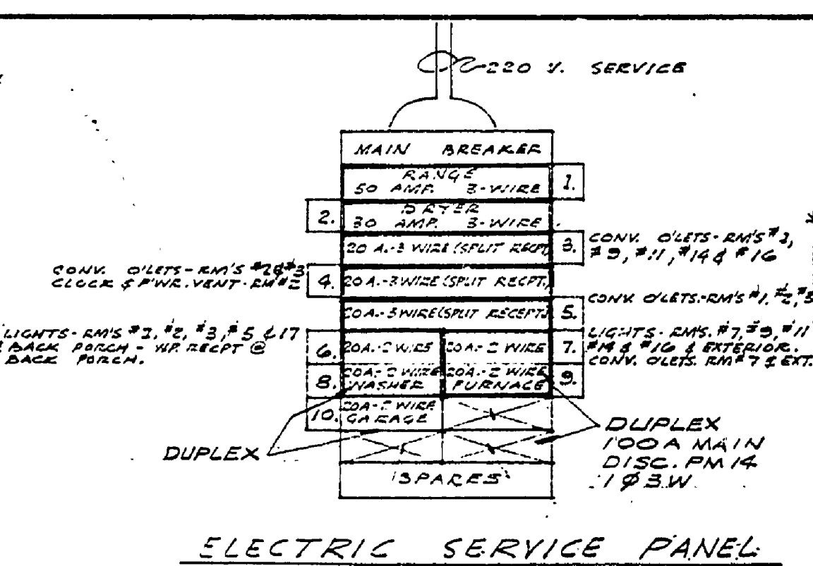
ELECTRIC SERVICE PANEL
