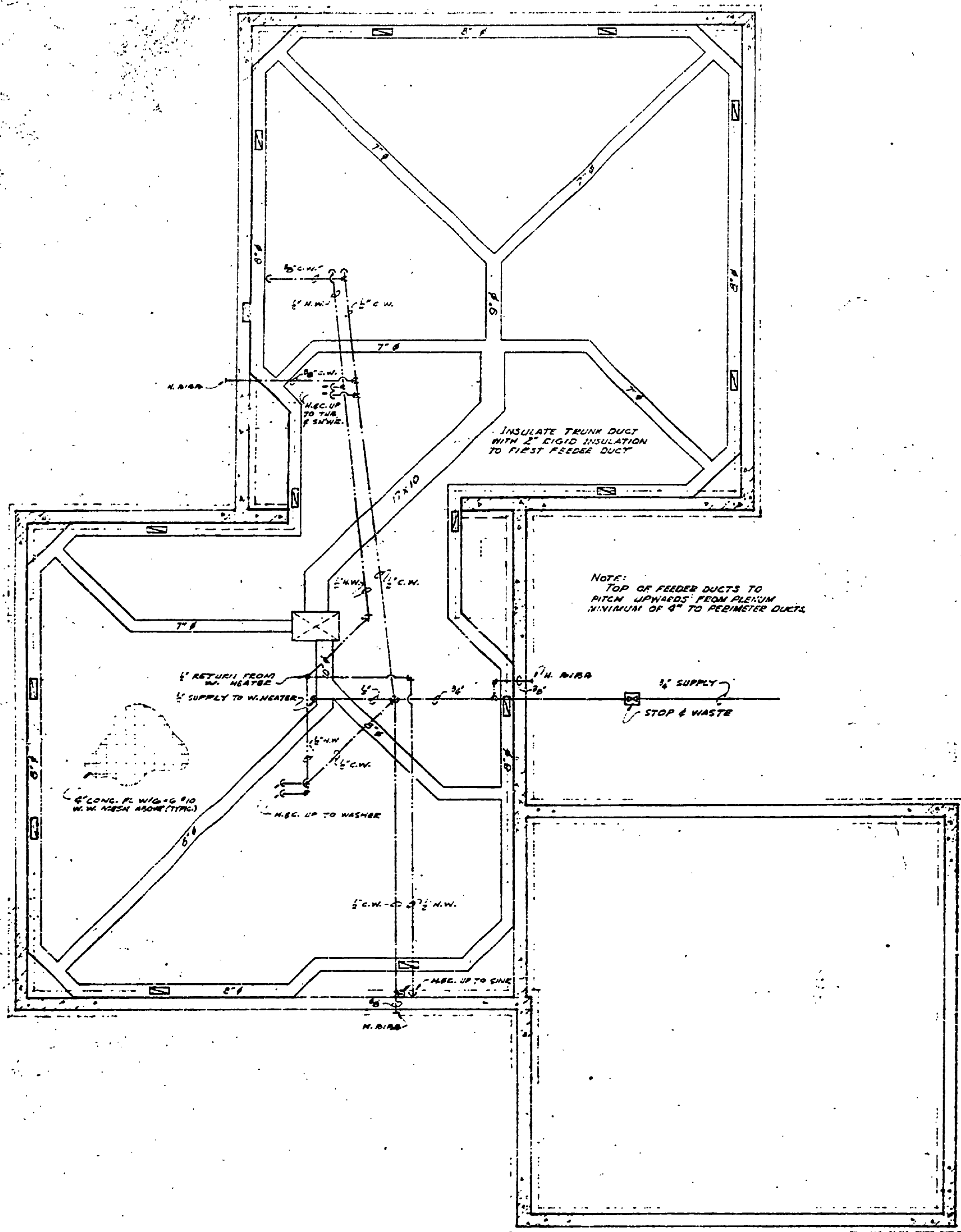
U.G. - HEATING & W. SUPPLY REVERSE PLAN
