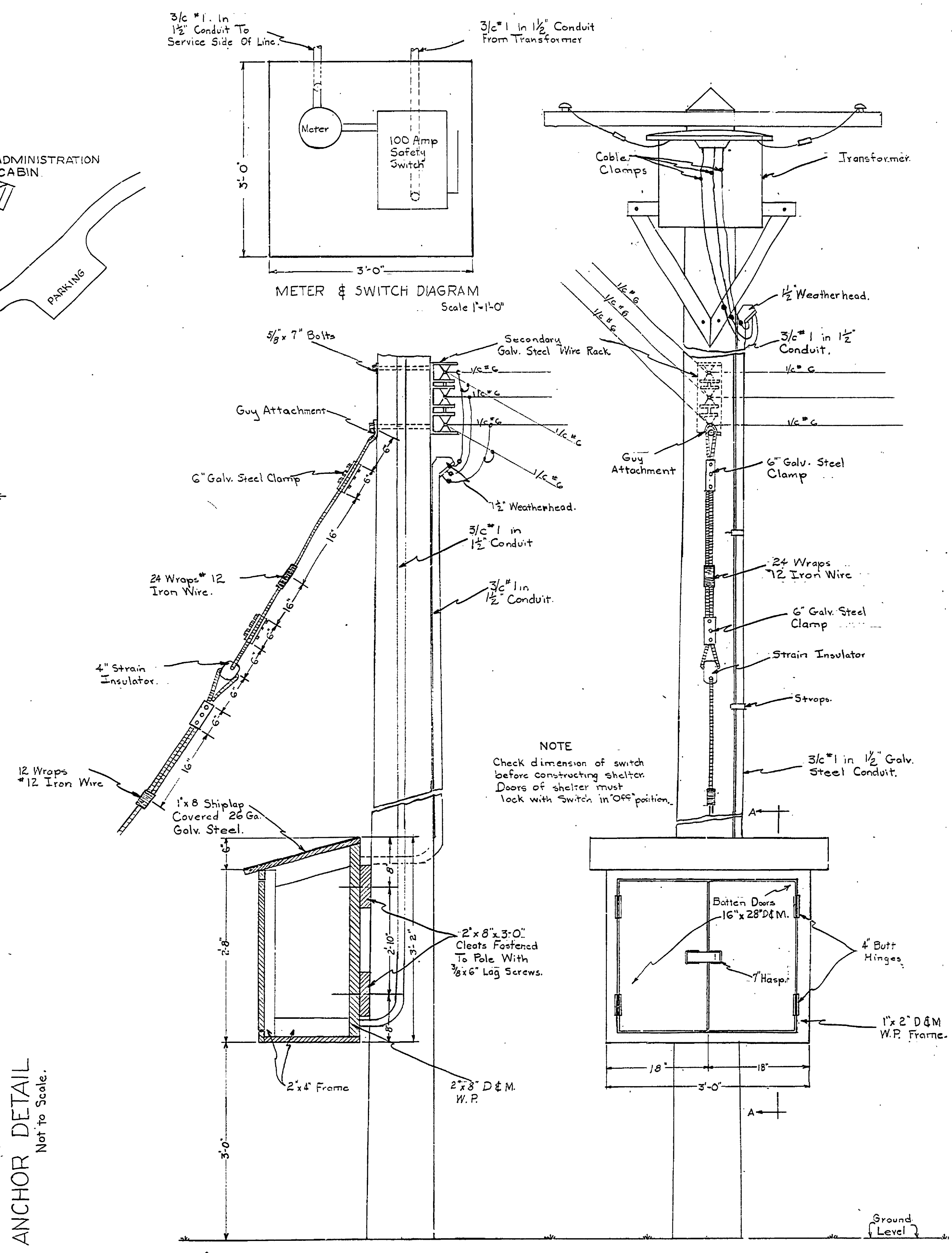
SECTION A-A FRONT VIEW SWITCH SHELTER DETAILS Scale 1"=1'-0"
