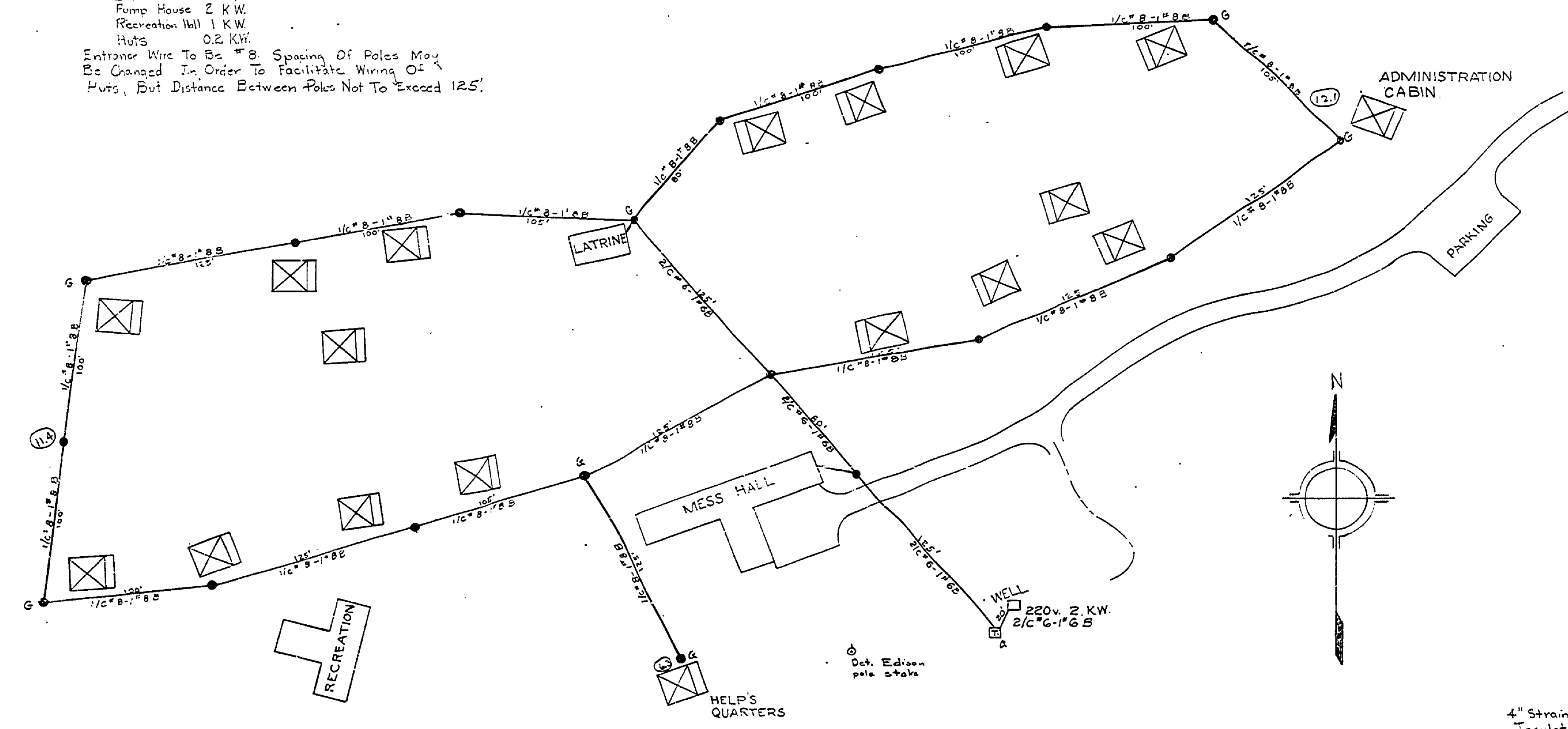
ELECTRICAL DISTRIBUTION SYSTEM PLAN Scale 1"=50'-0"
