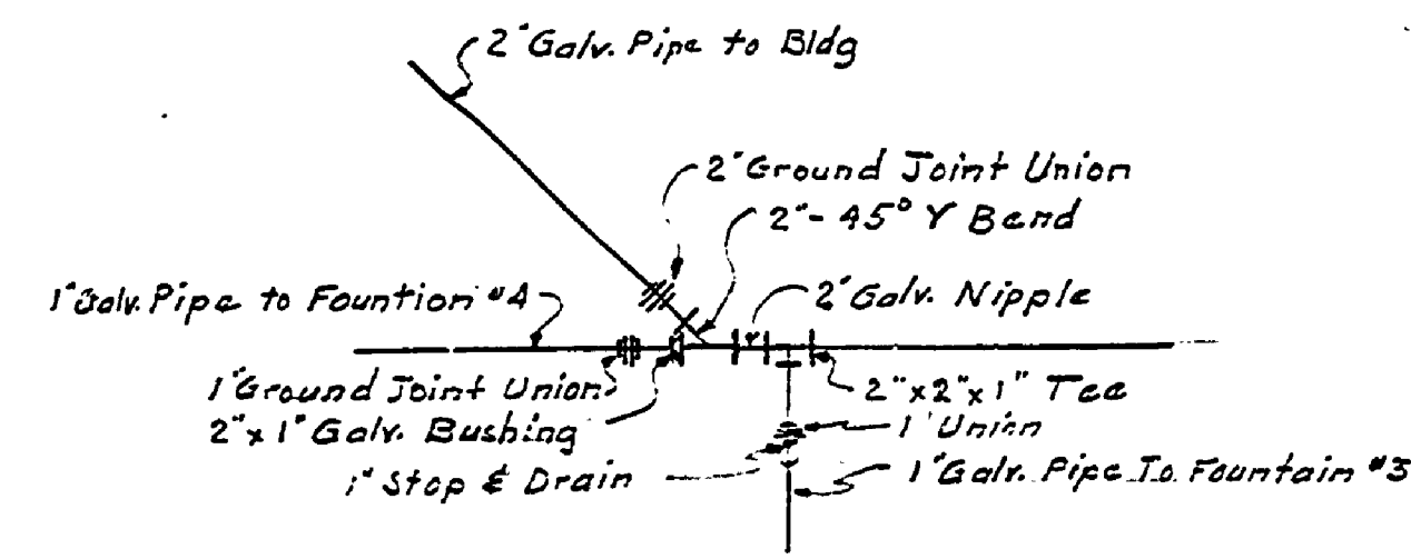
PIPE CONNECTIONS STA. 0+25 No SCALE
