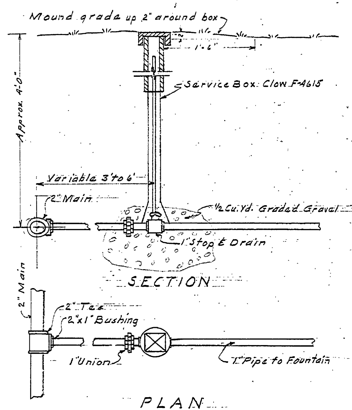
SECTION PLAN STOP AND DRAIN SCALE 1" = 1' 0"
