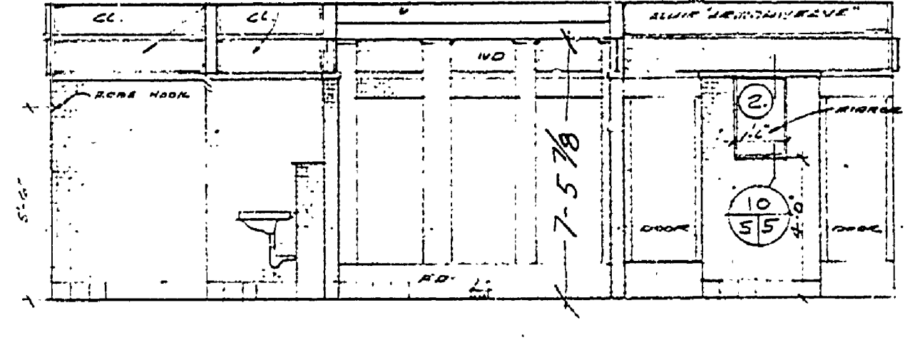
SOUTH INTERIOR ELEV. - MEN'S TOILET
