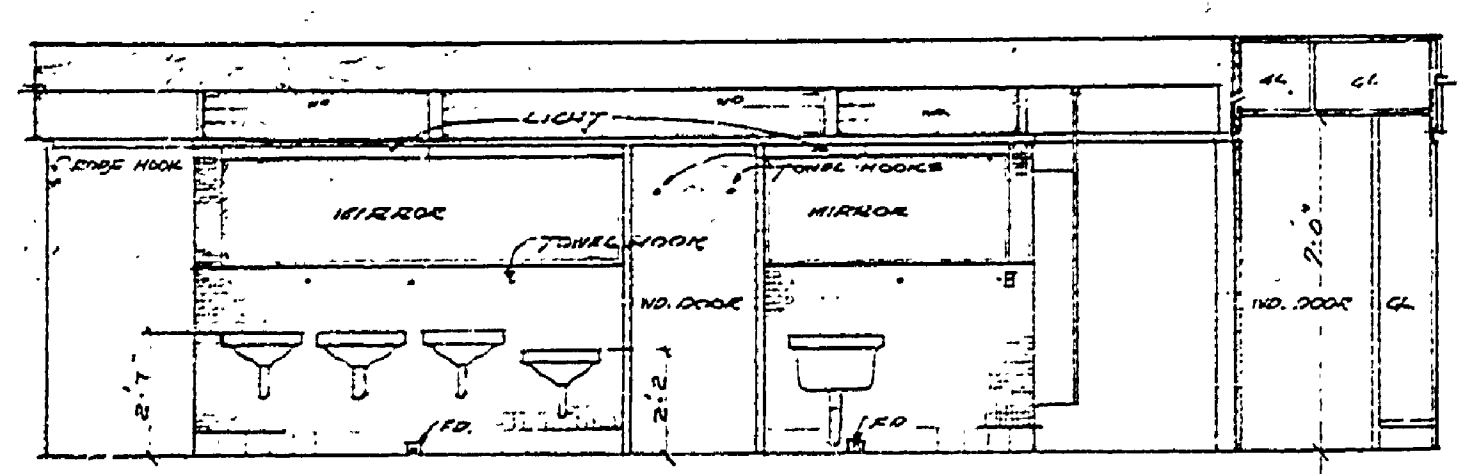
EAST INTERIOR ELEV. - WOMEN'S TOILET
