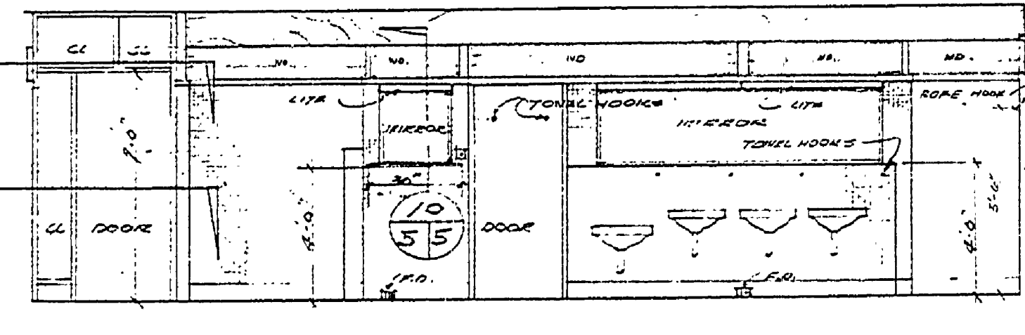
WEST INTERIOR ELEVATION - MEN'S TOILET
