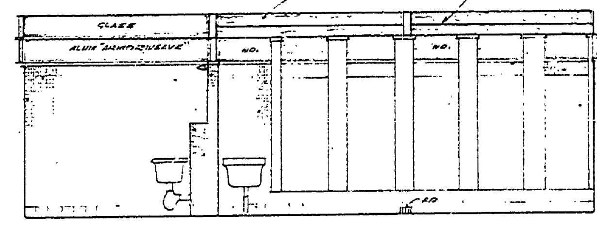
NORTH INTERIOR ELEV. - WOMEN'S TOILET
