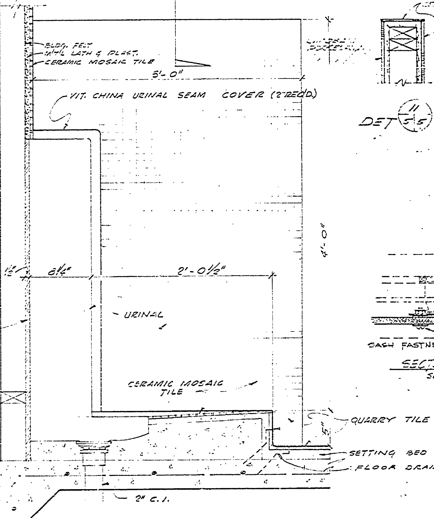
DET. 7 AT URINAL SCALE 1/2" = 1'-0"
