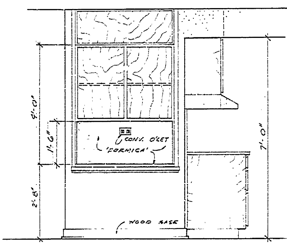
CHINA CAB. (DIN. RM.) SCALE - 1/2" = 1'-0"
