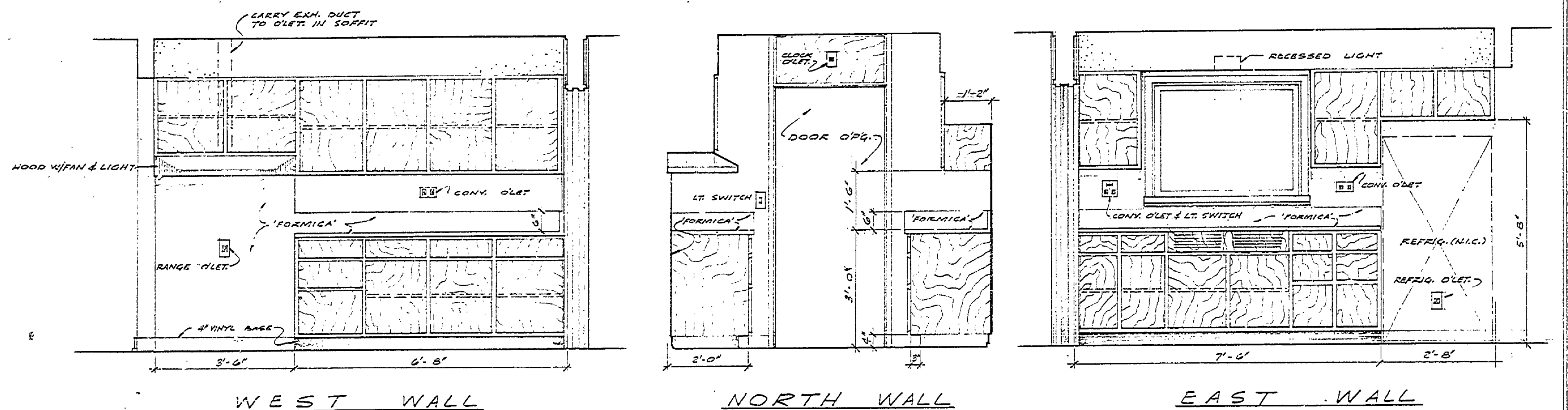
WEST WALL NORTH WALL EAST WALL KITCHEN CASES SCALE - 1/2" = 1'-0"
