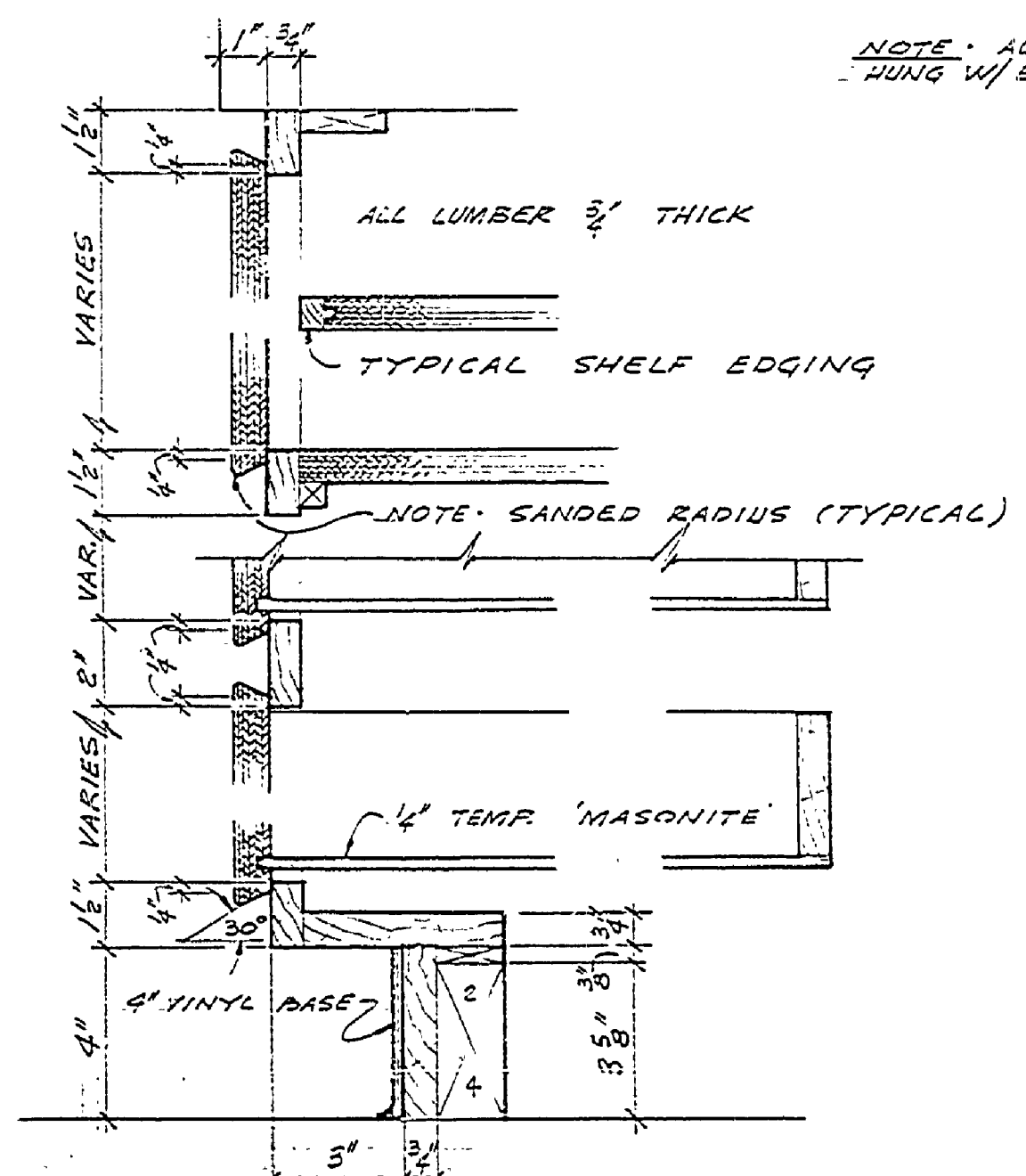
CABINET DETAILS SCALE - 3/8" = 1'-0"
