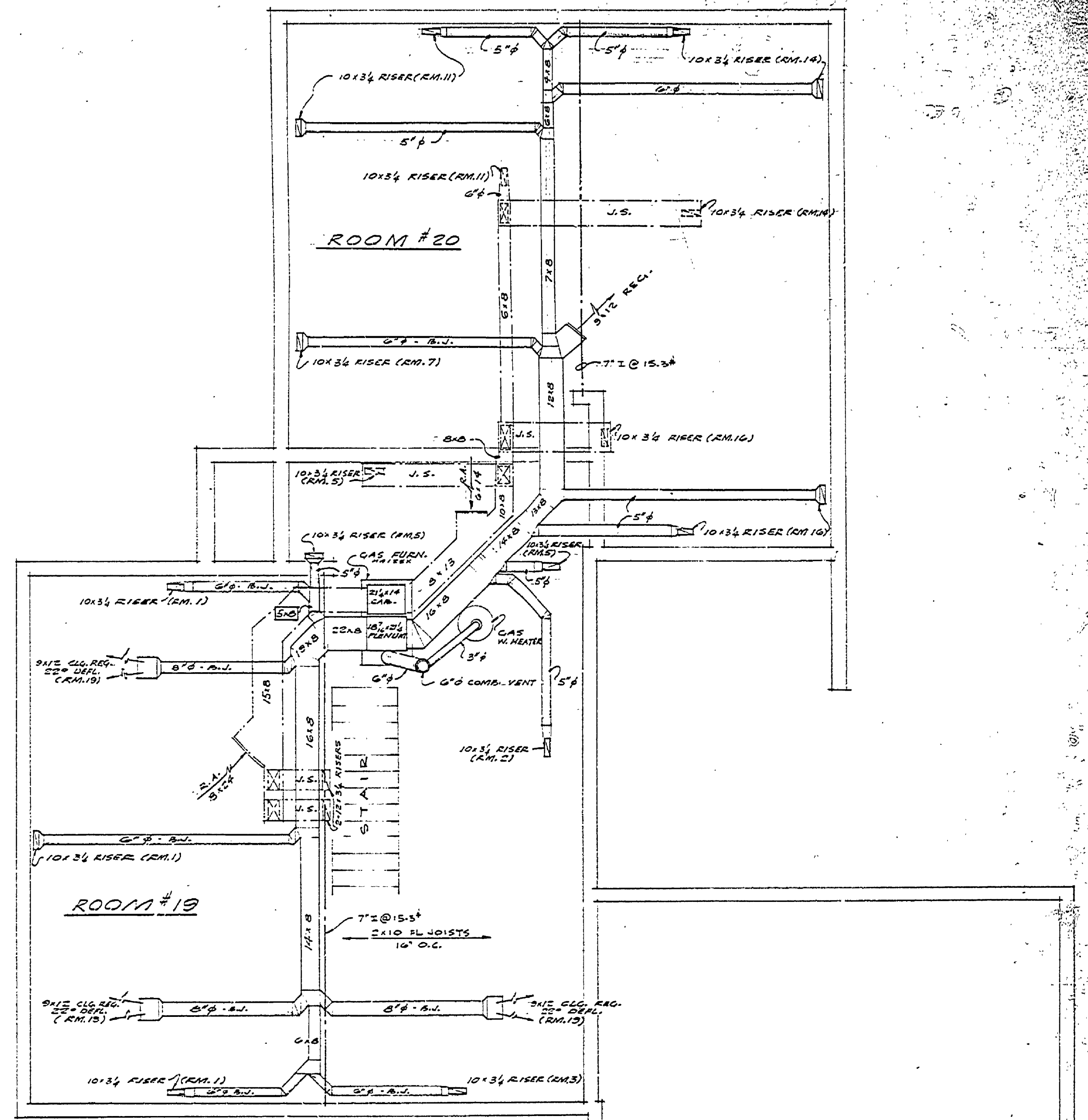
HEATING PLAN - BASEMENT SCALE - 1/4" = 1'-0"
