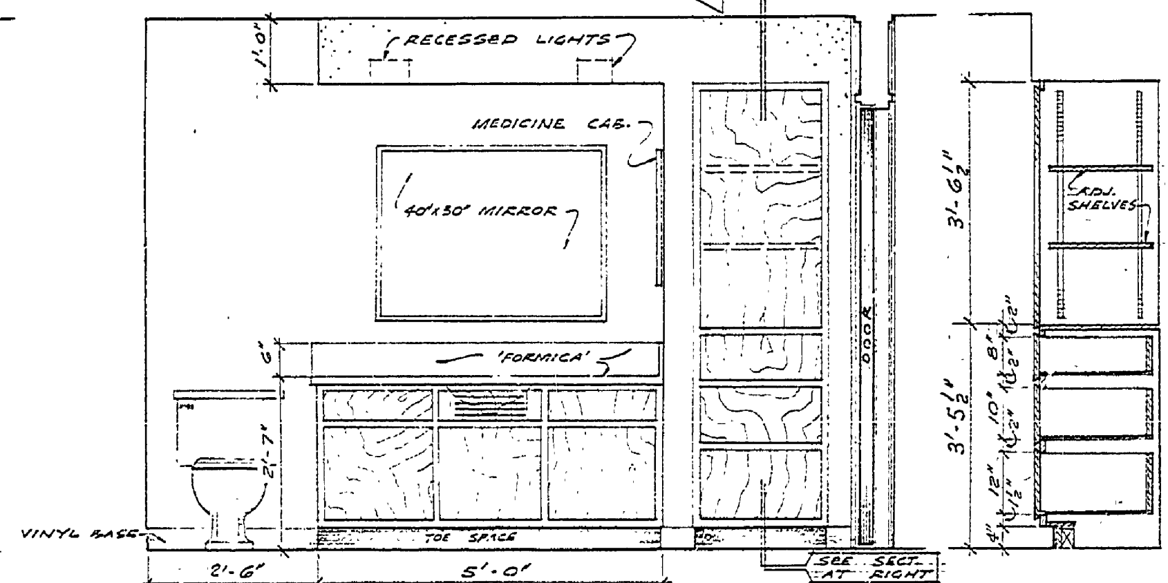
NORTH WALL (BATH) SECT. - LINEN CAB SCALE - 1/2" = 1'-0"
