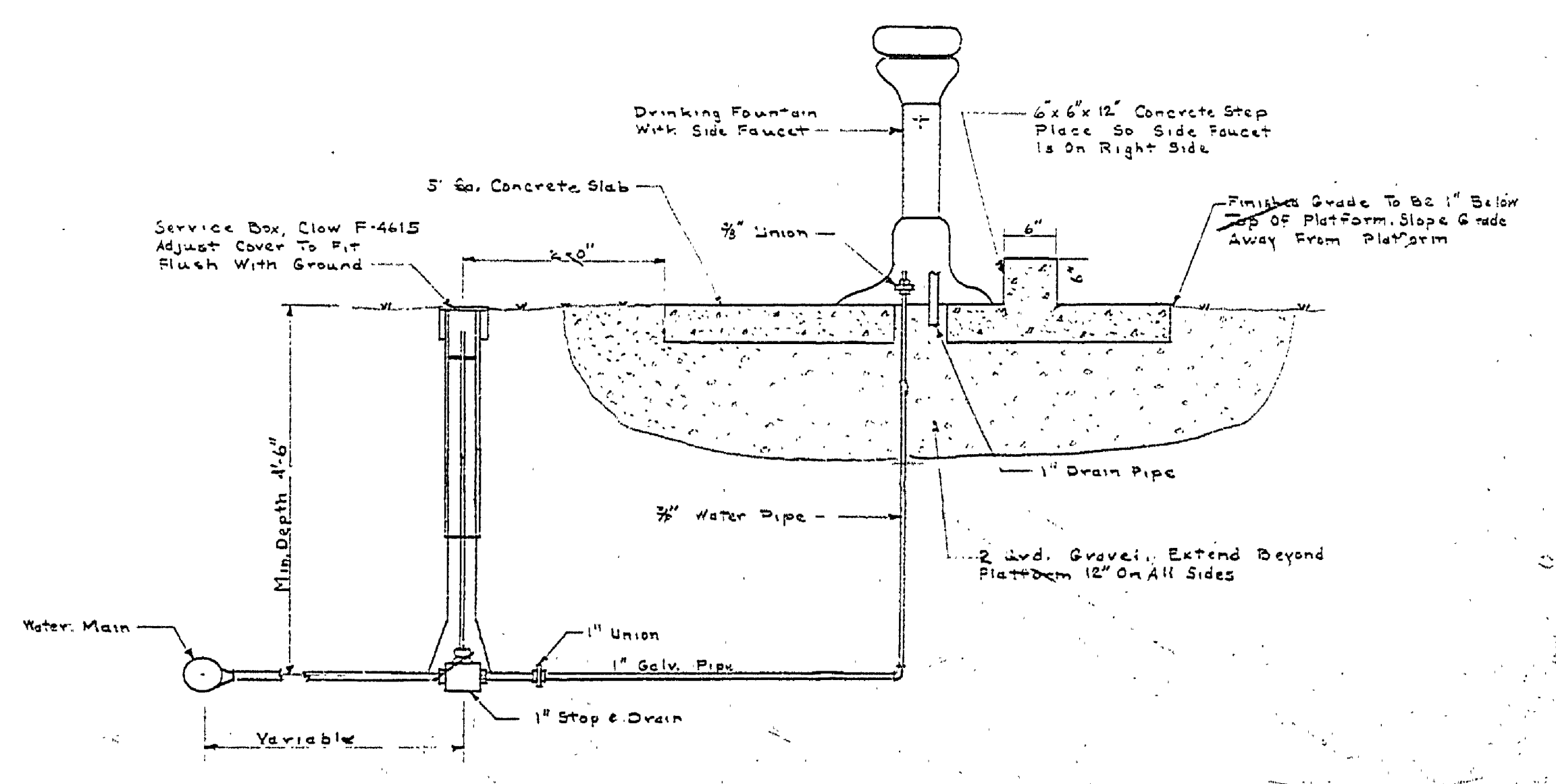
DETAIL OF DRINKING FOUNTAIN TO BE SALVAGED Scale 3/4\"/>
