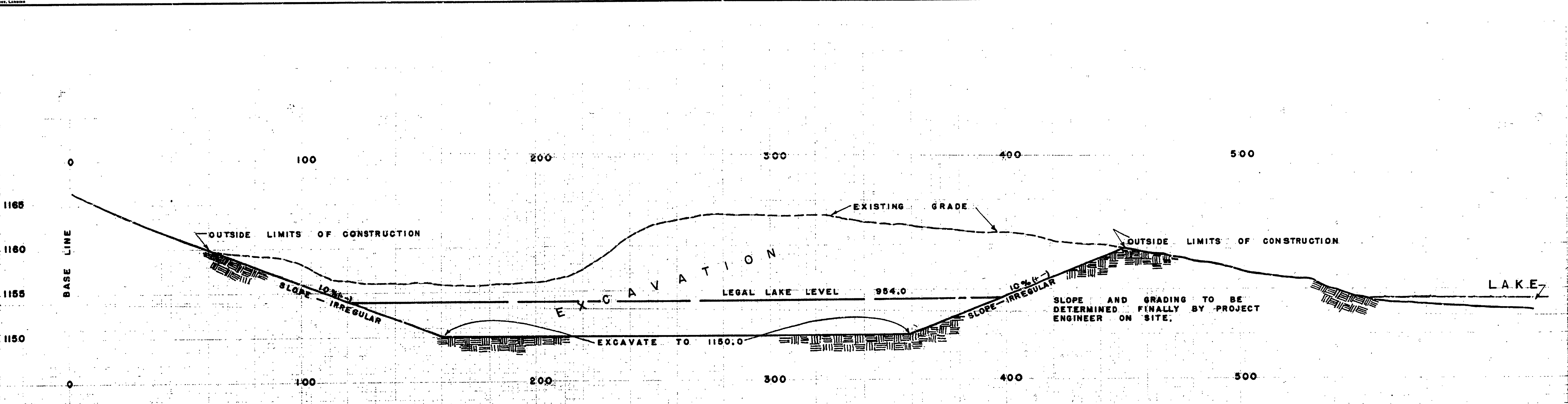
LAGOON EARTH EXCAVATION DETAIL DETAIL "F"
