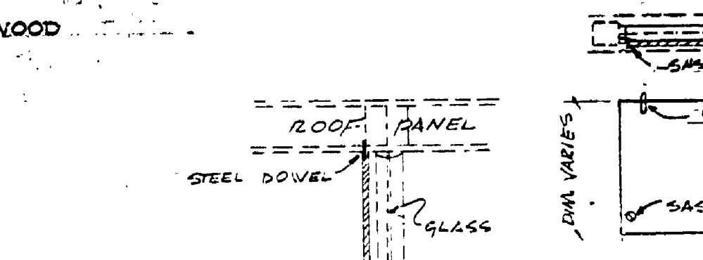
DETAILS - WINTERIZING PANEL NO SCALE
