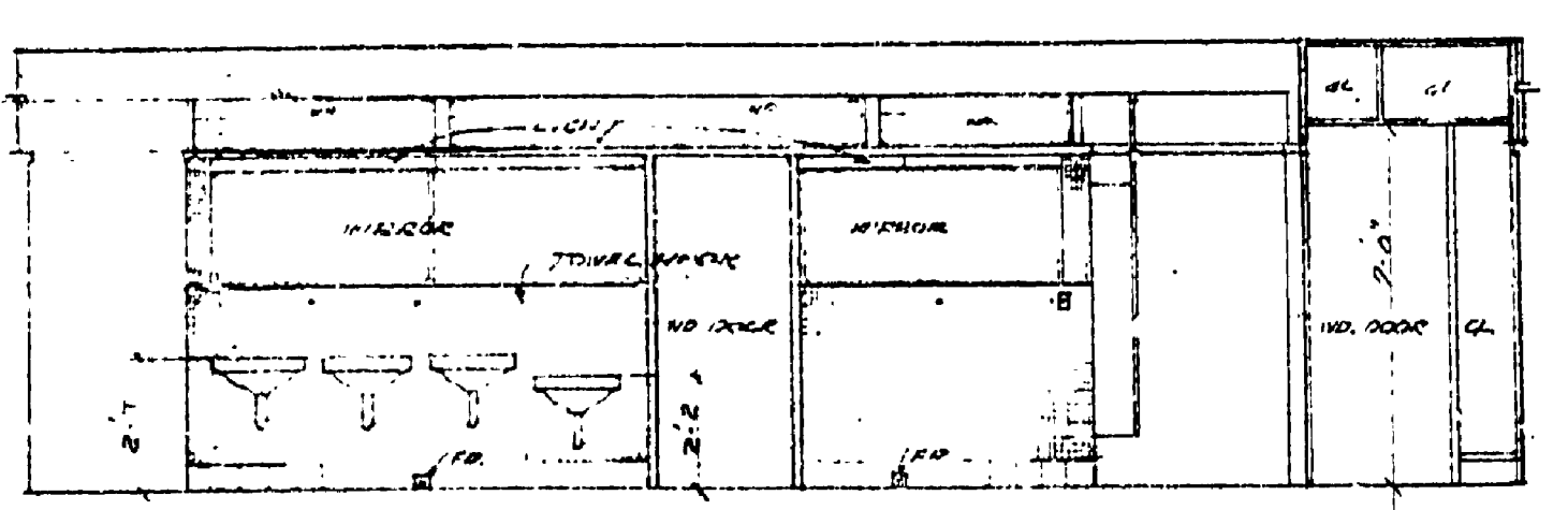
WEST INTERIOR ELEV. - WOMEN'S TOILET SCALE: 1/8" = 1'-0"
