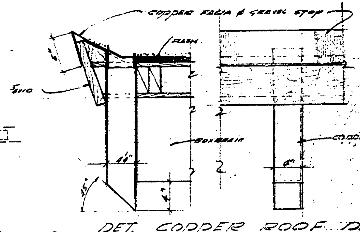
DET. COPPER ROOF DRAIN & REED SCALE: 1/8" = 1'-0"
