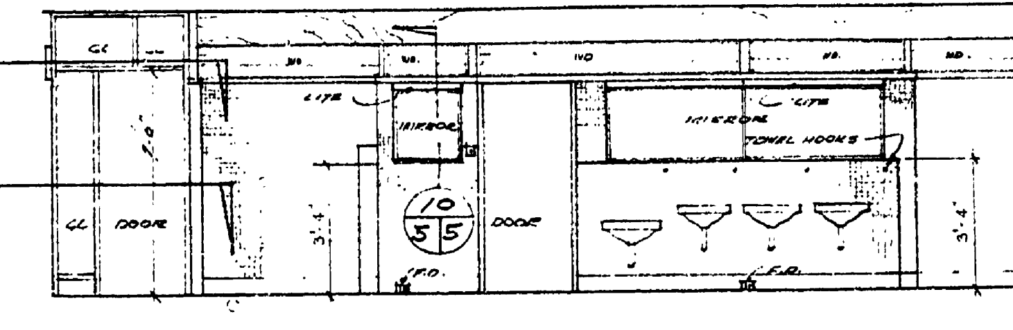
EAST INTERIOR ELEVATION - MEN'S TOILET SCALE: 1/8" = 1'-0"
