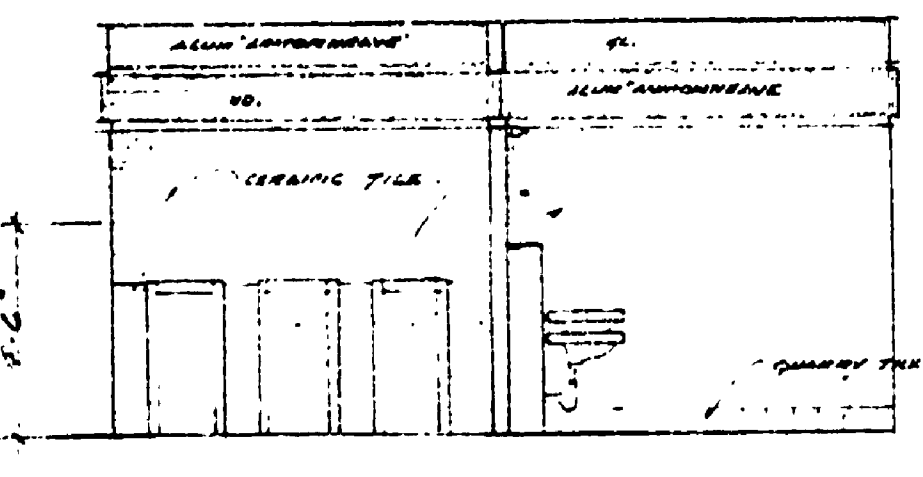
SOUTH INT. ELEV. - MEN'S TOILET SCALE: 1/8" = 1'-0"
