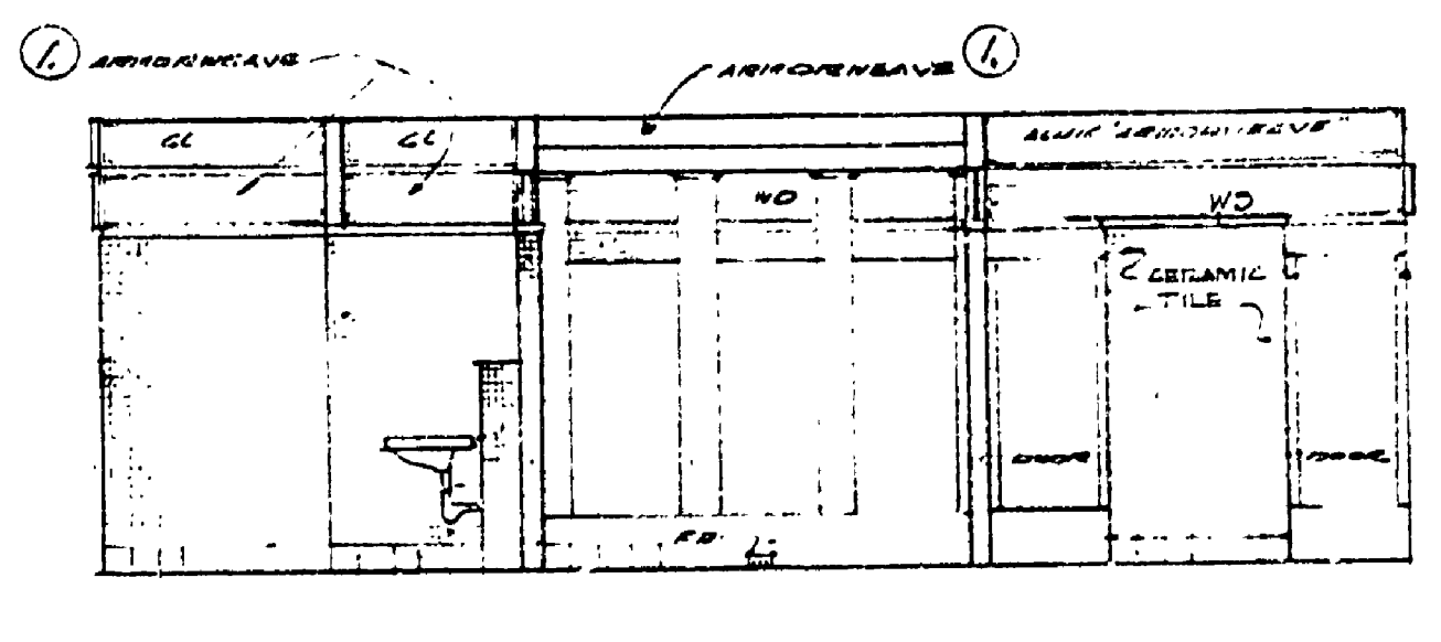
NORTH INTERIOR ELEV. - MEN'S TOILET SCALE: 1/8" = 1'-0"
