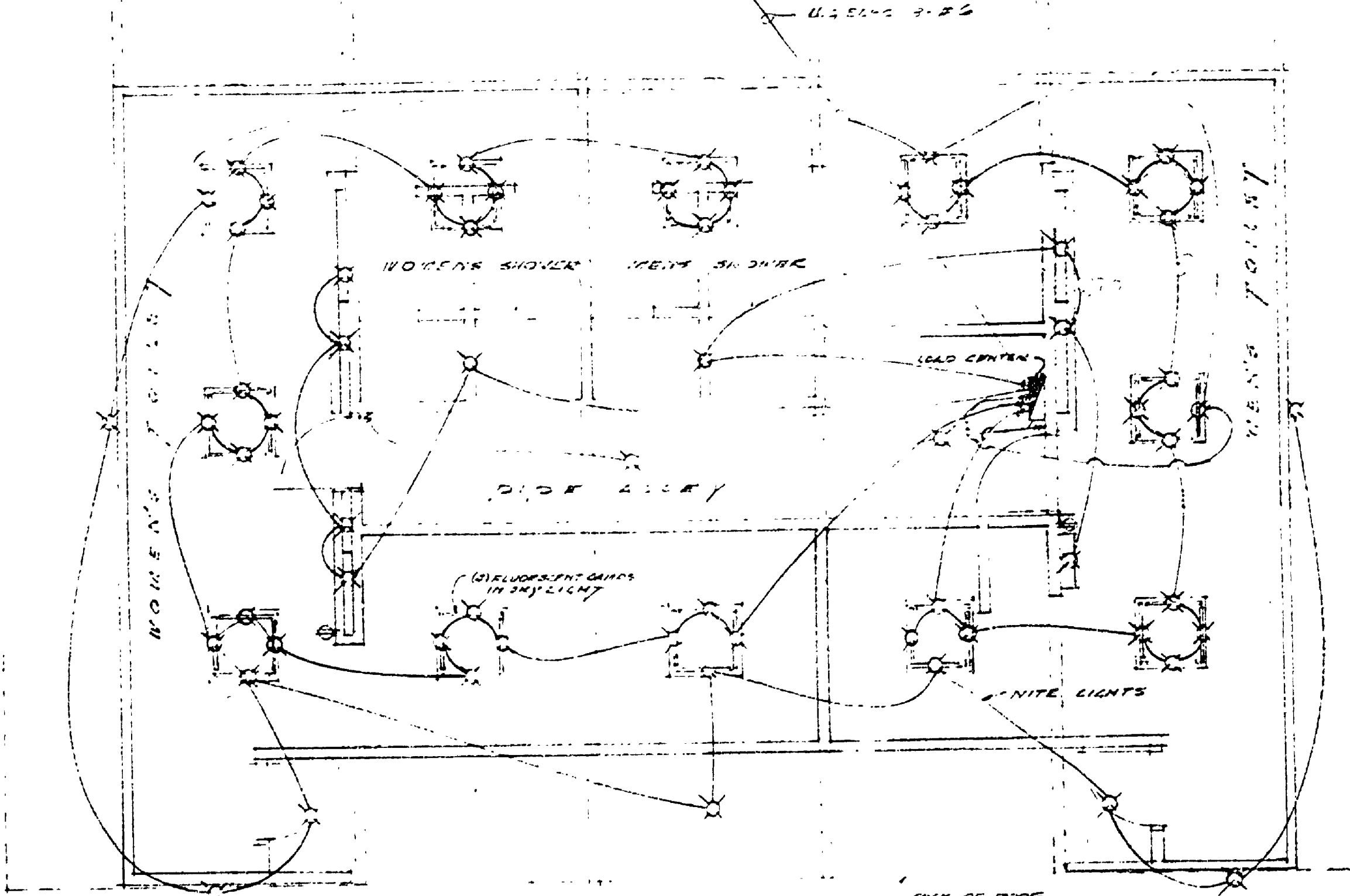
ELECTRICAL LIGHTING PLAN SCALE: 1/8" = 1'-0"
