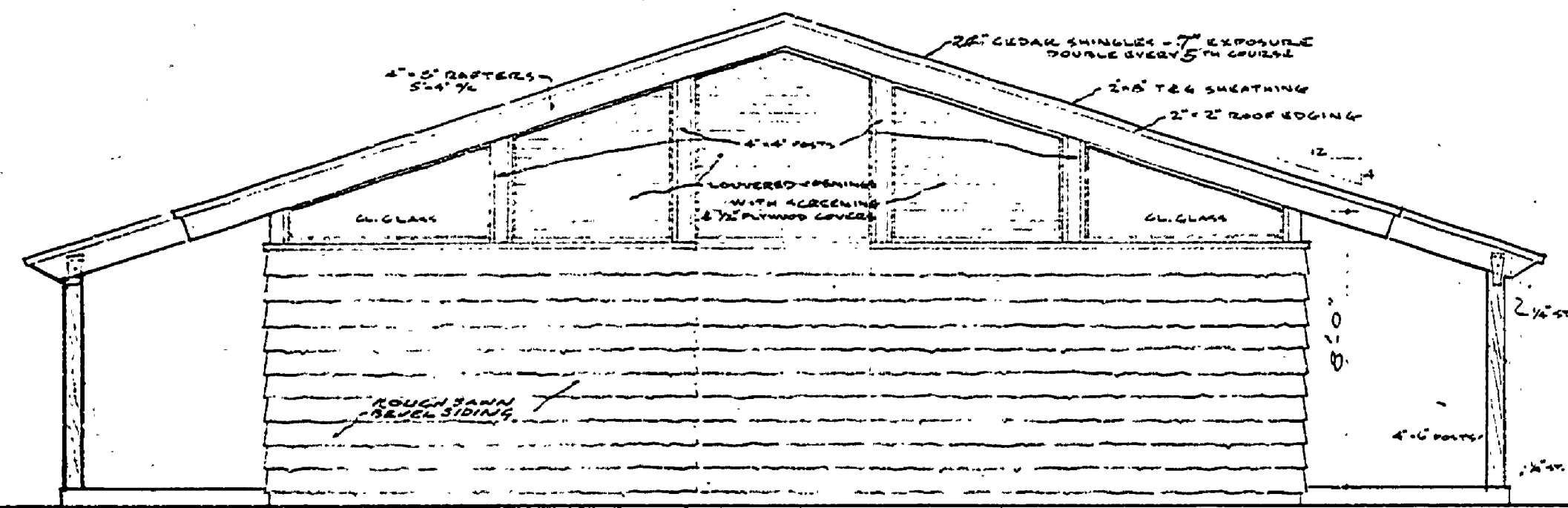
NORTH ELEVATION 1/4" = 1'-0"
