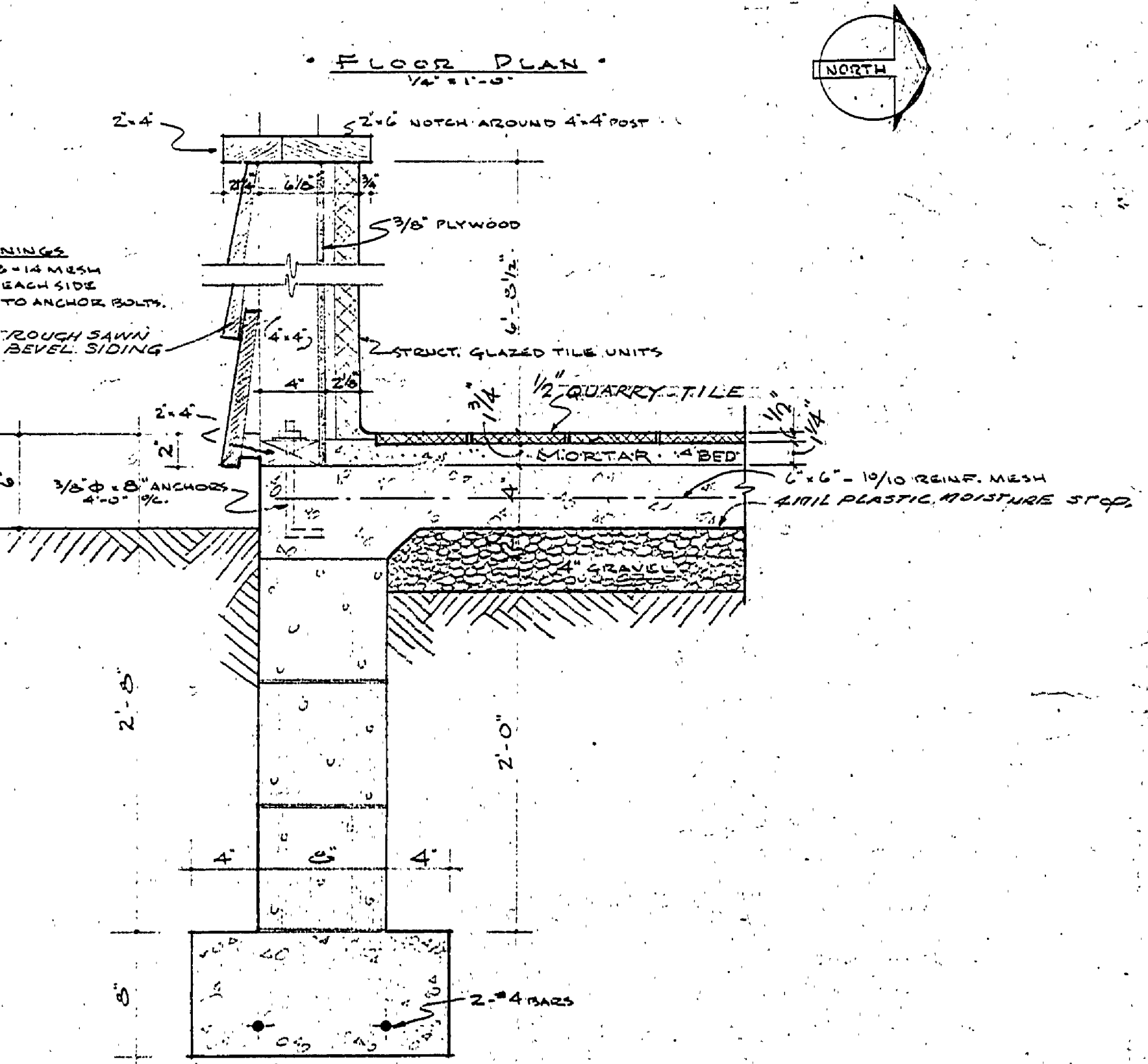
FOUNDATION SECTION 1/2" = 1'-0"
