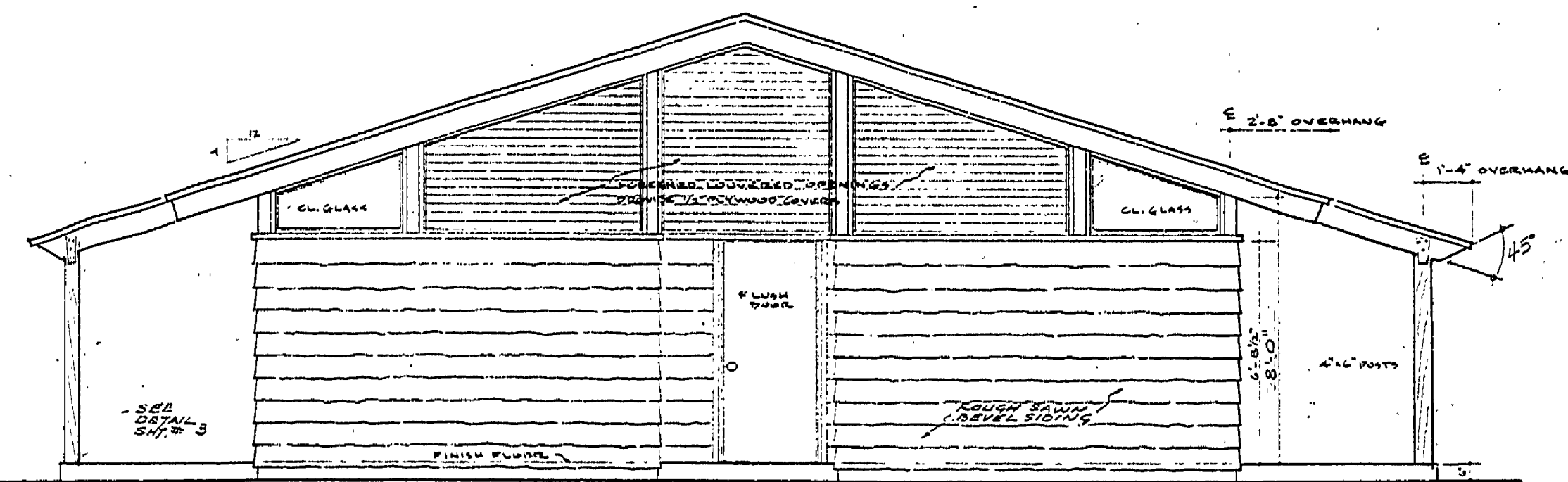
SOUTH ELEVATION 1/4" = 1'-0"
