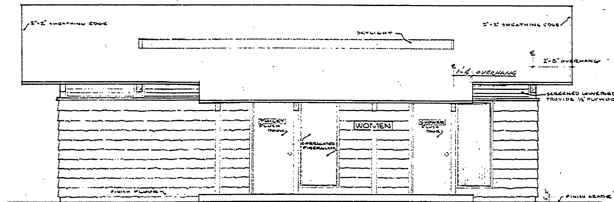
WEST ELEVATION 1/4" = 1'-0"
