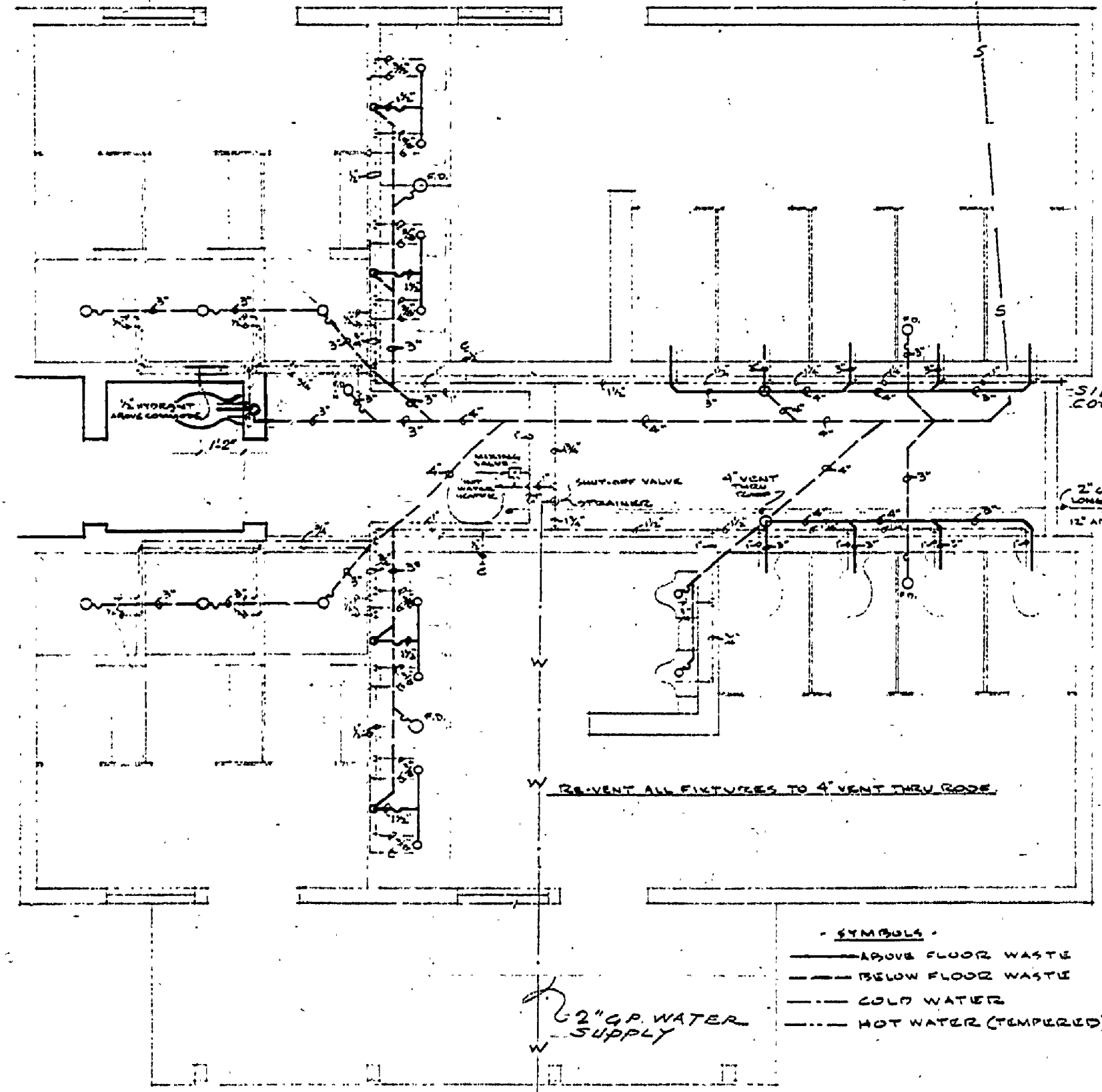
PLUMBING PLAN 1/4" = 1'-0"
