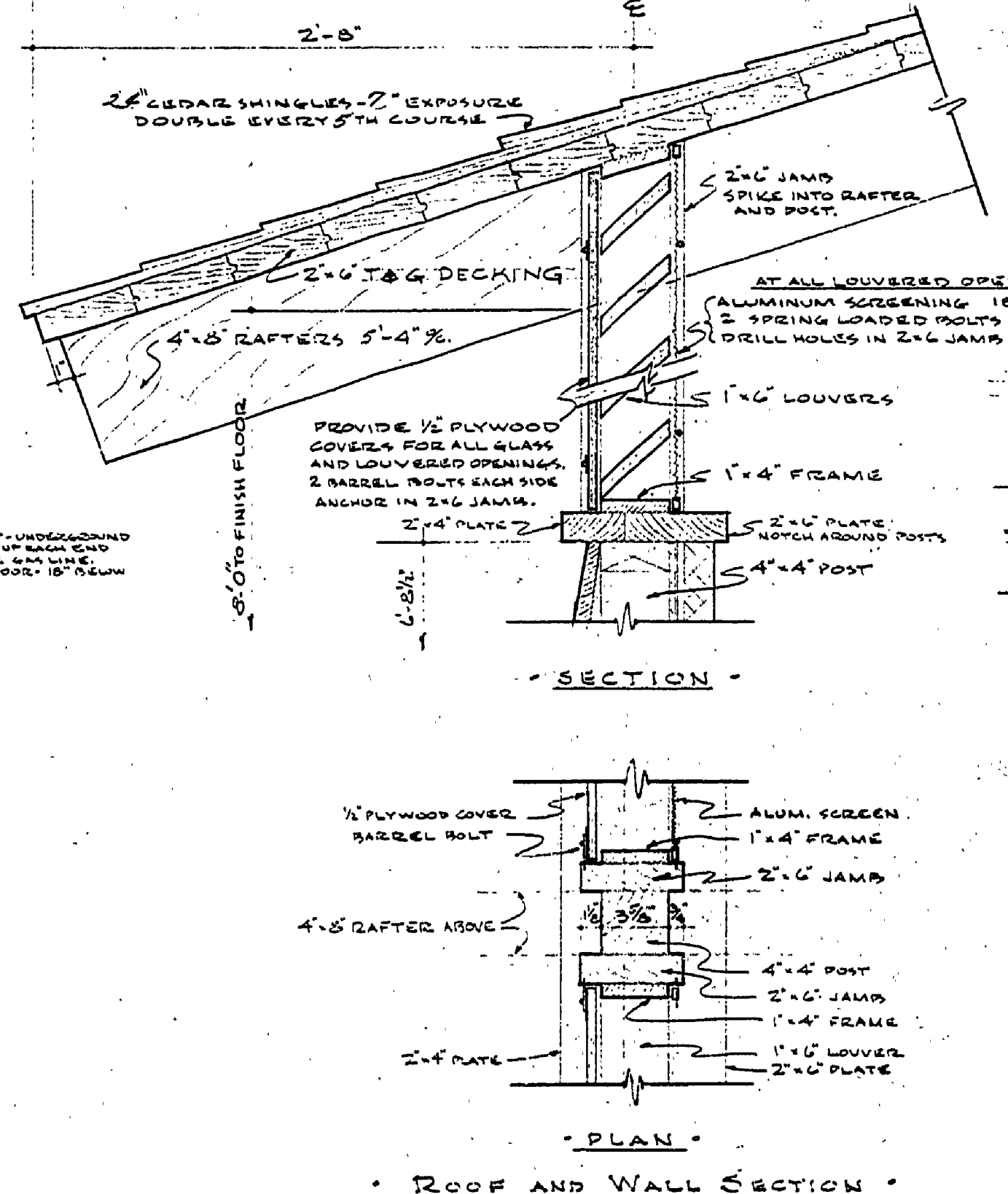
ROOF AND WALL SECTION 1/2" = 1'-0"
