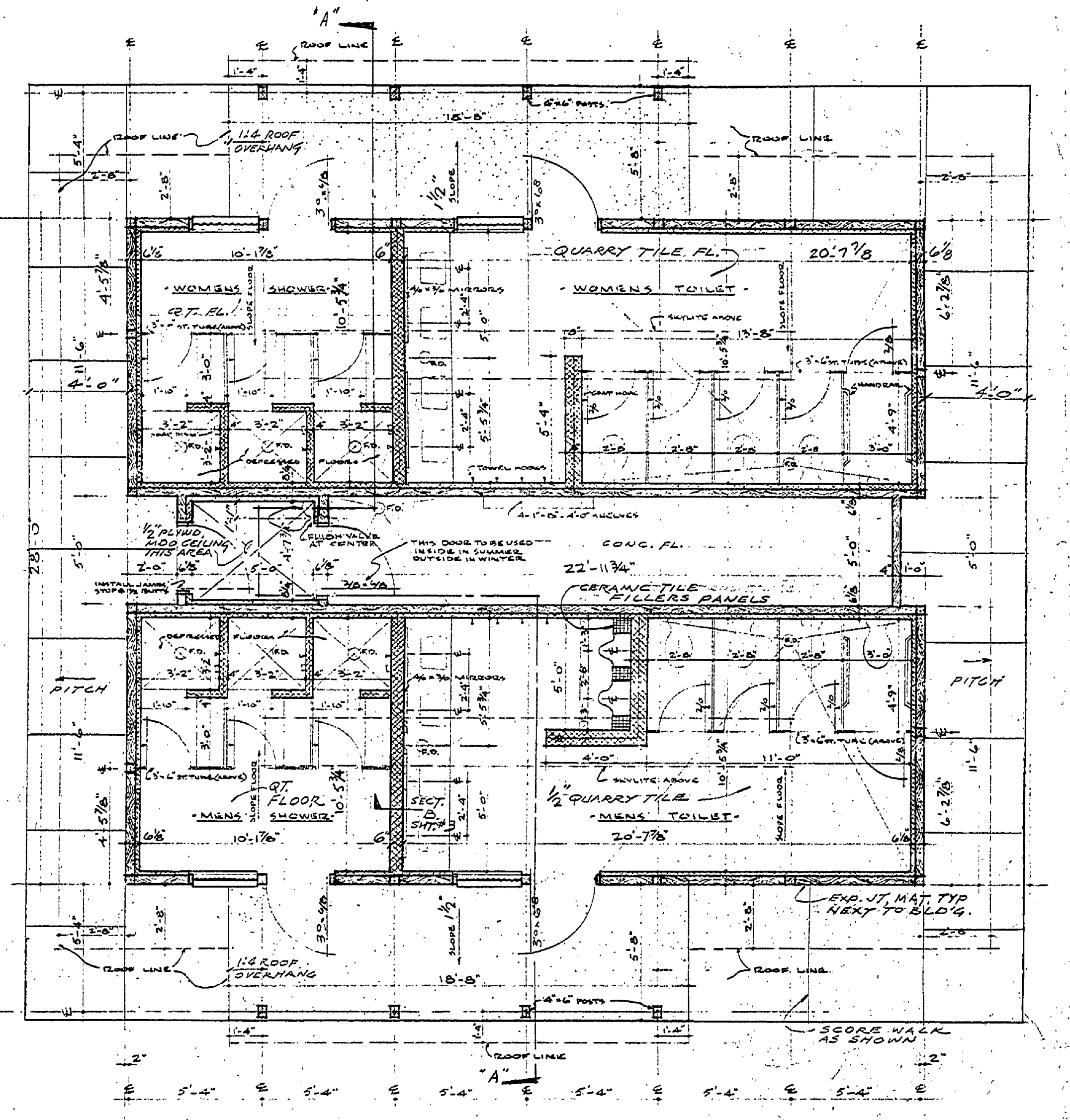
FLOOR PLAN 1/4" = 1'-0"
