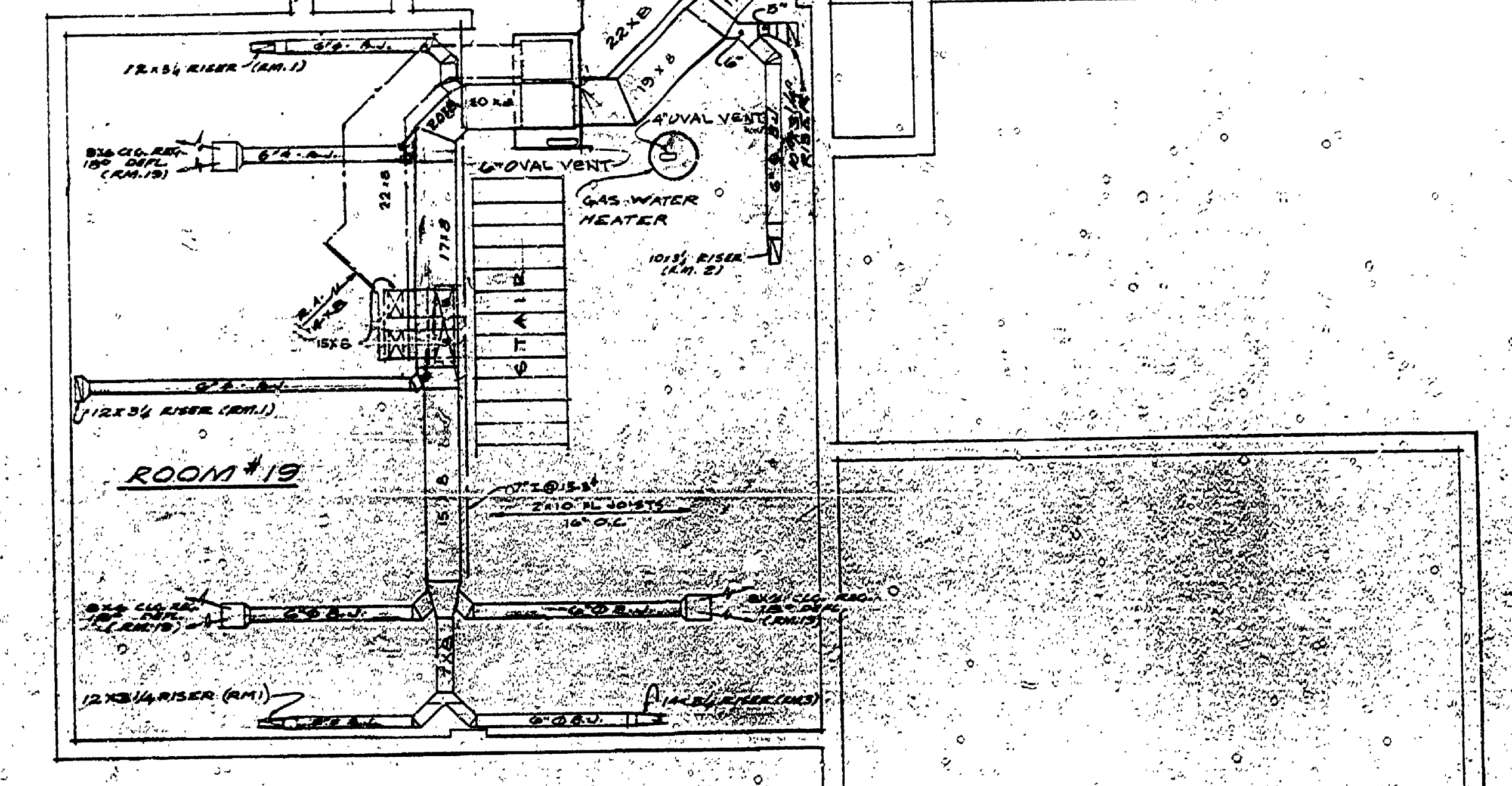
HEATING PLAN - BASEMENT SCALE 1/2" = 1'-0"
