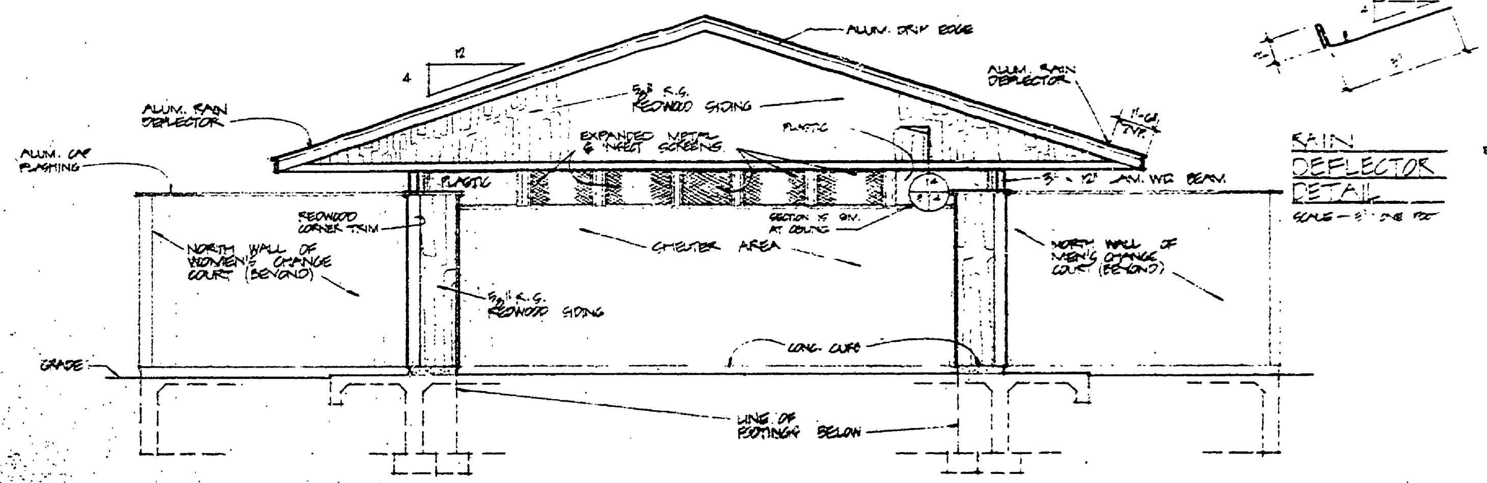
NORTH ELEVATION SCALE - 1/4" = ONE FOOT
