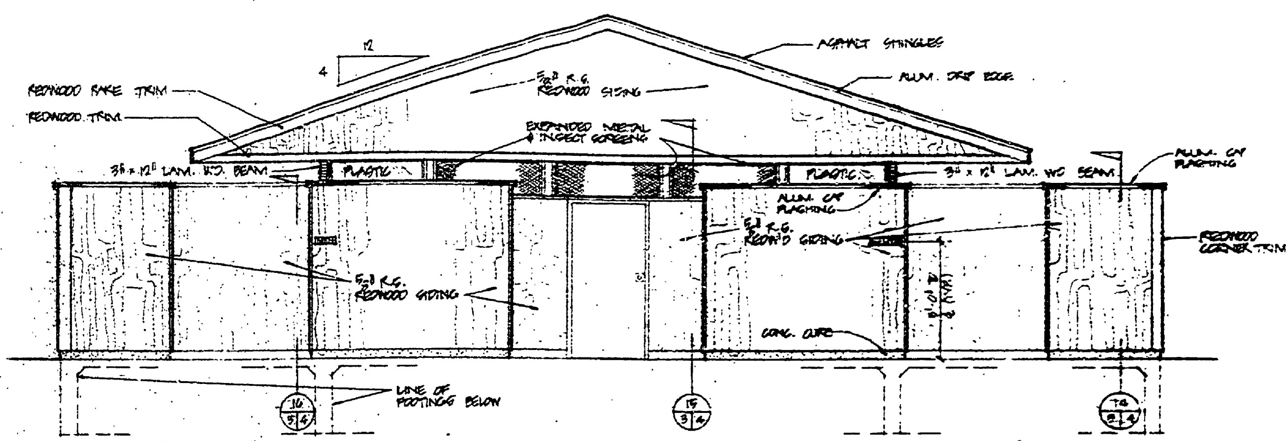
SOUTH ELEVATION SCALE - 1/4" = ONE FOOT
