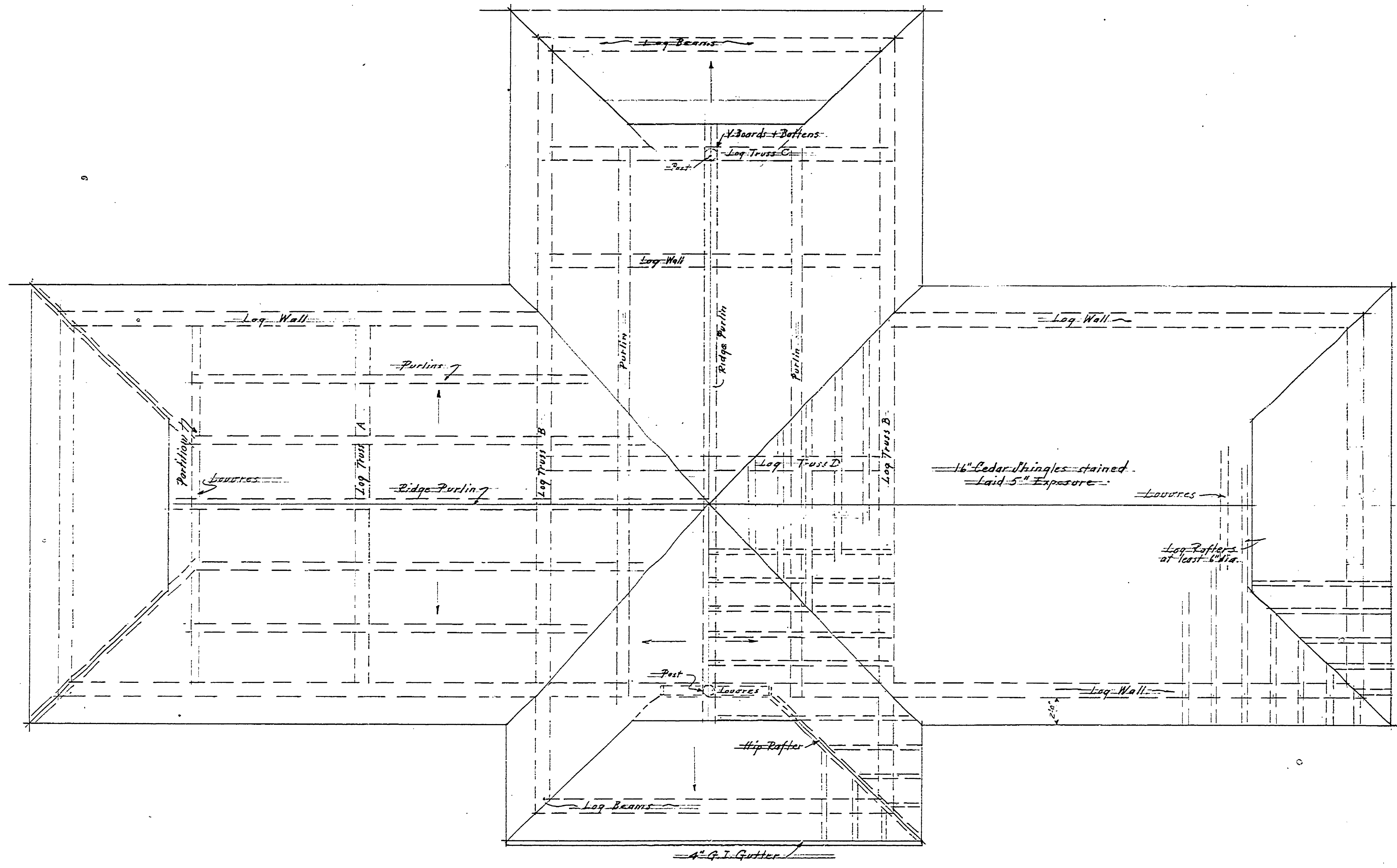
R O O F P L A N Scale \frac{1}{4}'' = 1'-0''
