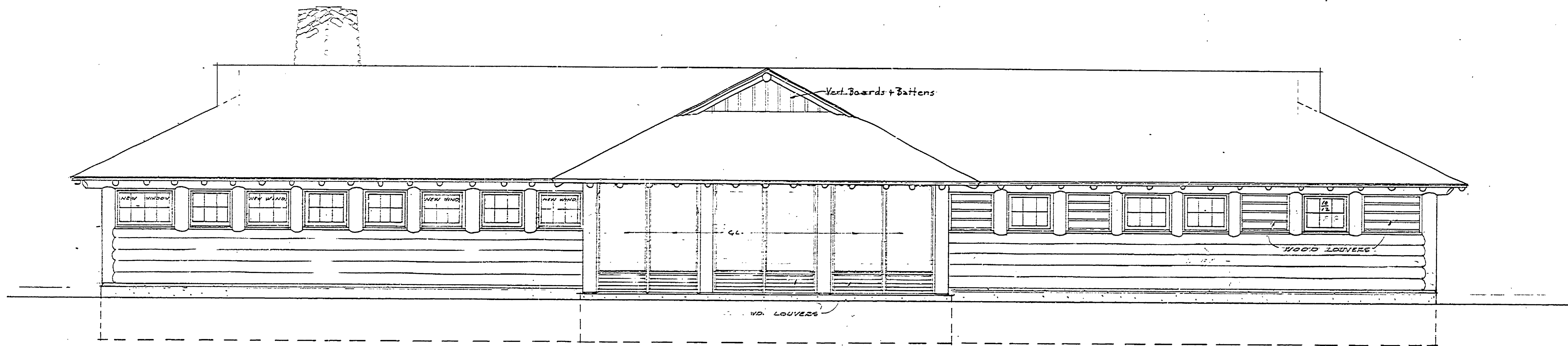
LAKE (NORTH) ELEVATION
