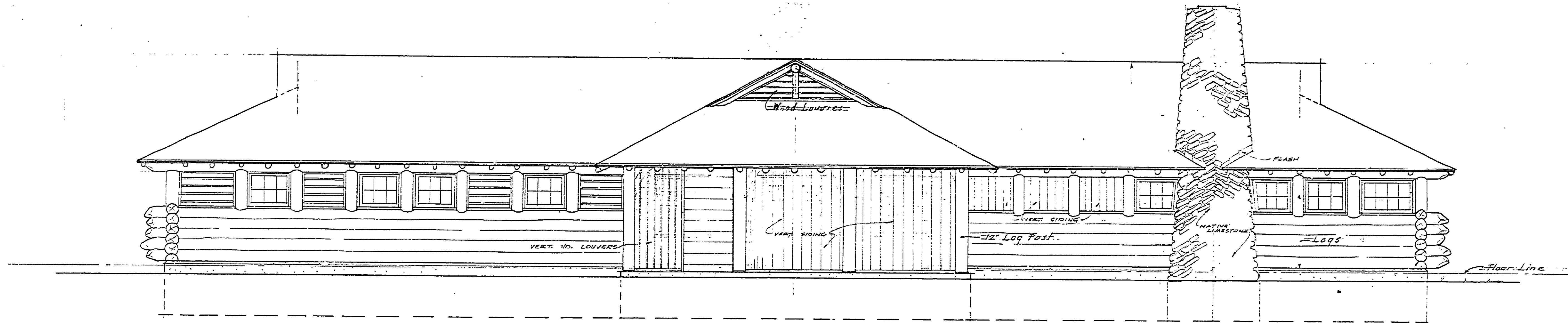
ENTRANCE (SOUTH) ELEVATION
