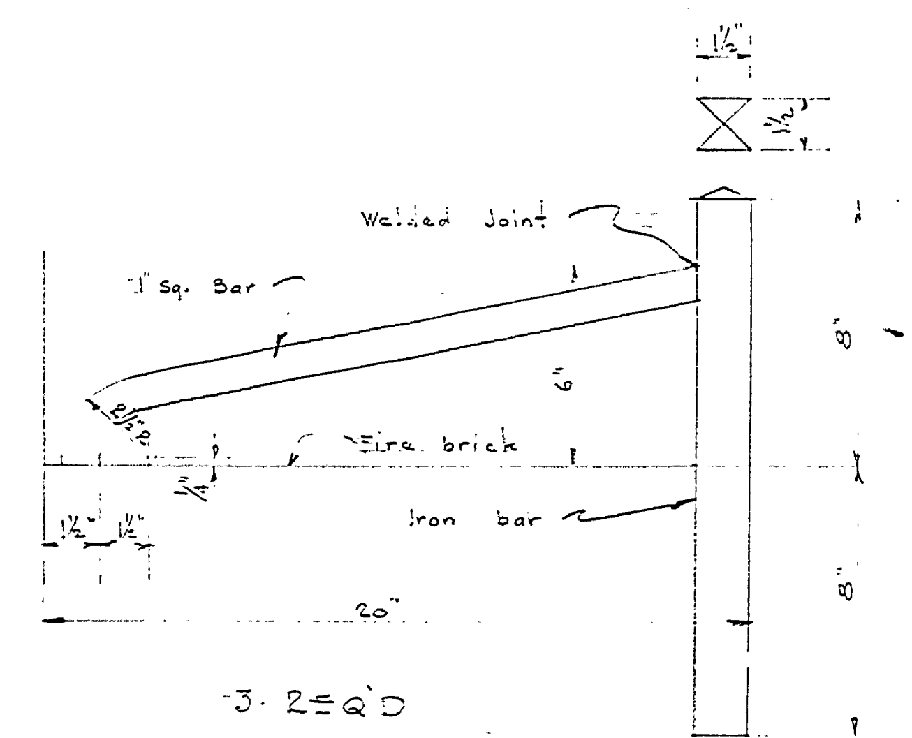
ELEVATION OF END IRONS Scale 1/2" = 1'-0"
