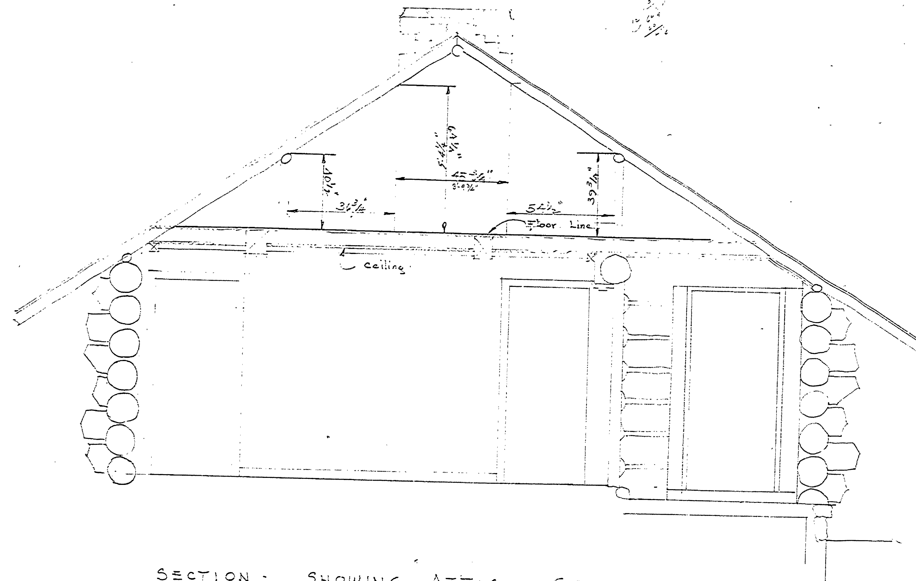
SECTION - SHOWING ATTIC SPACE. scale 1/4" = 1'-0"
