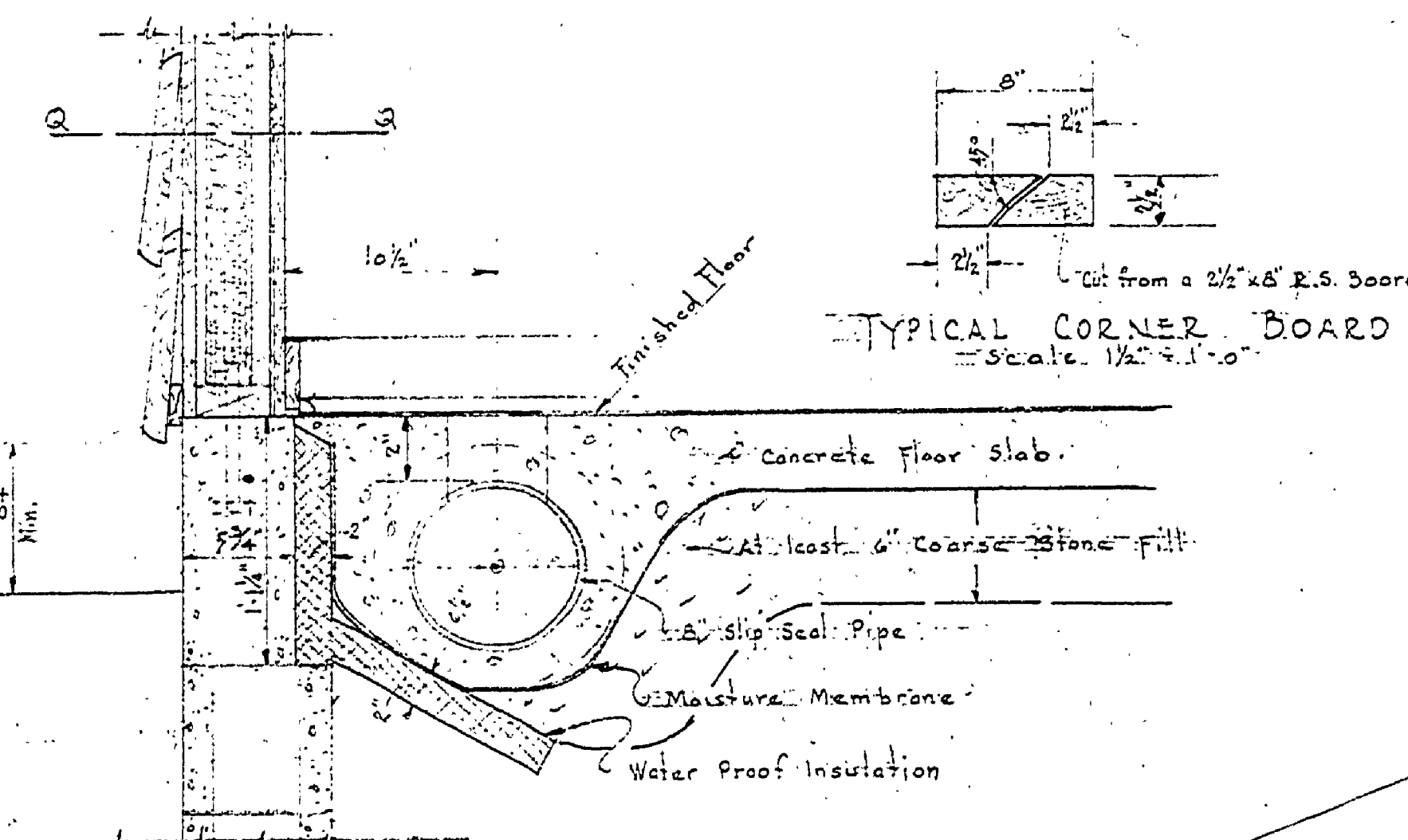
HEATING DUCT DETAIL Scale 1/4" = 1'-0"
