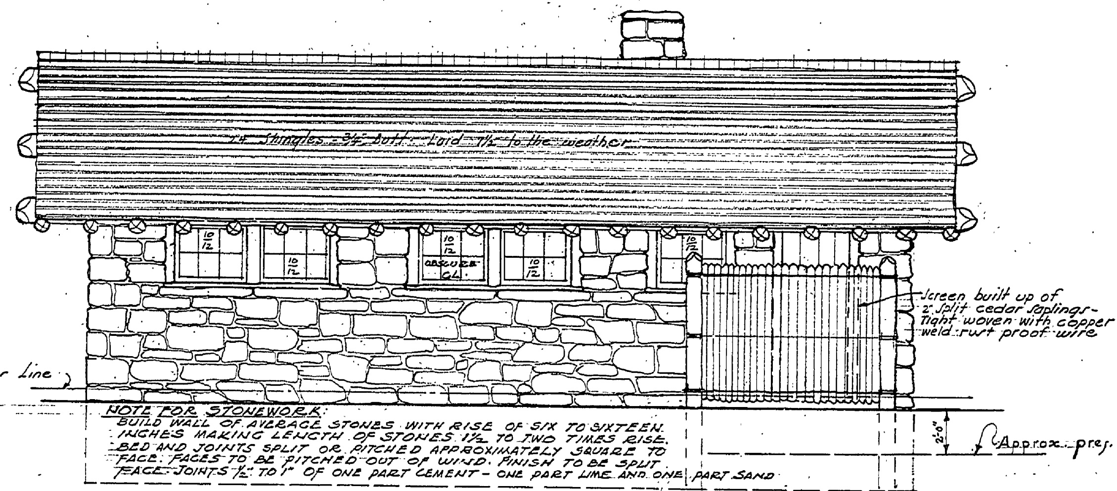
FRONT ELEVATION
