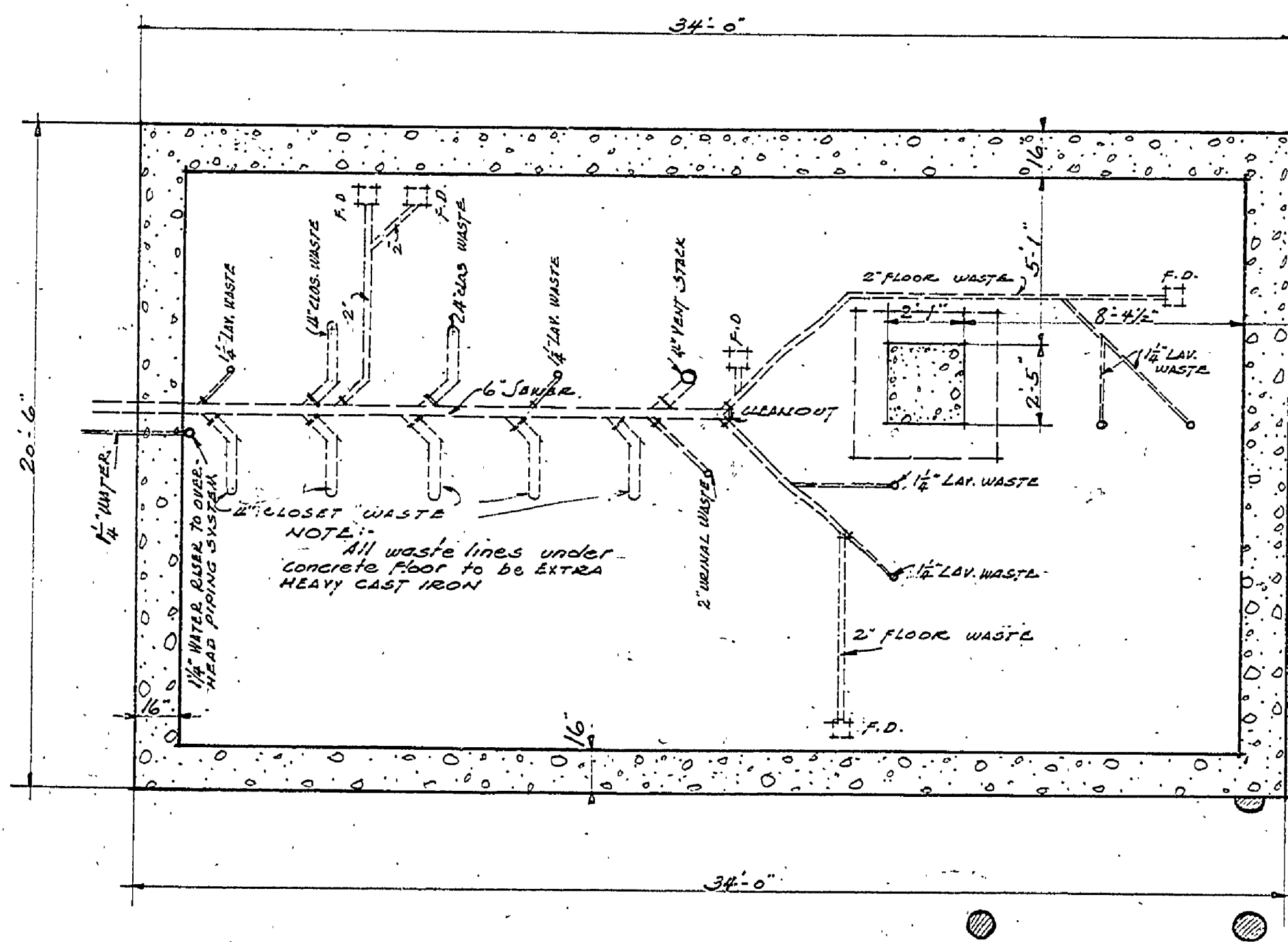
FOUNDATION & PIPING PLAN Scale: 1/4" = 1'-0"
