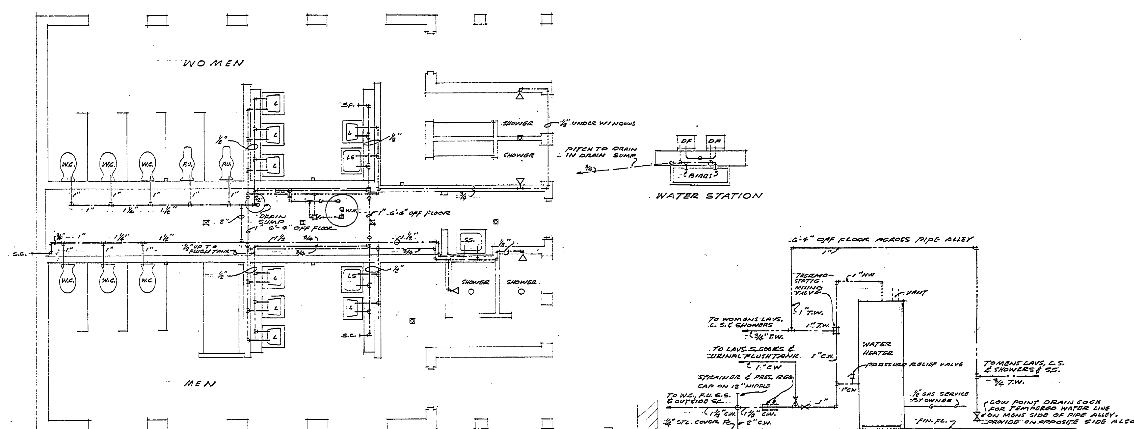
PLUMBING SUPPLY FLOOR PLAN SCALE 1/4" = 1'-0"
