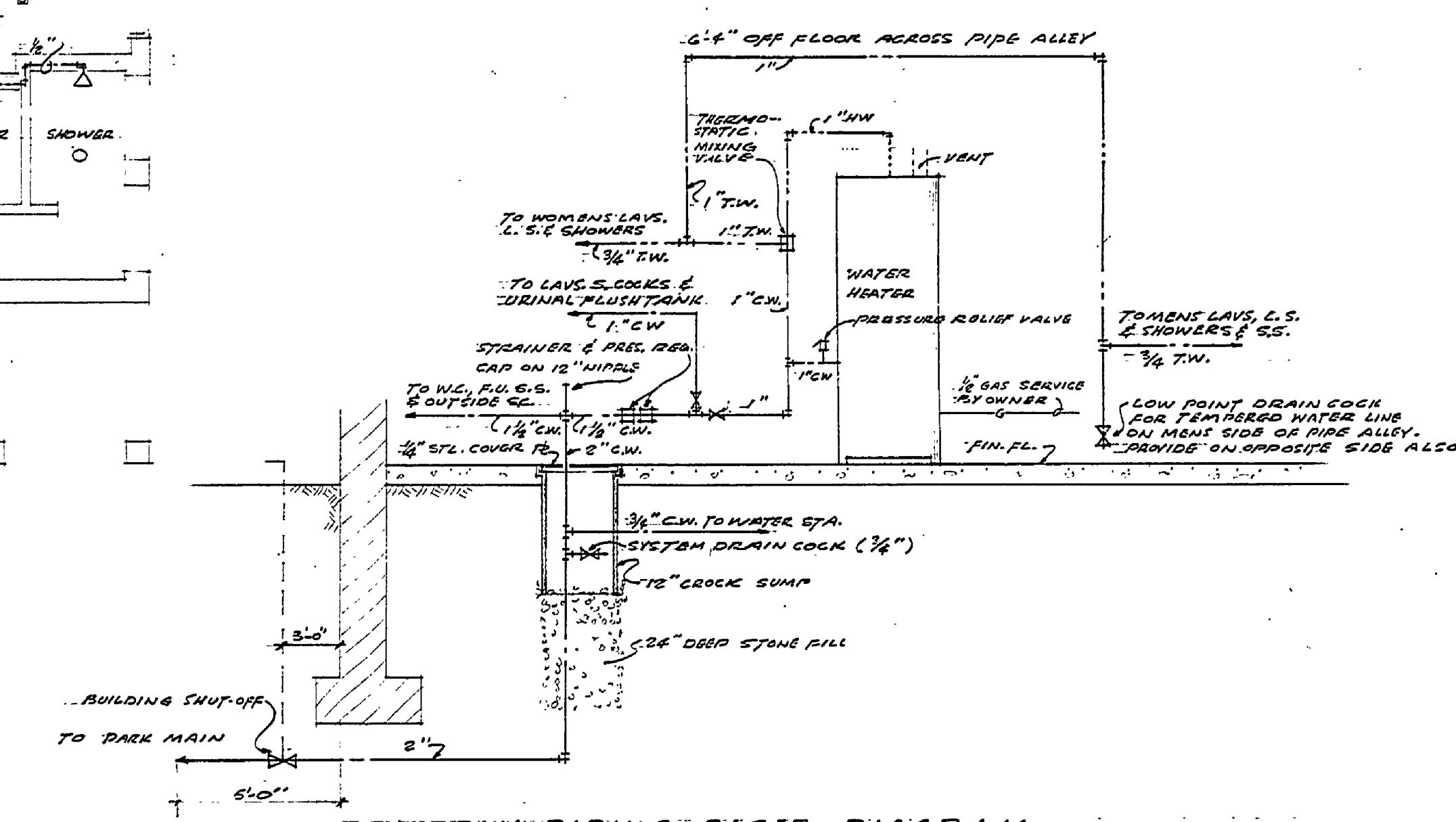
SUPPLY PIPING RISER DIAGRAM NO SCALE
