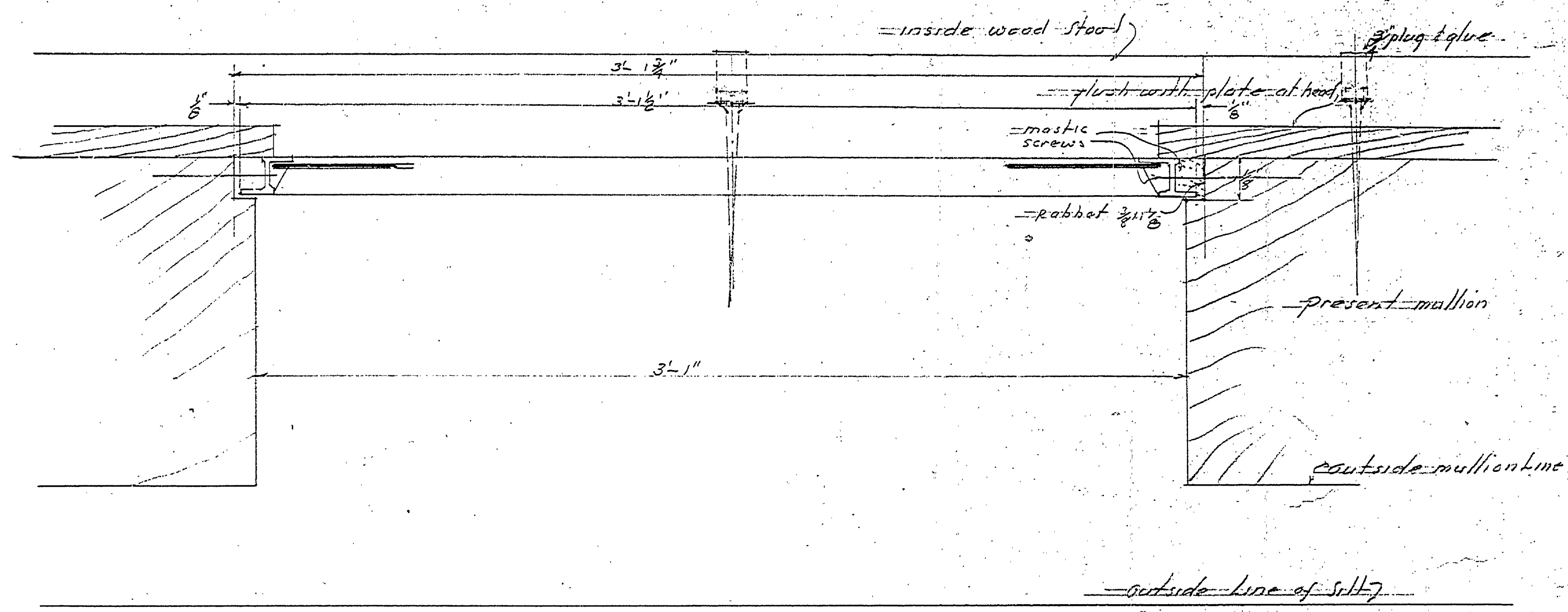
PLAN SECTION Scale 1/2" = 1'-0"
