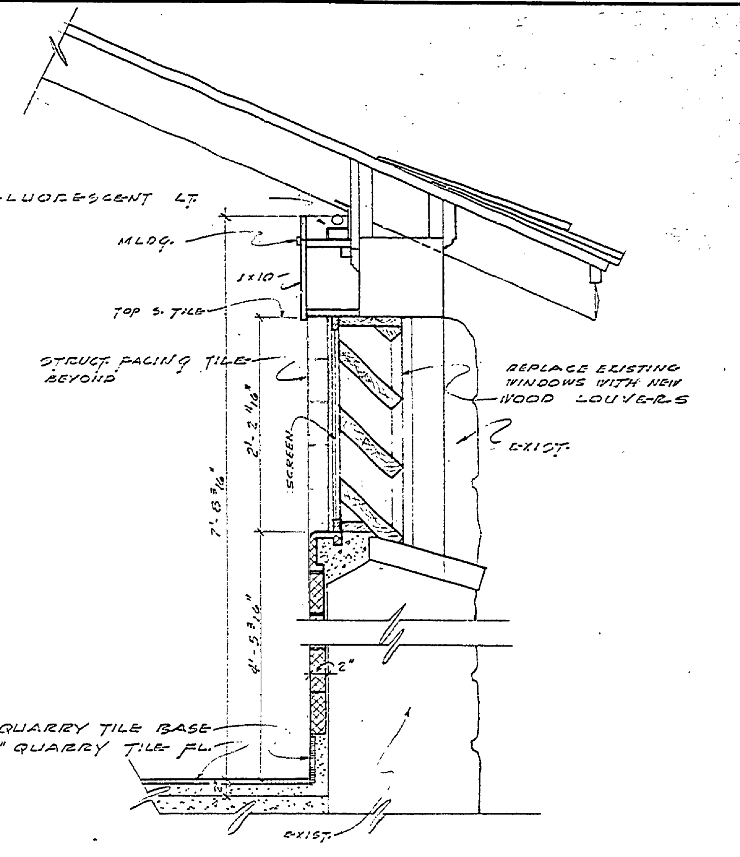
WALL SECTION - NORTH & SOUTH SIDES SCALE - 1" = 1'-0"
