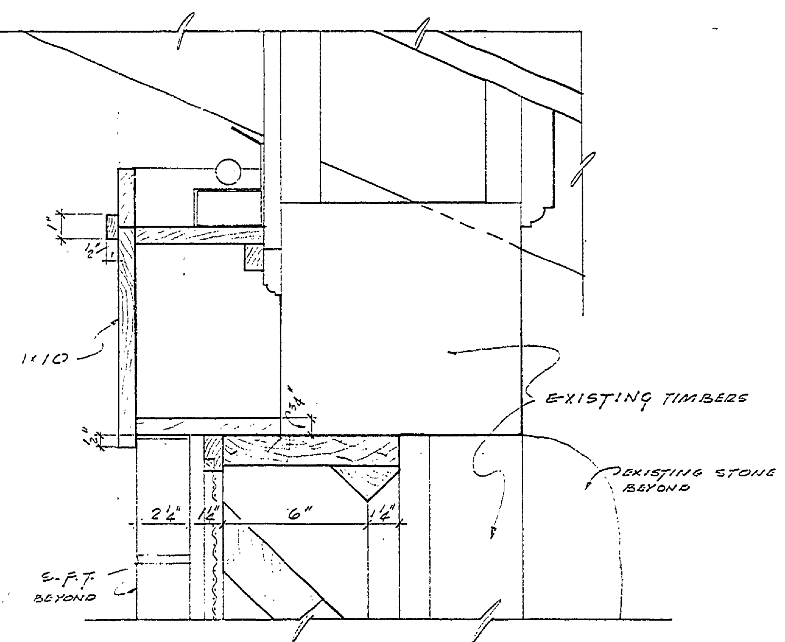
HEAD DETAIL SCALE - 3" = 1'-0"
