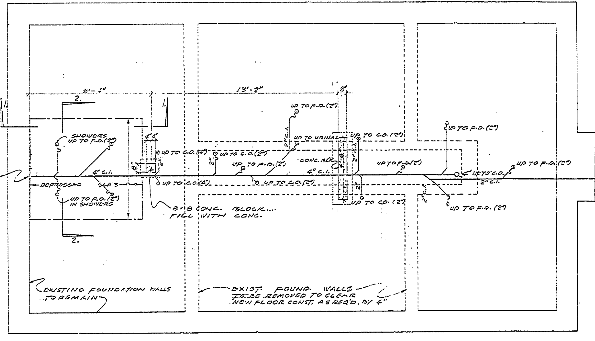
FOUNDATION & U.G. PLUMBING PLAN
