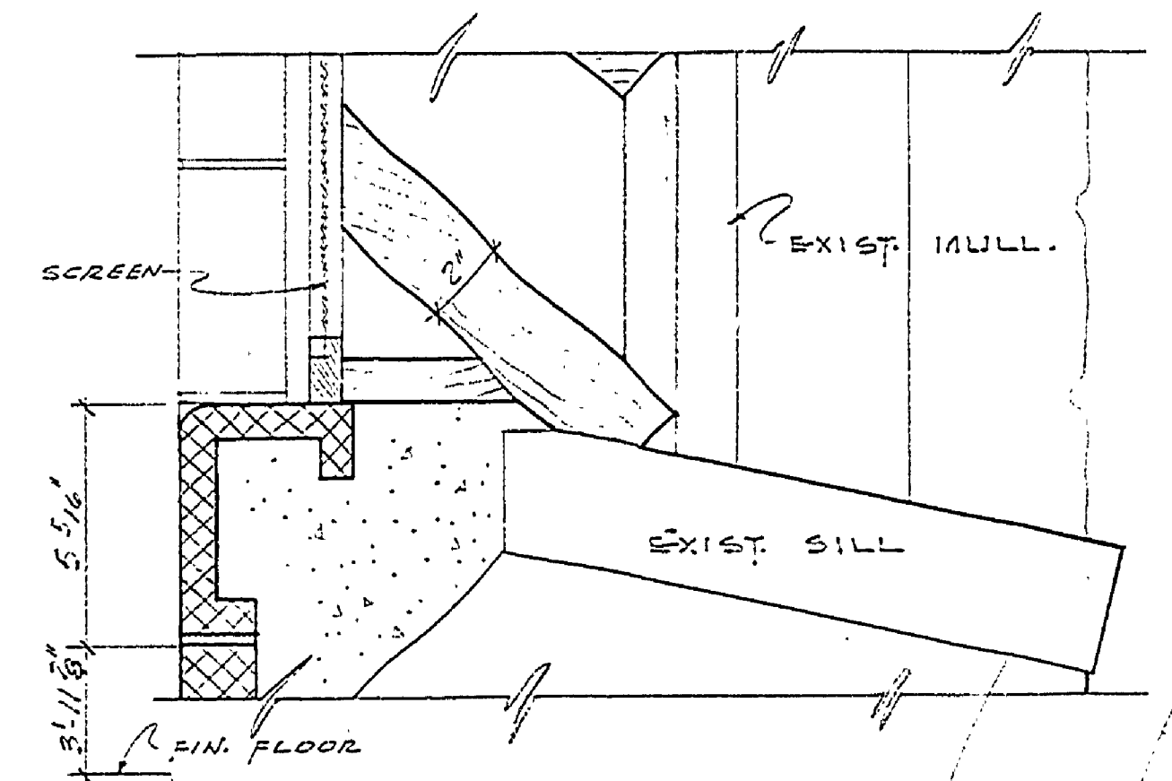
SILL DETAIL SCALE - 3" = 1'-0"
