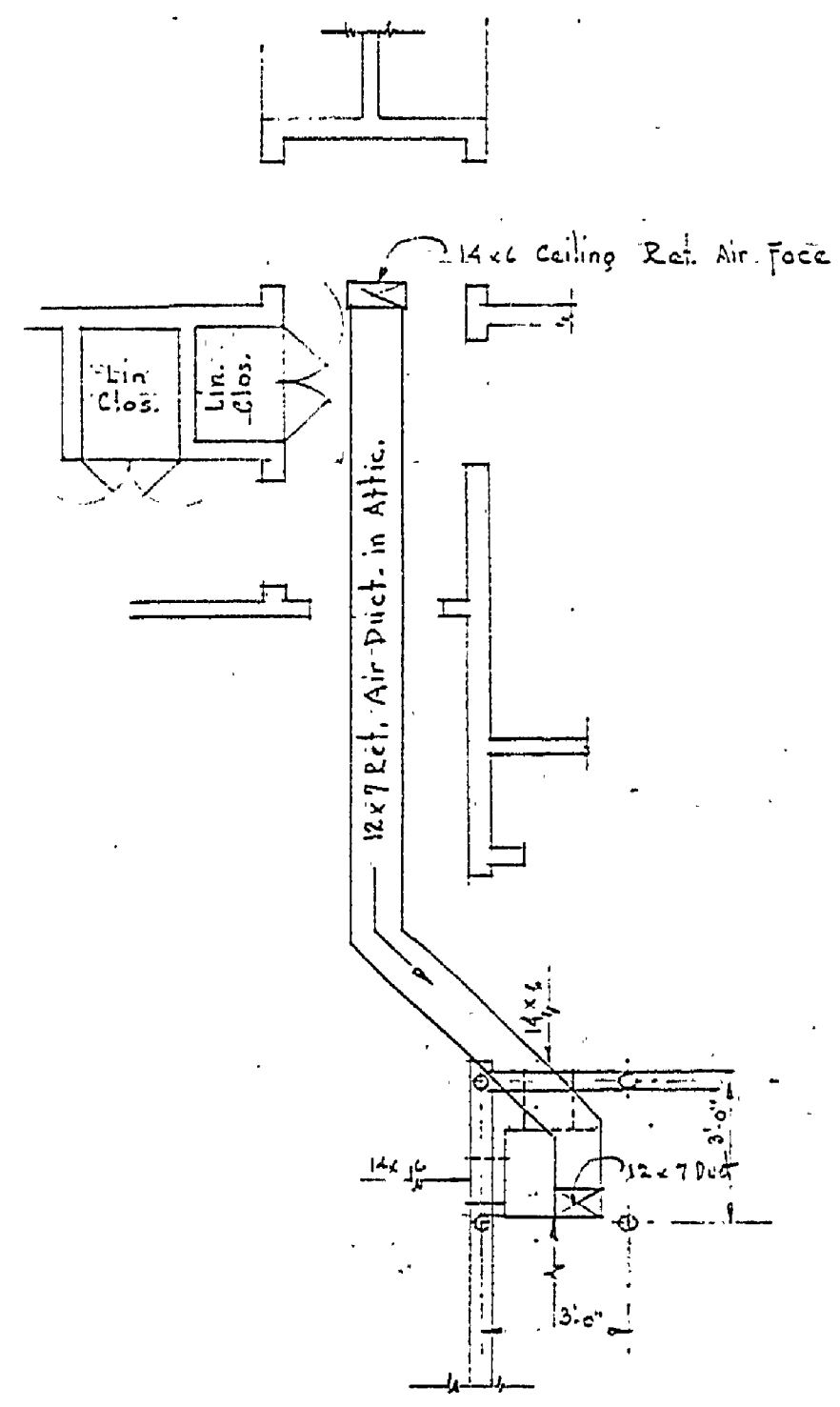
PLAN LAYOUT OF RETURN DUCT Scale 1/4" = 1'-0"
