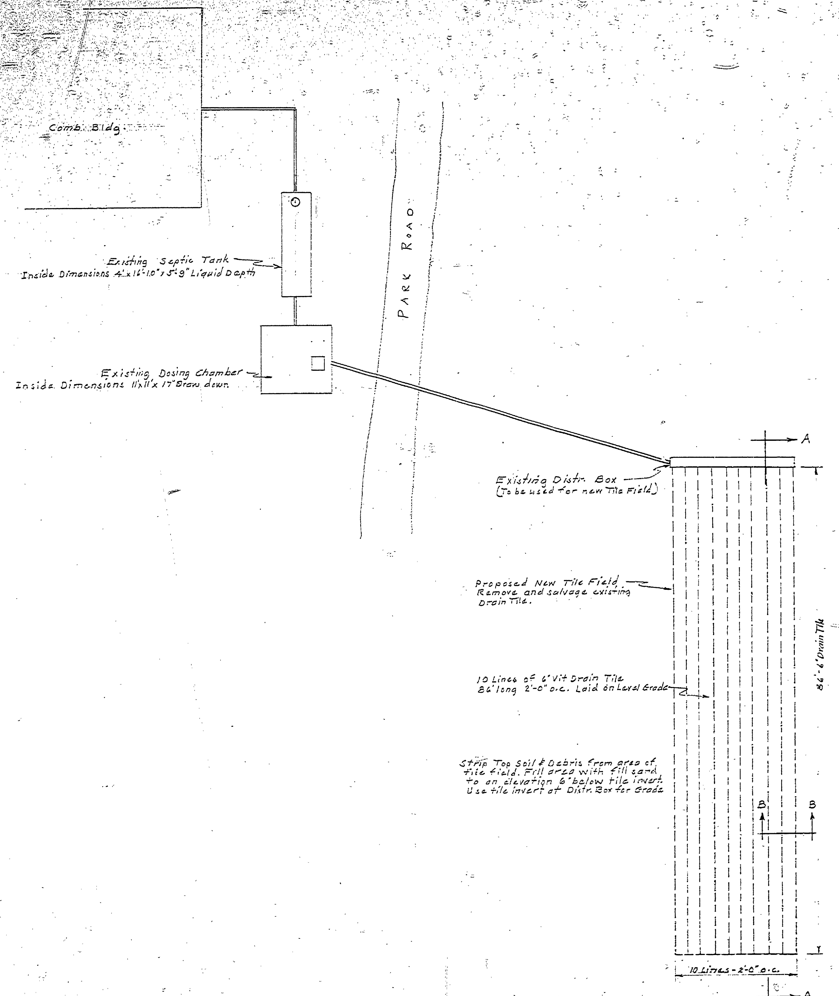
SEWAGE SYSTEM PLAN SCALE 1"=10'-0"
