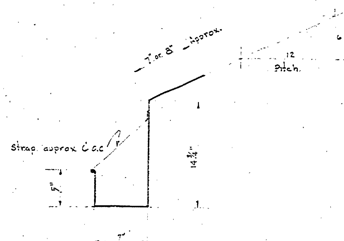
SECTION THRU HANGING GUTTER.
