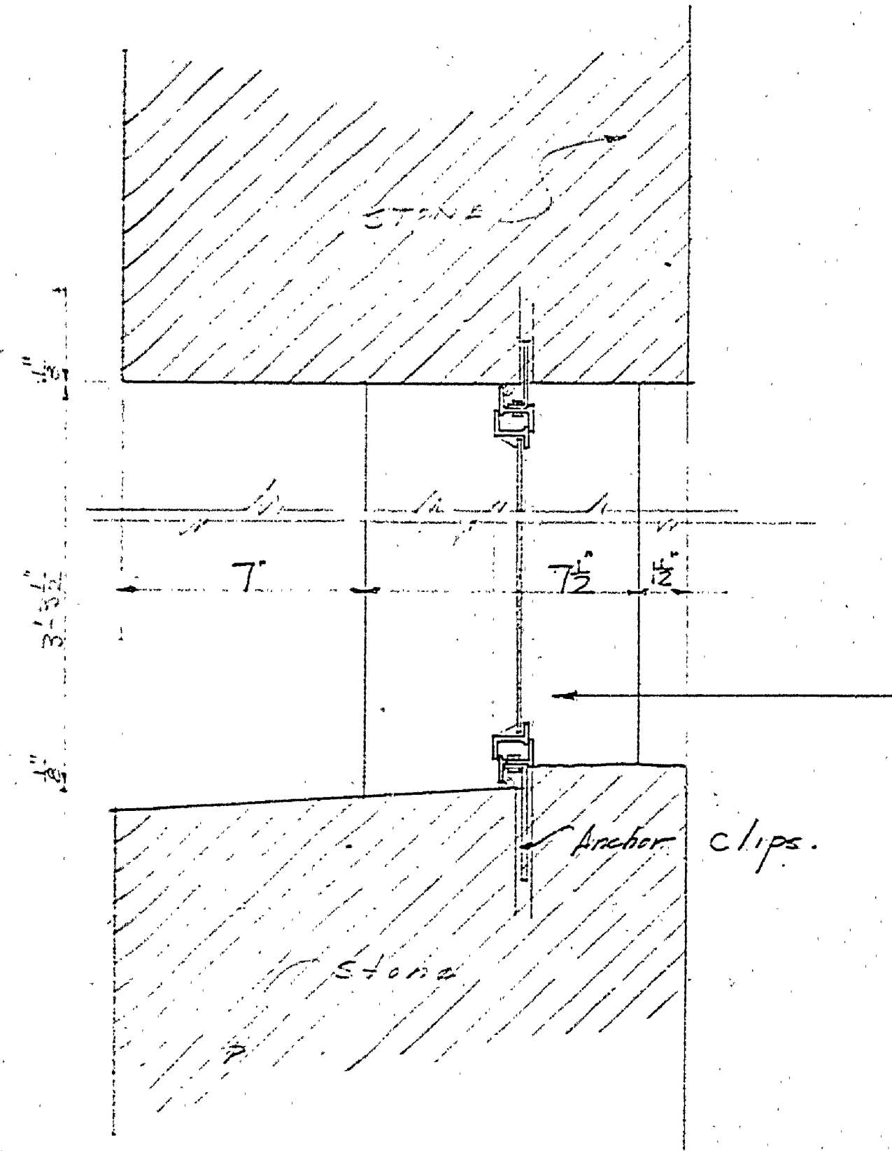
JAMB SECTION SCALE 3" = 1'-0"
