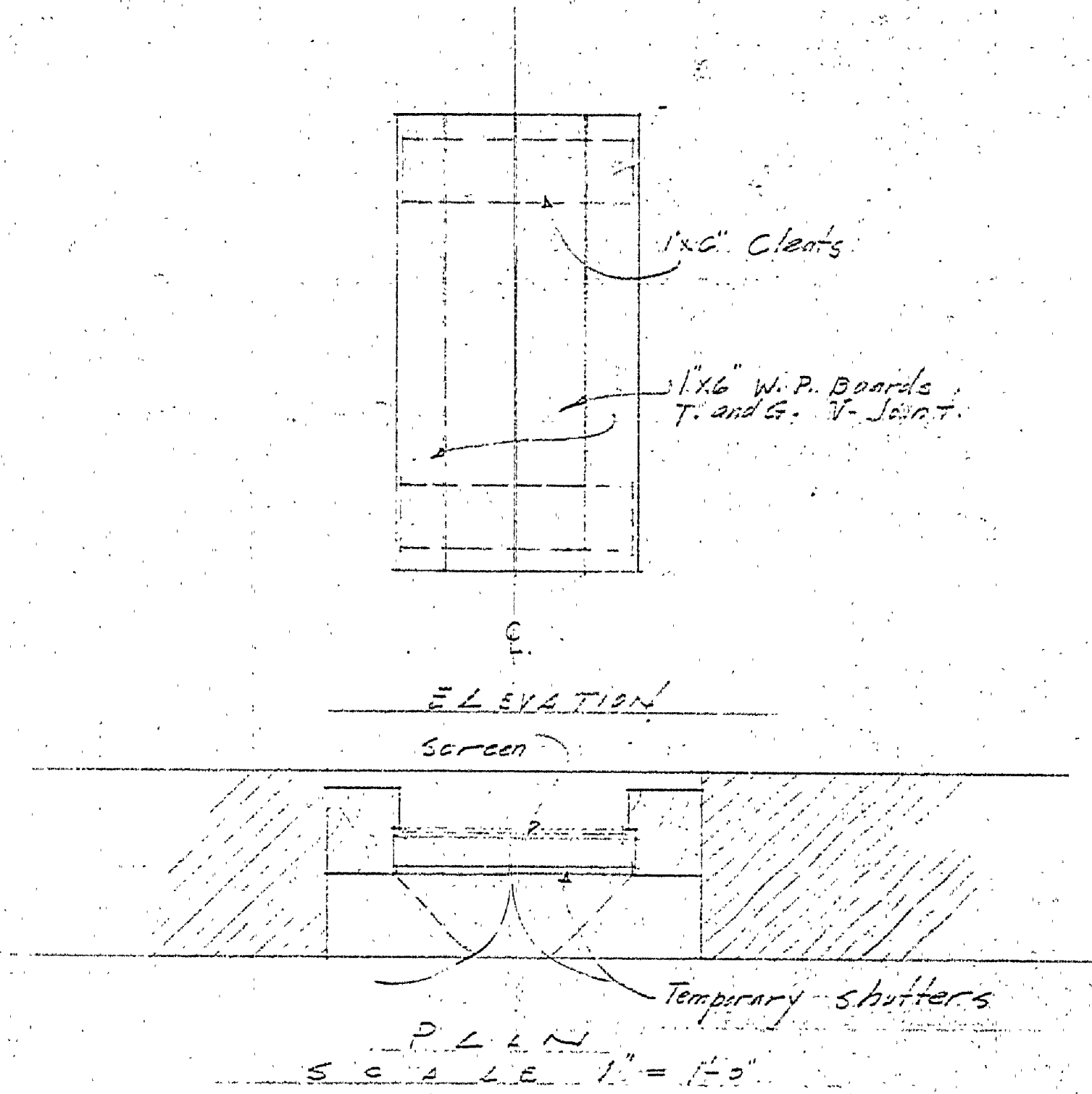
TEMPORARY ENCLOSURE FOR WINDOW OPENING AT FOOT OF BASEMENT STAIRS
