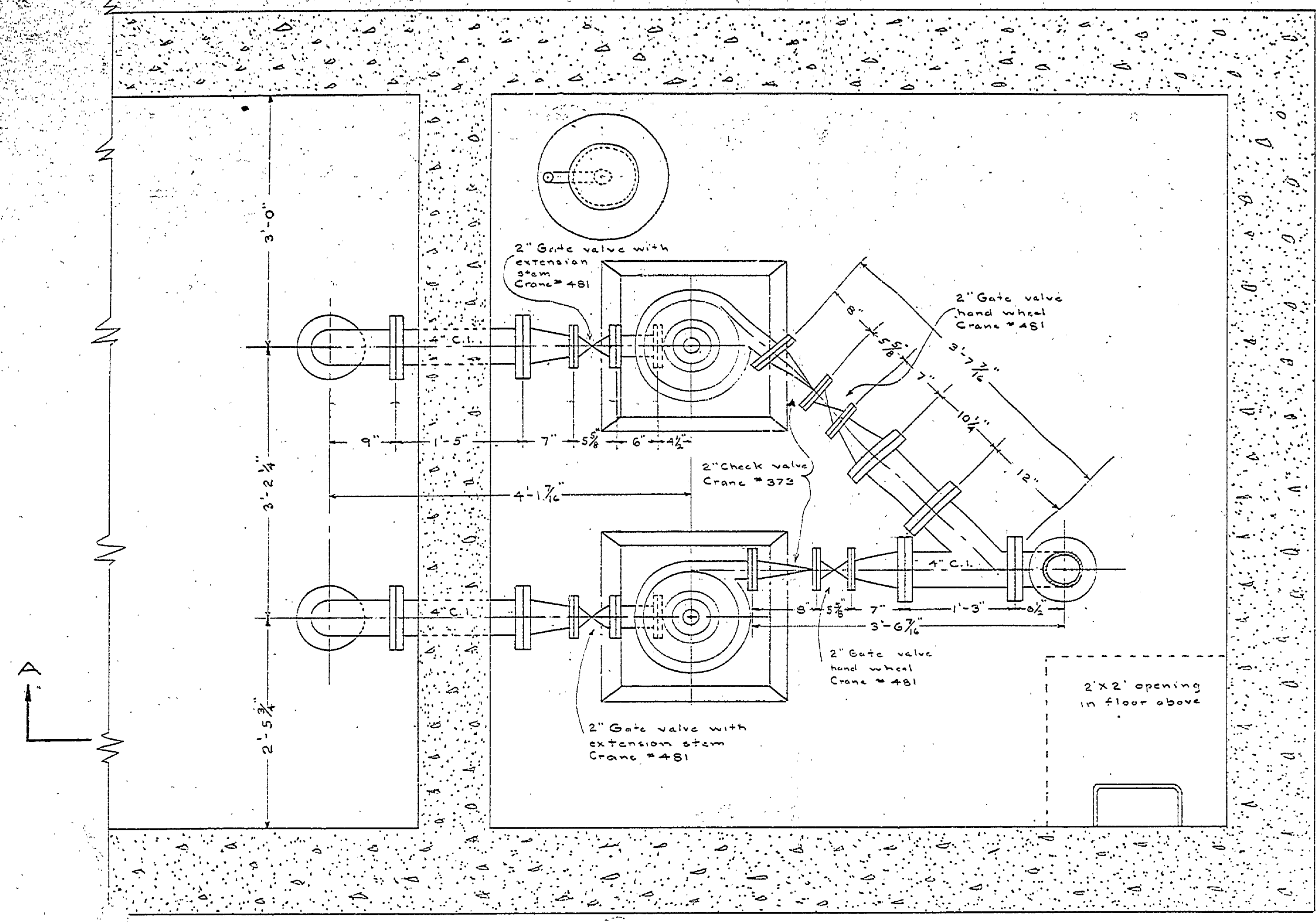
PLAN AT ELEV. 628.00 SCALE: 1"=1'-0"
